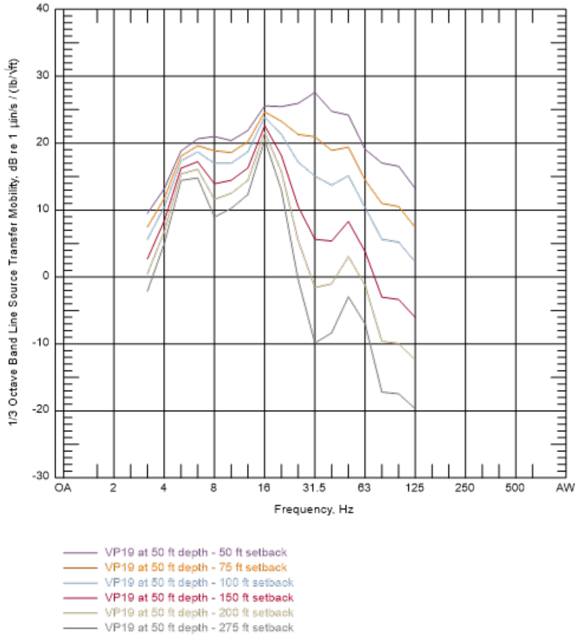
Figure C-1 Line Source Response for Borehole Impact Site VP19 – 50 ft Depth
