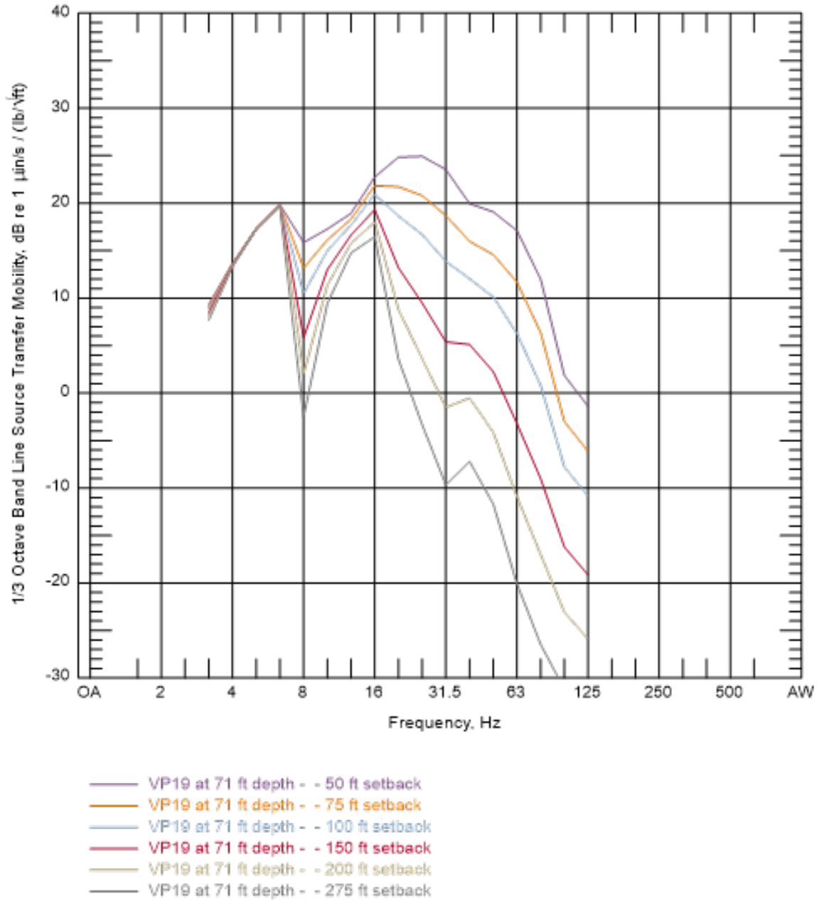
Figure C-3 Line Source Response for Borehole Impact Site VP19 – 71 ft Depth
