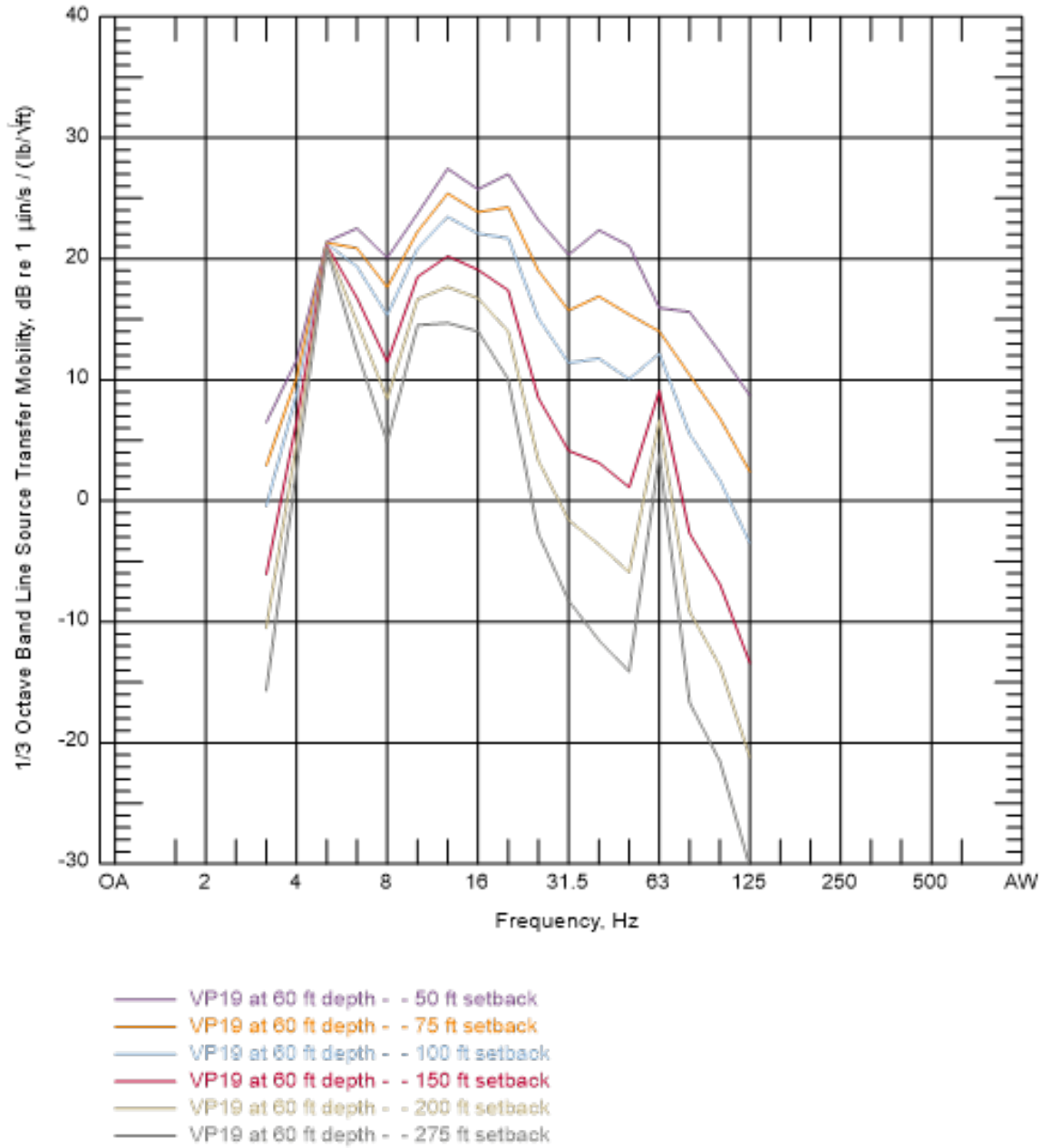
Figure C-2 Line Source Response for Borehole Impact Site VP19 – 60 ft Depth
