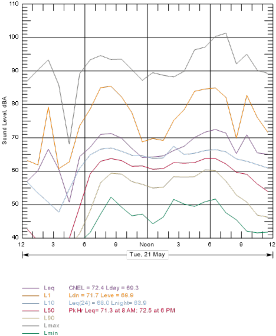
Figure B-168 Hourly Summary of Noise Levels Measured at N59 on May 21, 2013
