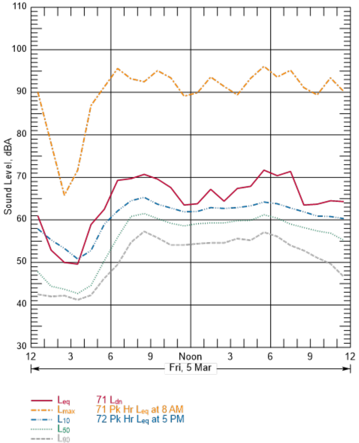
Figure B-161 Hourly Summary of Noise Levels Measured at N56 on March 5, 2010
