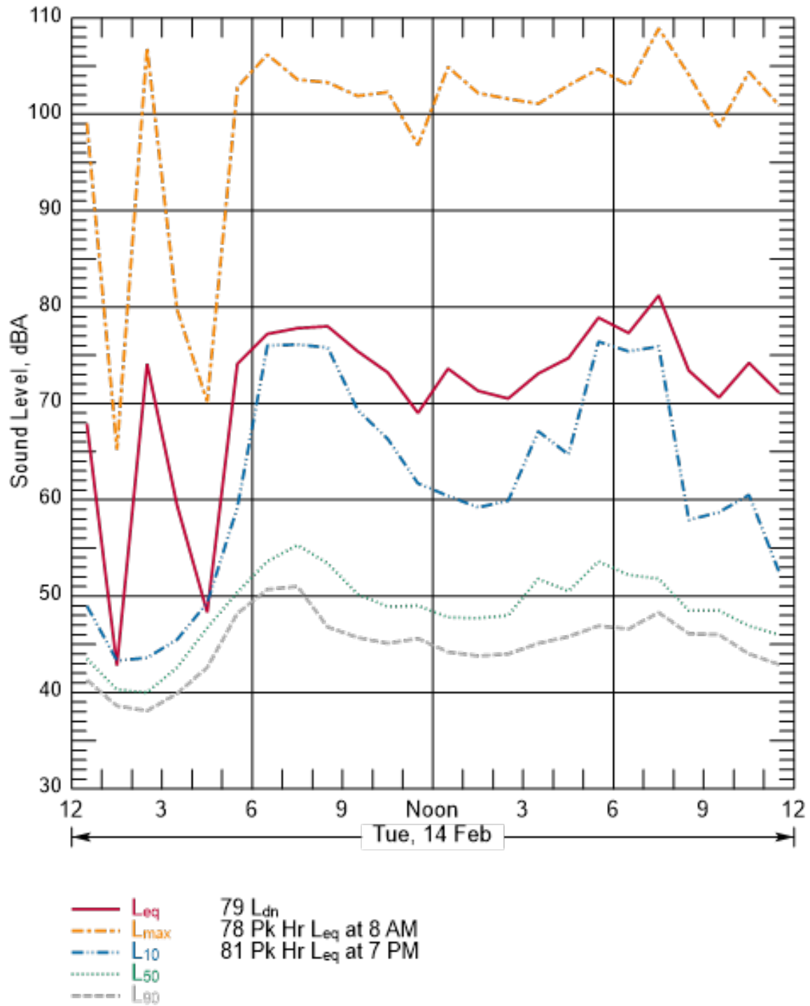
Figure B-98 Hourly Summary of Noise Levels Measured at N34 on February 14, 2017
