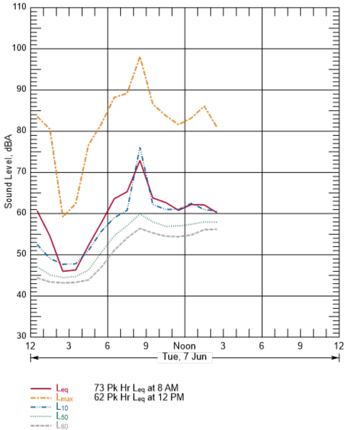
Figure B-174 Hourly Summary of Noise Levels Measured at N60 on June 7, 2016
