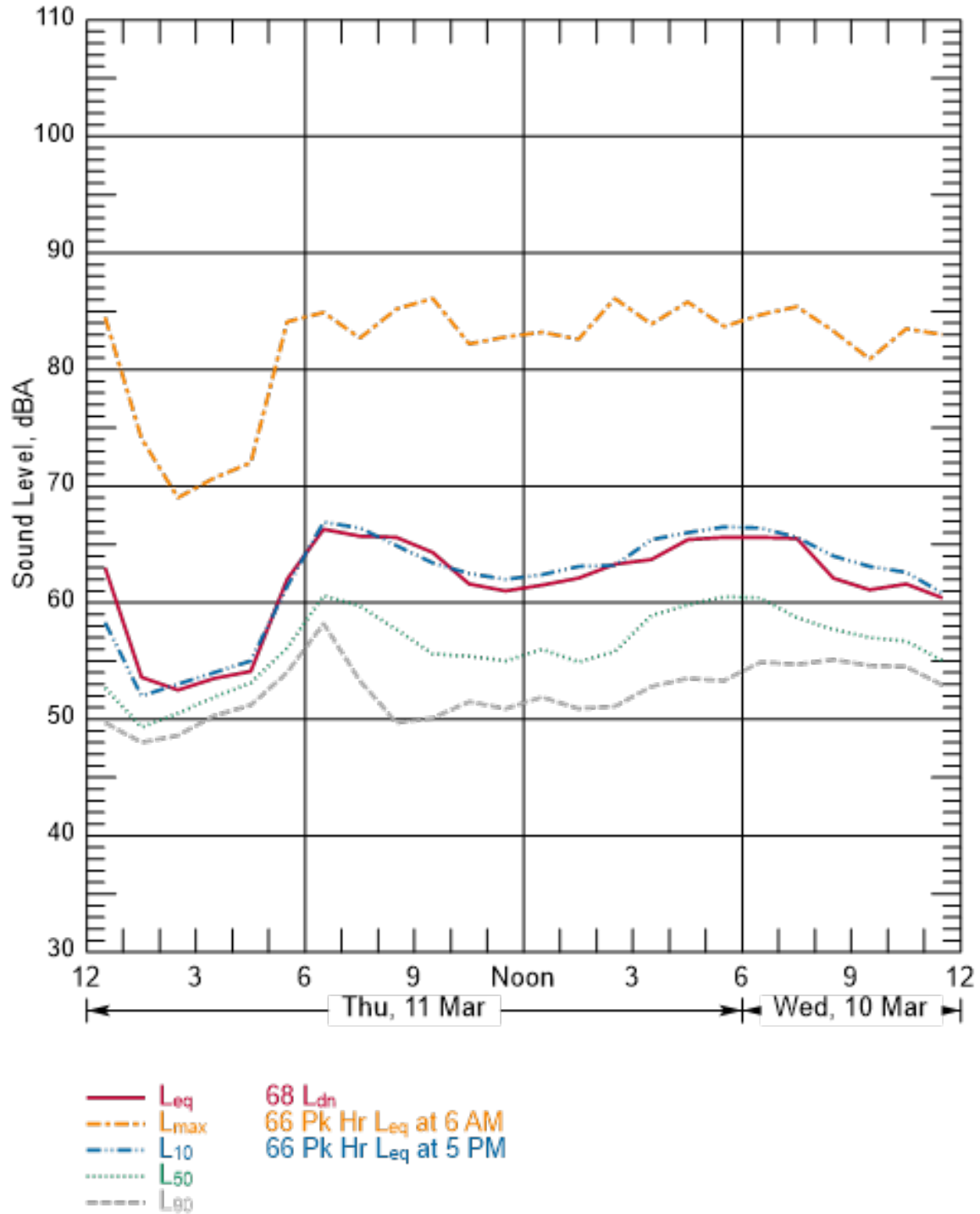
Figure B-80 Hourly Summary of Noise Levels Measured at N28 on March 10 and 11, 2010
