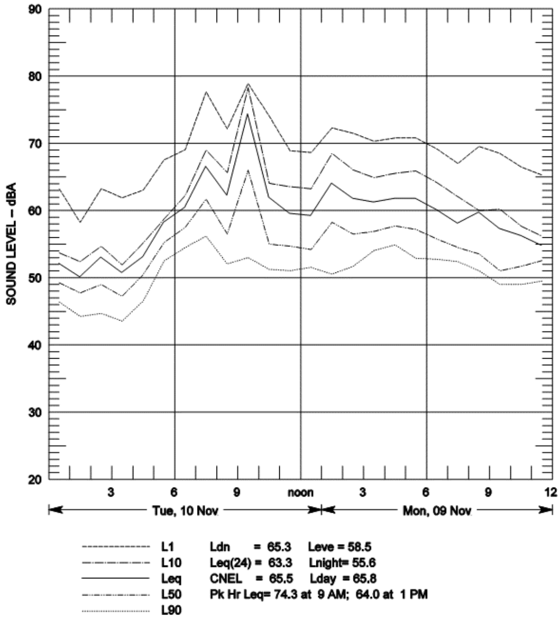
Figure B-10 Hourly Summary of Noise Levels Measured at N03 on November 9 and 10, 2009
