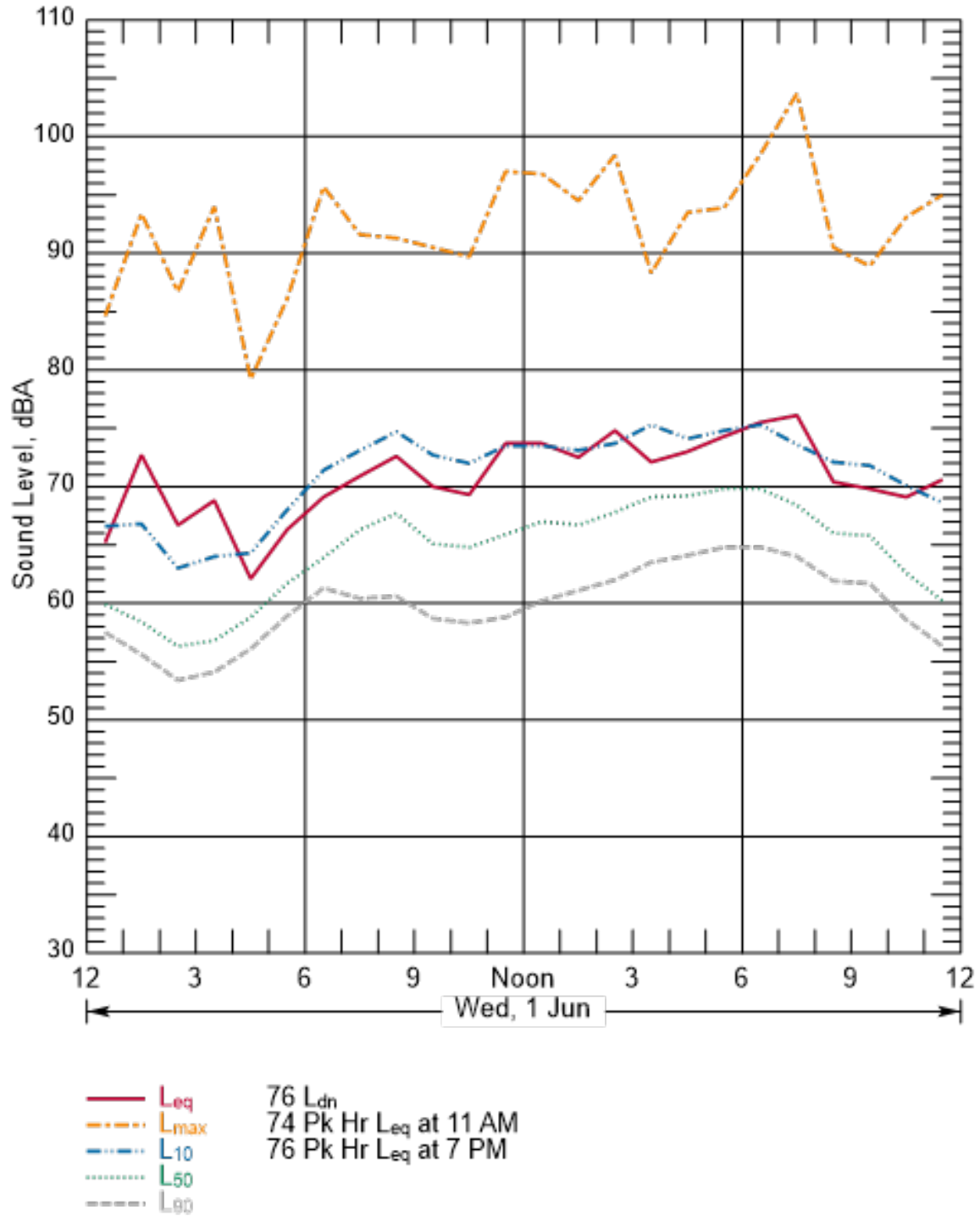
Figure B-58 Hourly Summary of Noise Levels Measured at N20 on June 1, 2016
