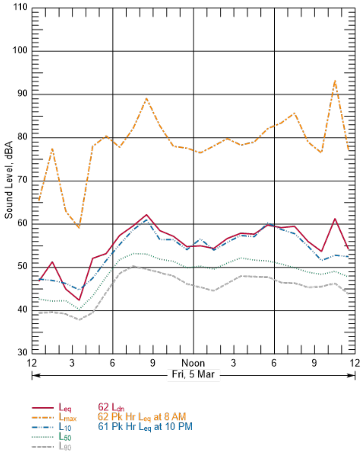
Figure B-178 Hourly Summary of Noise Levels Measured at N62 on March 5, 2010
