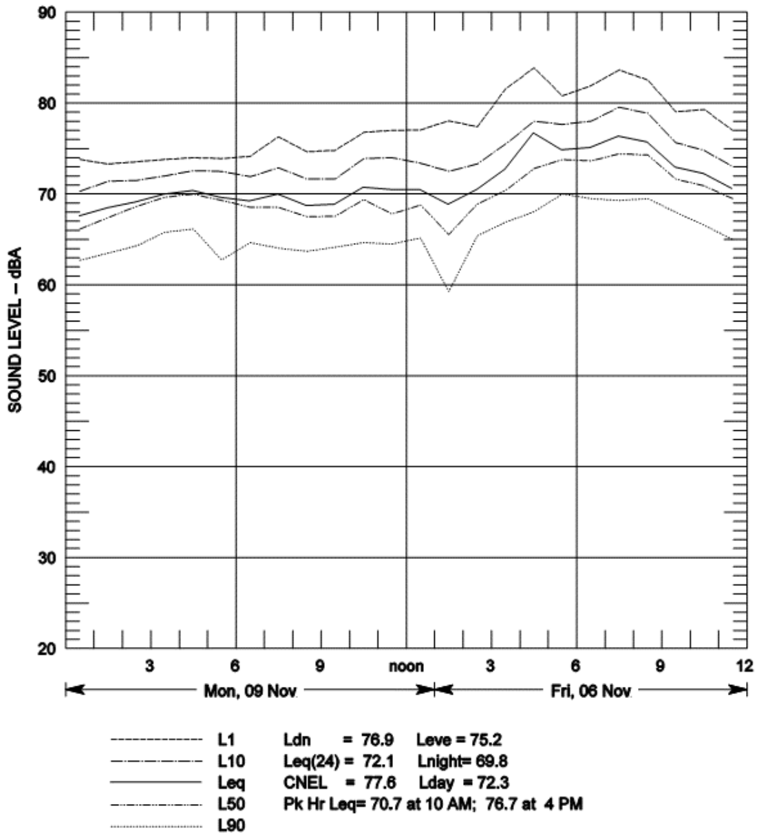
Figure B-20 Hourly Summary of Noise Levels Measured at N08 on November 6 and 9, 2009
