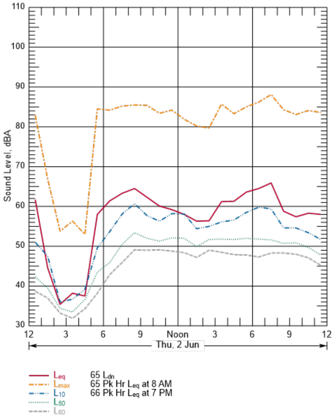
Figure B-109 Hourly Summary of Noise Levels Measured at N37 on June 2, 2016
