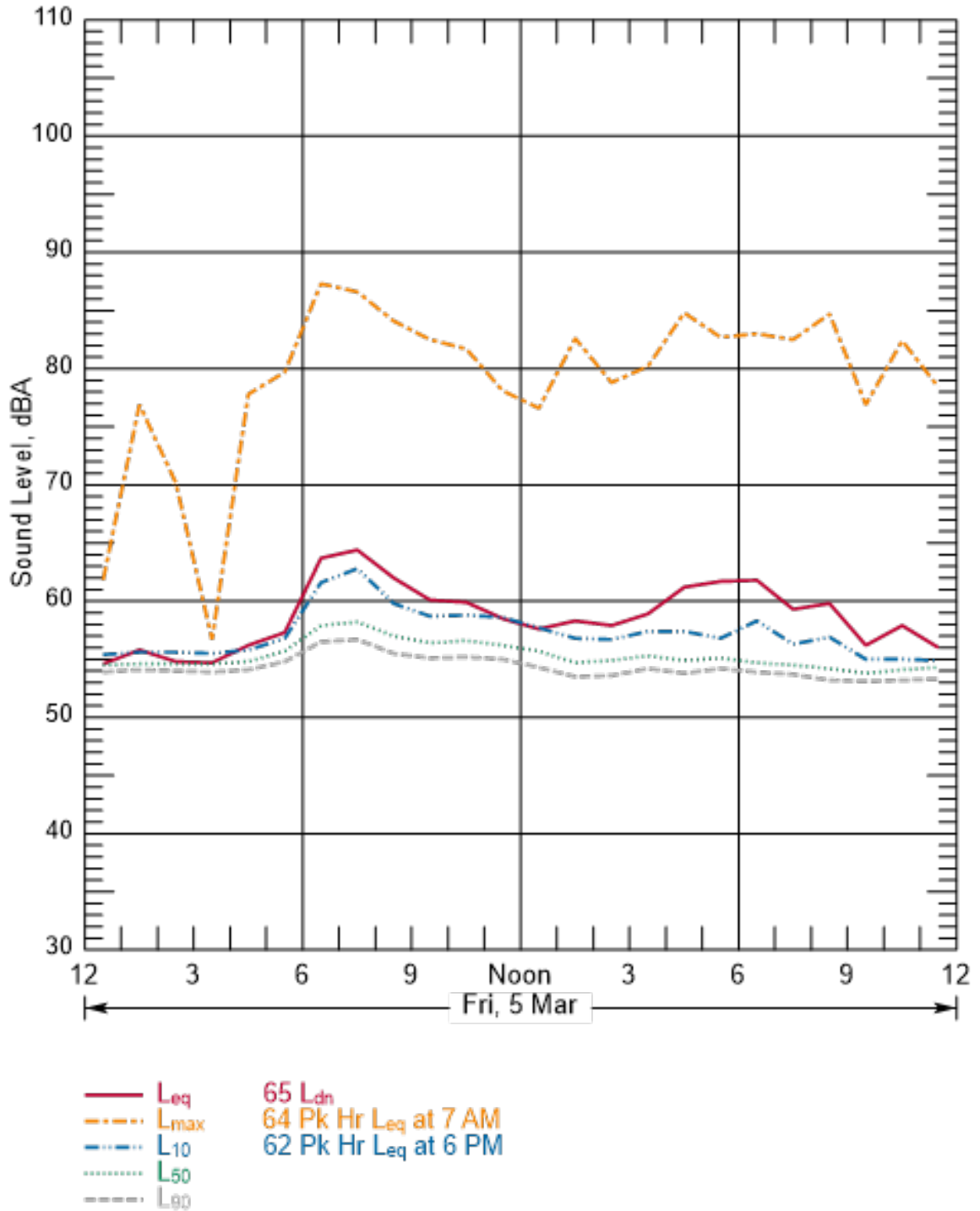
Figure B-213 Hourly Summary of Noise Levels Measured at N75 on March 5, 2010
