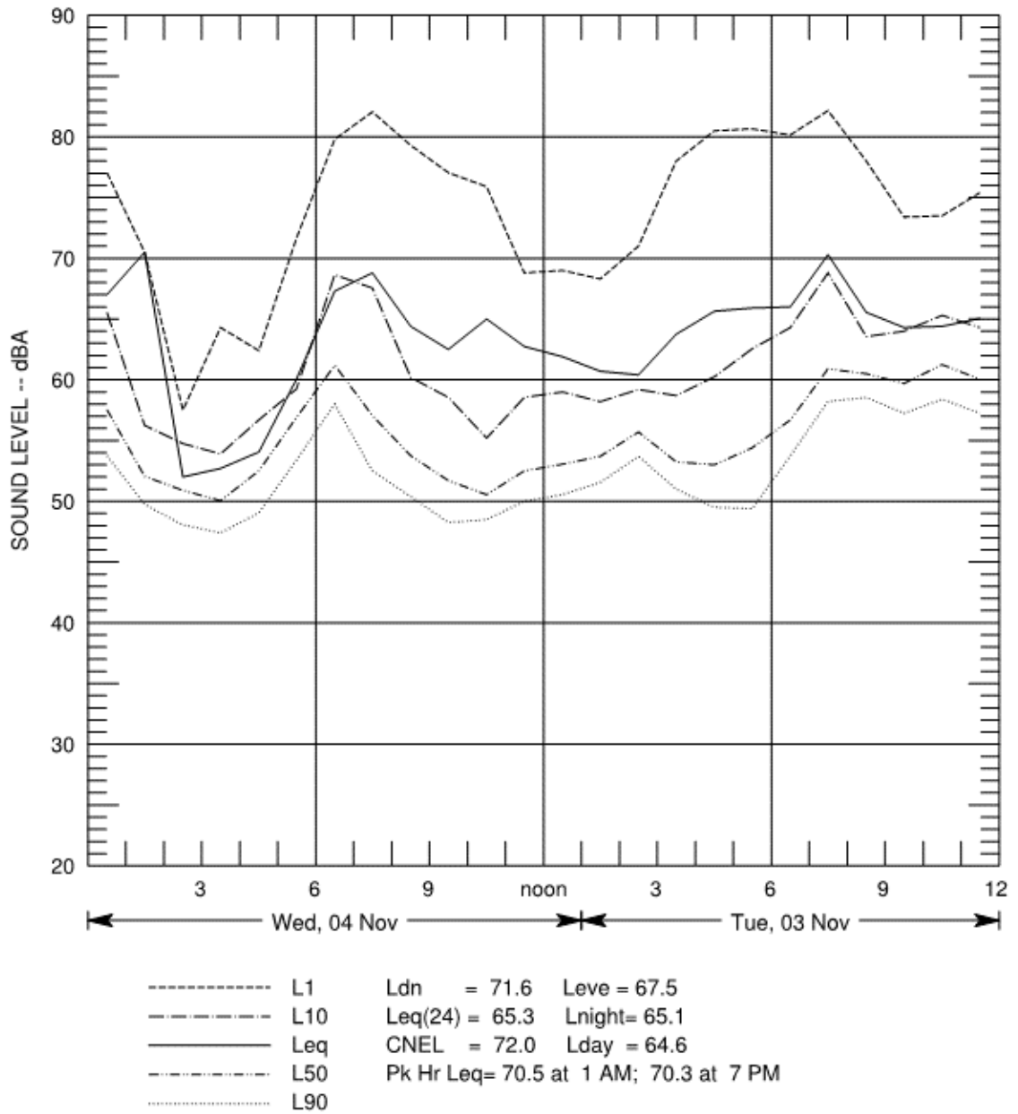
Figure B-67 Hourly Summary of Noise Levels Measured at N24 on November 3 and 4, 2010
