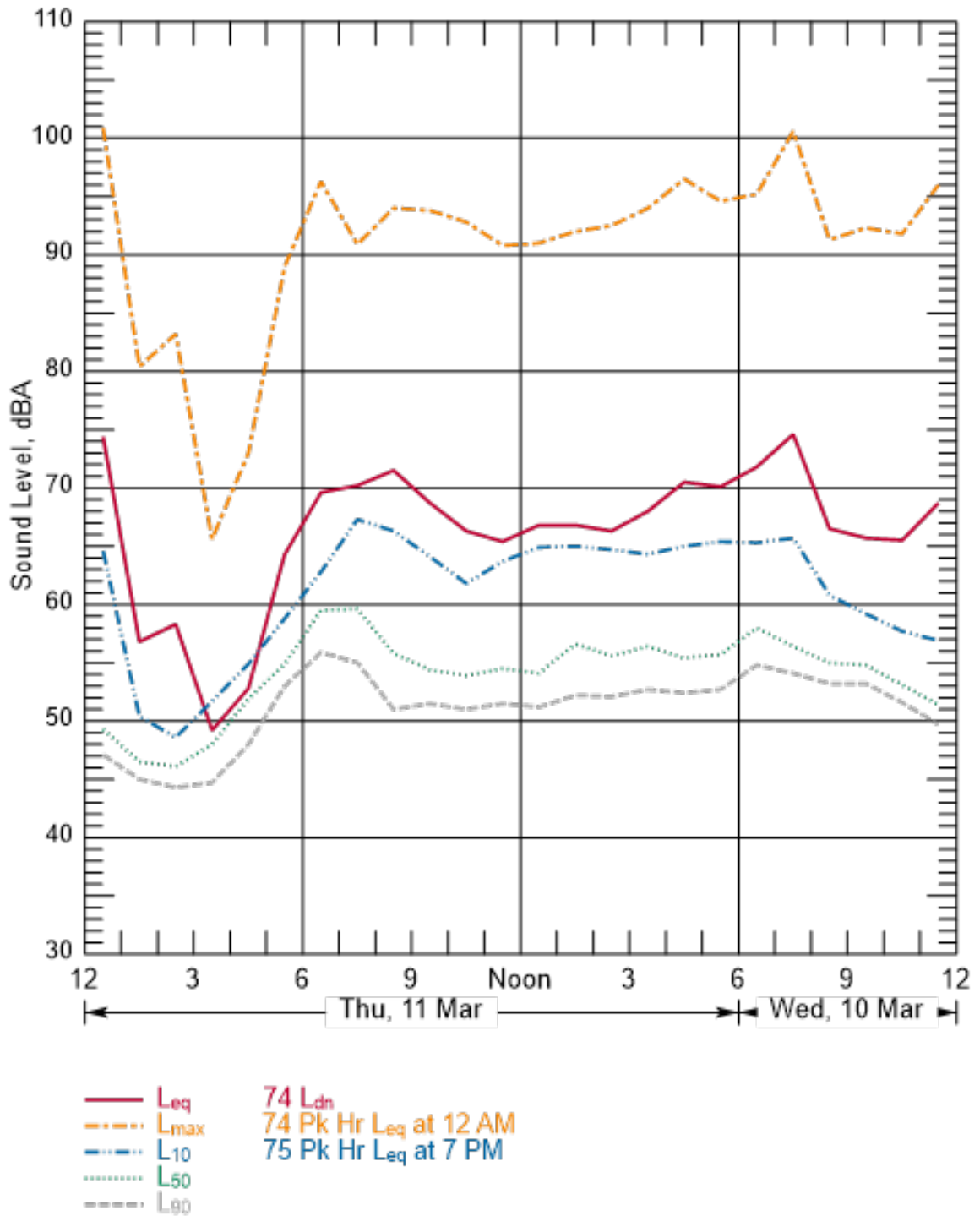
Figure B-61 Hourly Summary of Noise Levels Measured at N21 on March 10 and 11, 2010
