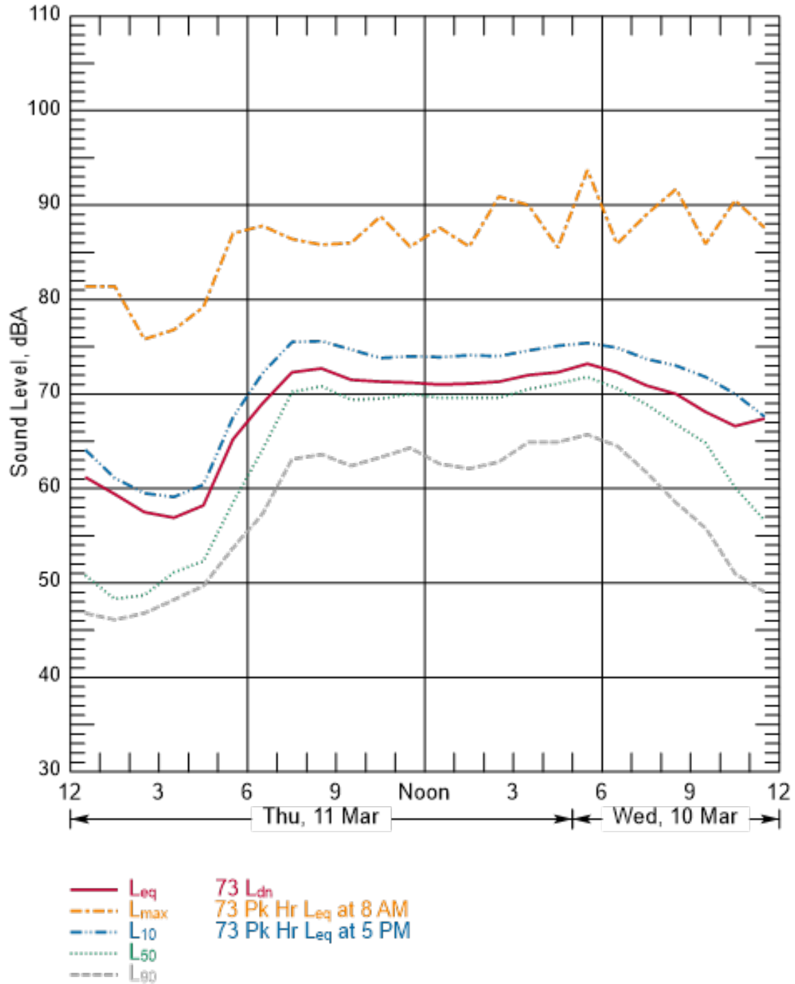
Figure B-130 Hourly Summary of Noise Levels Measured at N44 on March 10 and 11, 2010
