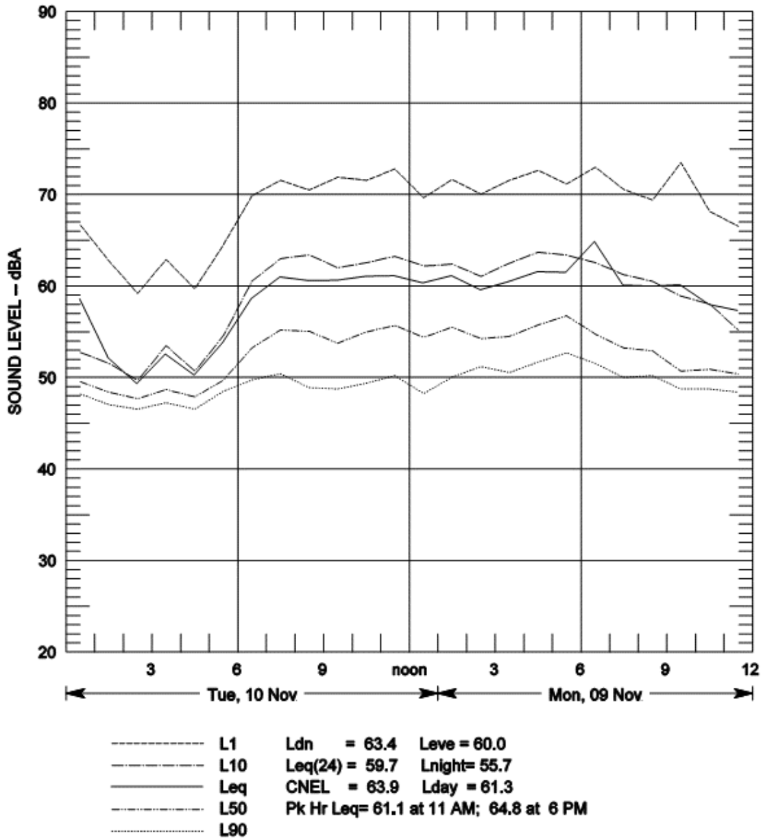
Figure B-14 Hourly Summary of Noise Levels Measured at N05 on November 9 and 10, 2009
