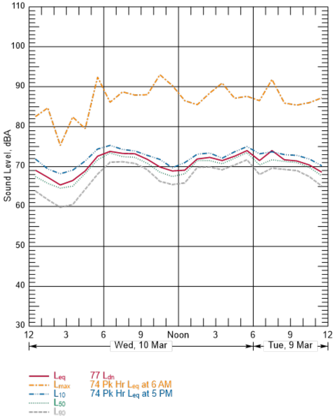
Figure B-43 Hourly Summary of Noise Levels Measured at N15 on March 9 and 10, 2010
