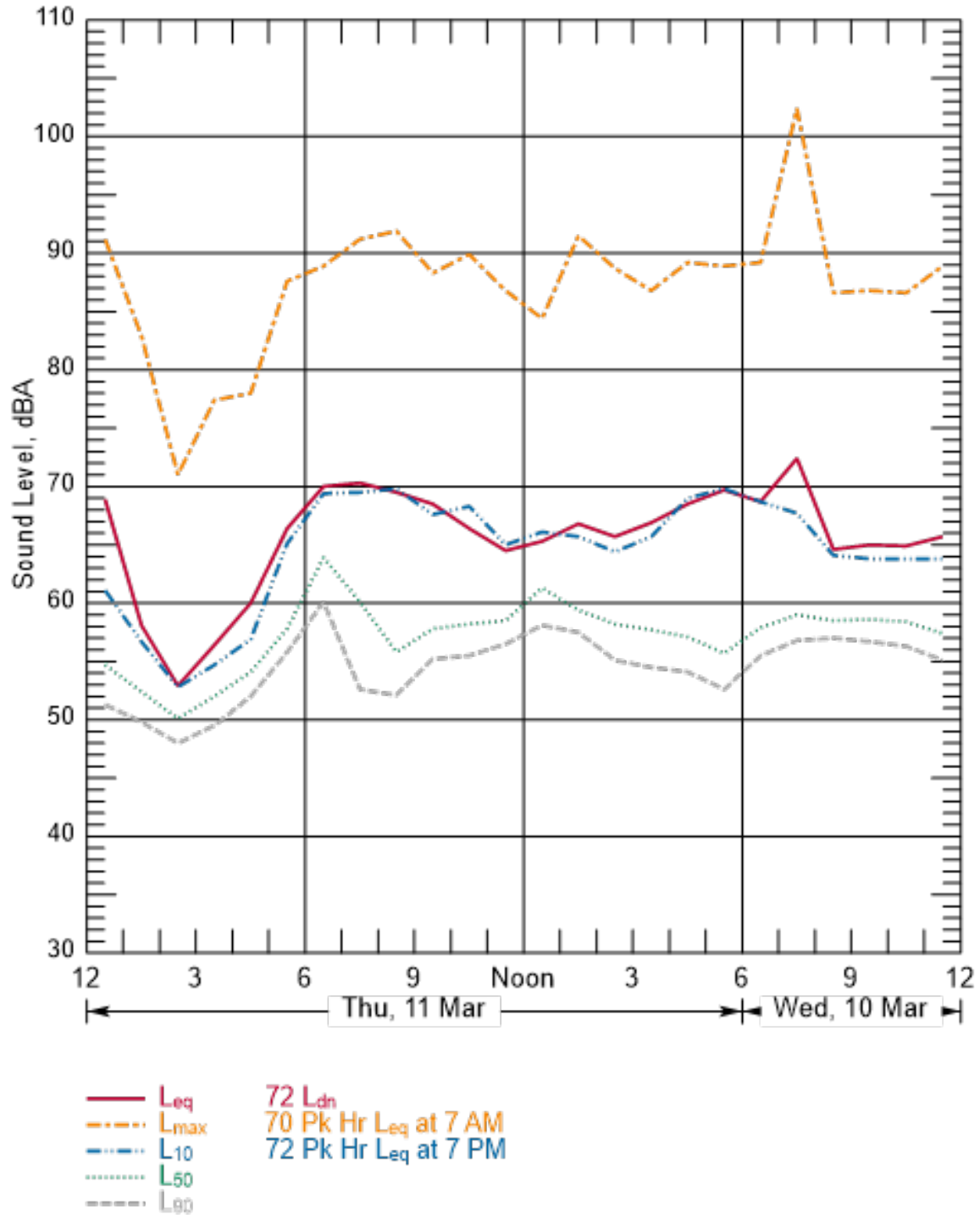
Figure B-78 Hourly Summary of Noise Levels Measured at N27 on March 10 and 11, 2010
