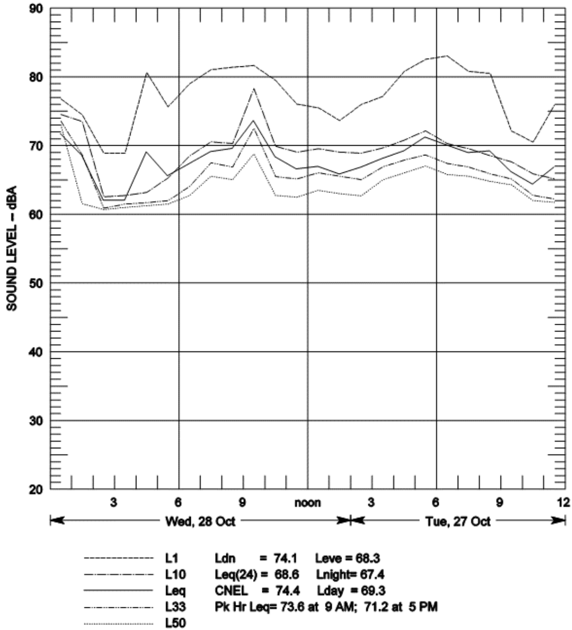
Figure B-116 Hourly Summary of Noise Levels Measured at N40 on October 27 and 28, 2009
