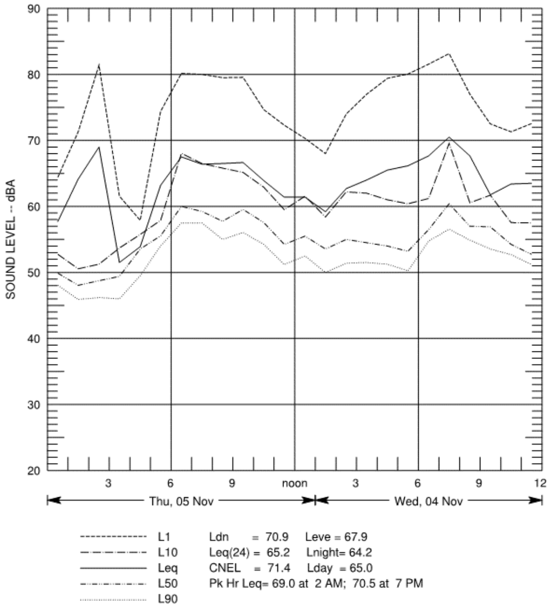
Figure B-68 Hourly Summary of Noise Levels Measured at N24 on November 4 and 5, 2010
