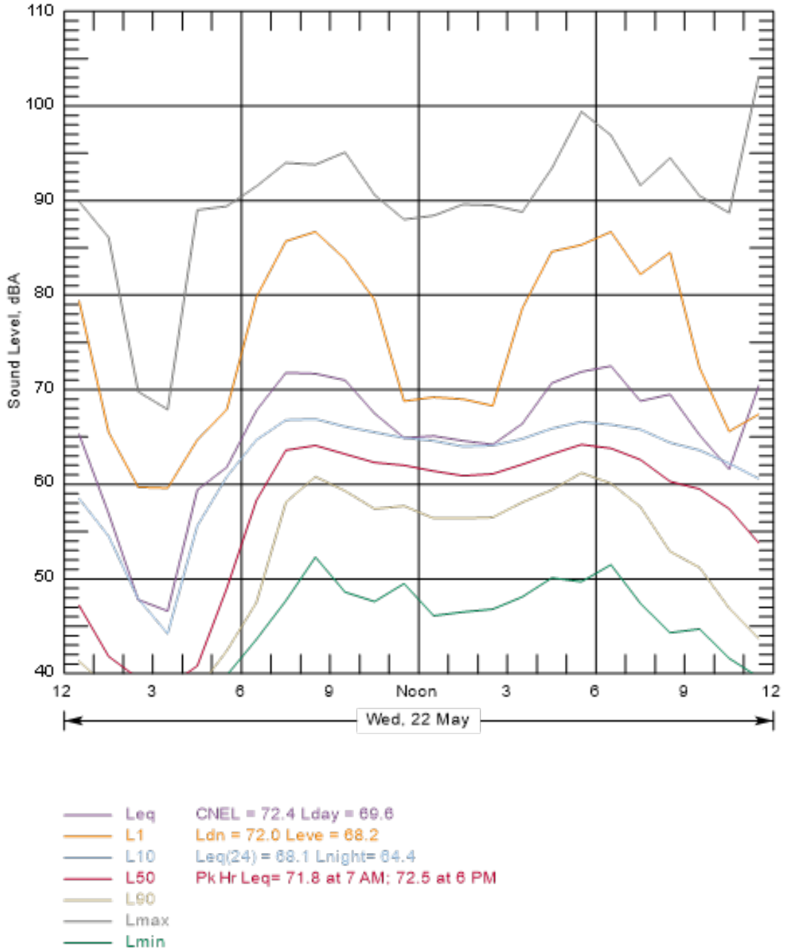
Figure B-169 Hourly Summary of Noise Levels Measured at N59 on May 22, 2013
