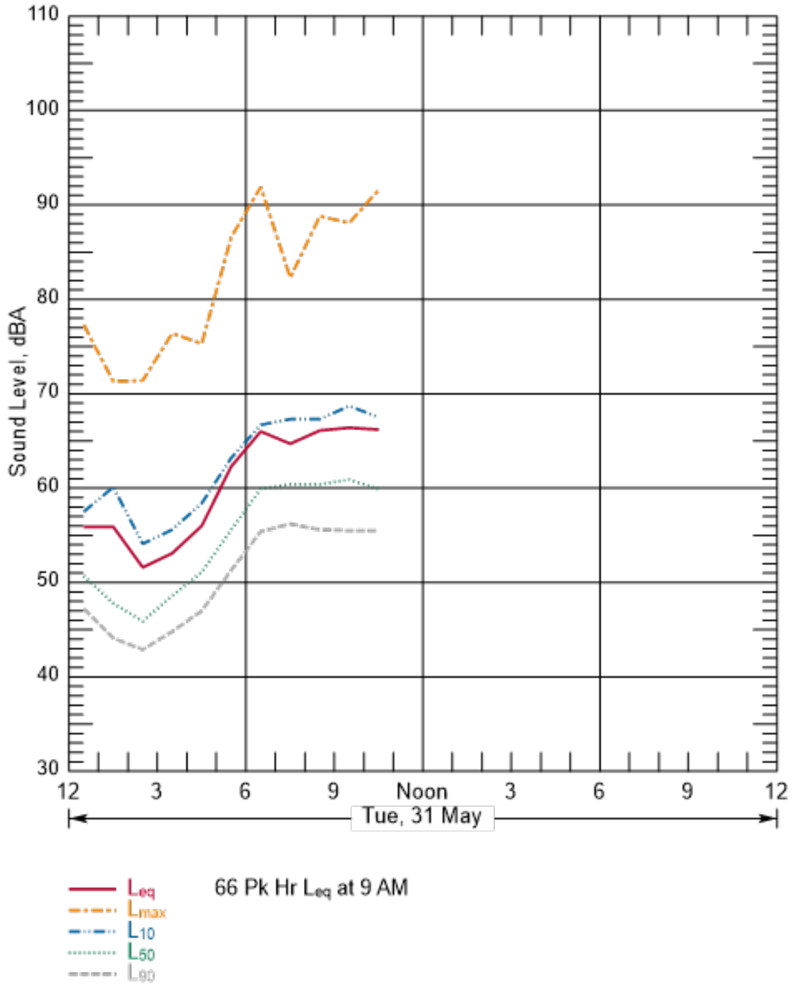
Figure B-29 Hourly Summary of Noise Levels Measured at N10 on May 31, 2016
