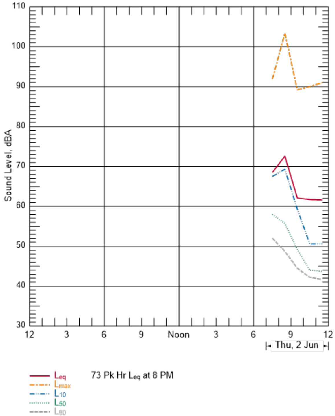
Figure B-144 Hourly Summary of Noise Levels Measured at N49 on June 2, 2016
