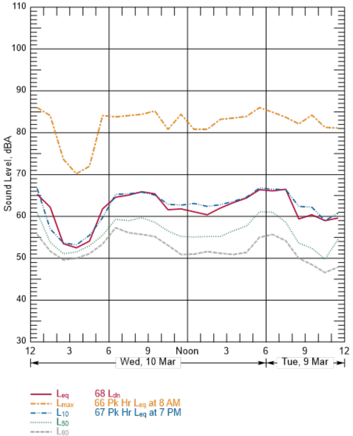
Figure B-79 Hourly Summary of Noise Levels Measured at N28 on March 9 and 10, 2010
