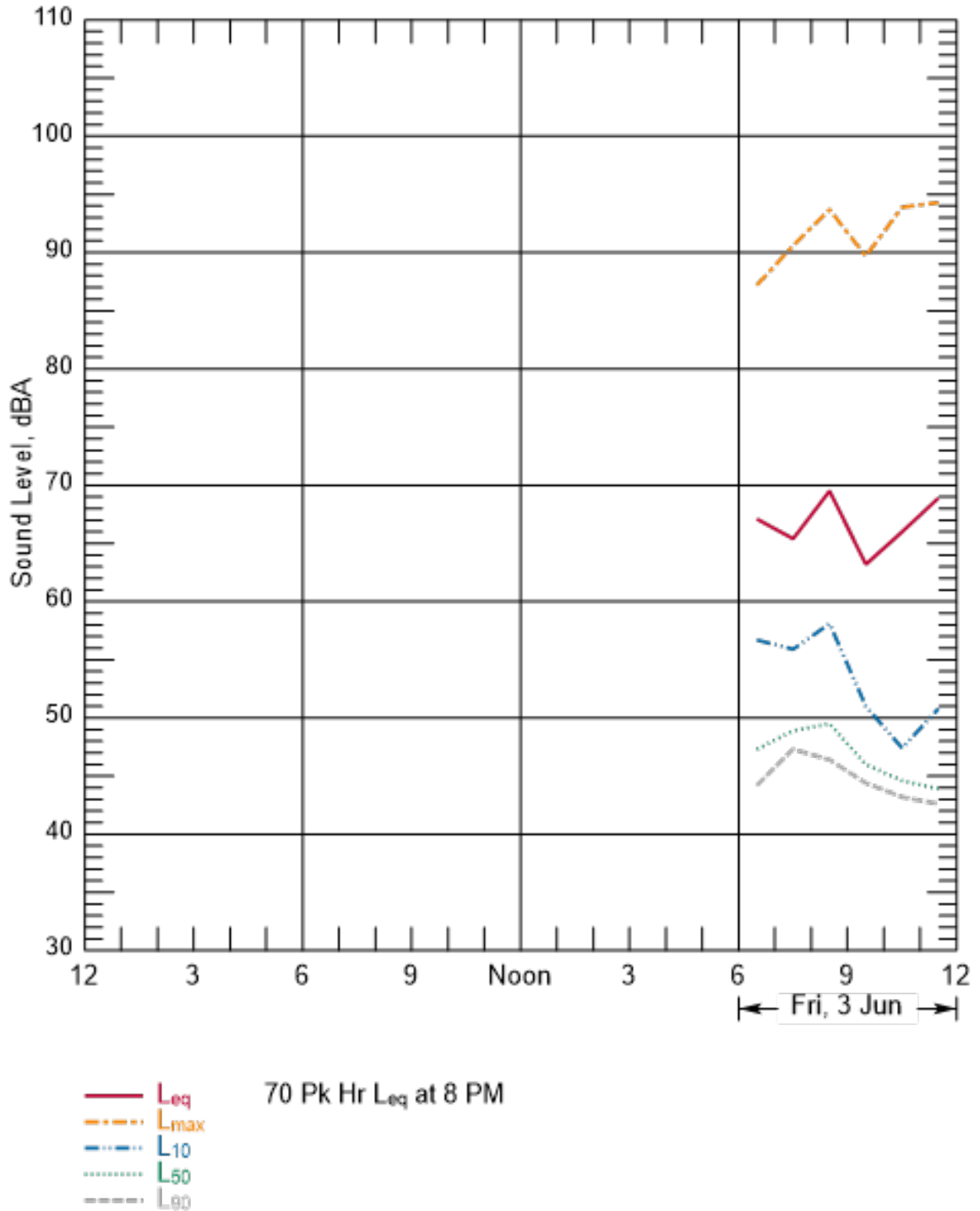
Figure B-147 Hourly Summary of Noise Levels Measured at N50 on June 3, 2016
