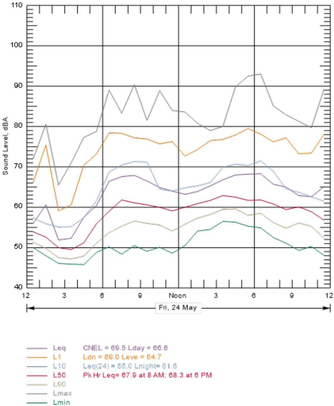
Figure B-210 Hourly Summary of Noise Levels Measured at N73 on May 24, 2013
