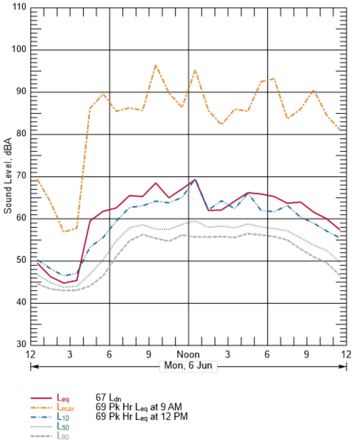
Figure B-173 Hourly Summary of Noise Levels Measured at N60 on June 6, 2016
