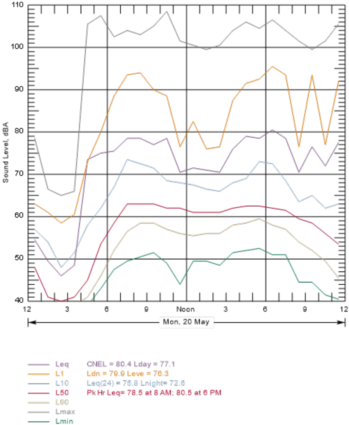
Figure B-180 Hourly Summary of Noise Levels Measured at N63 on May 20, 2013
