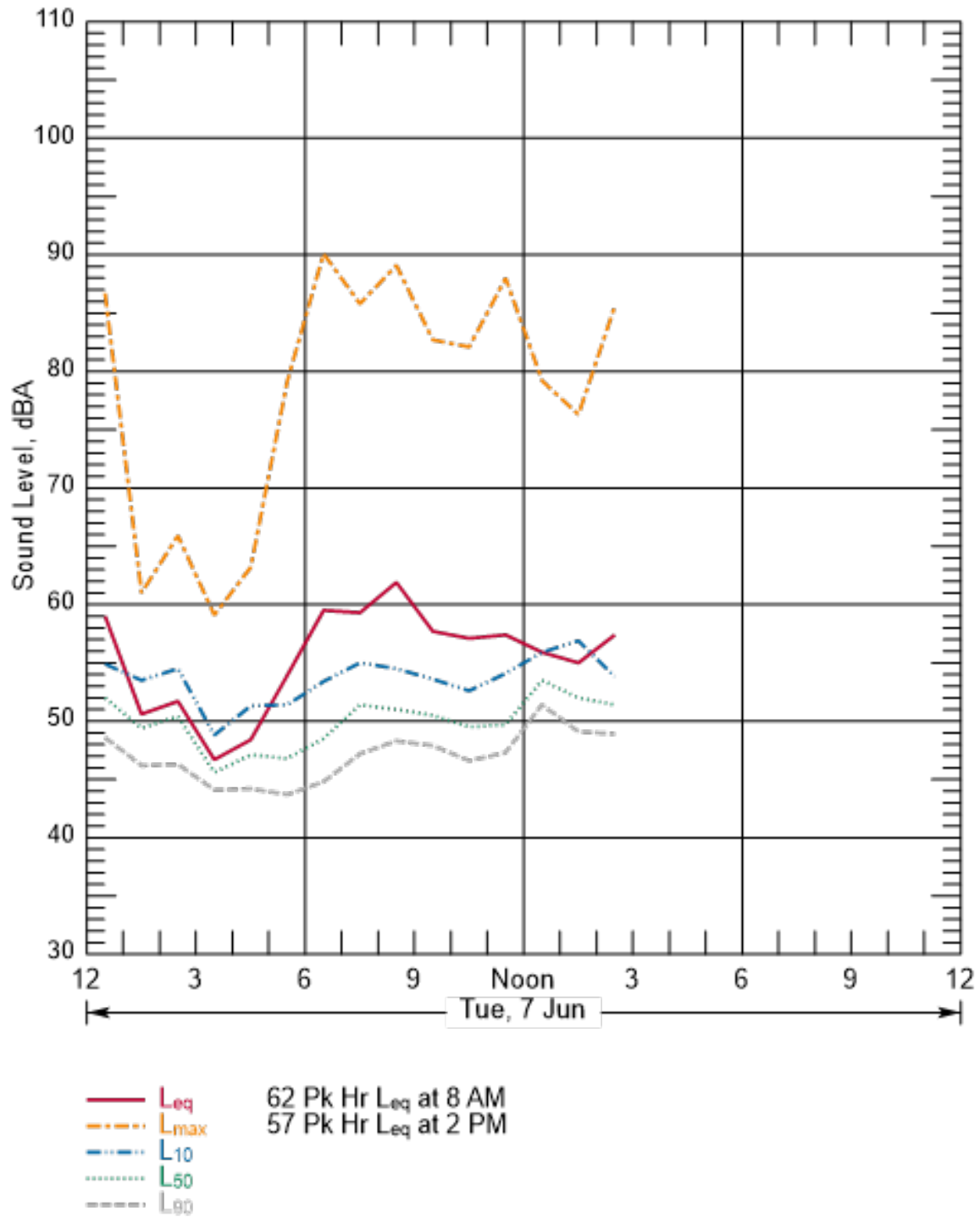
Figure B-160 Hourly Summary of Noise Levels Measured at N55 on June 7, 2016
