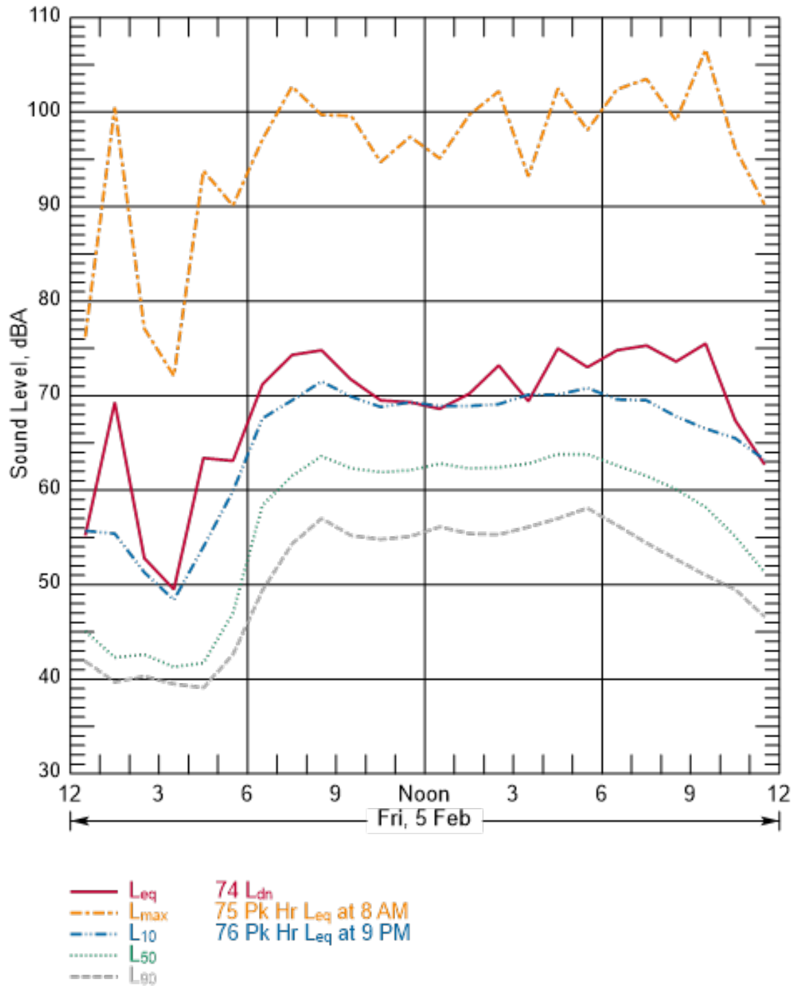
Figure B-202 Hourly Summary of Noise Levels Measured at N71 on February 5, 2010
