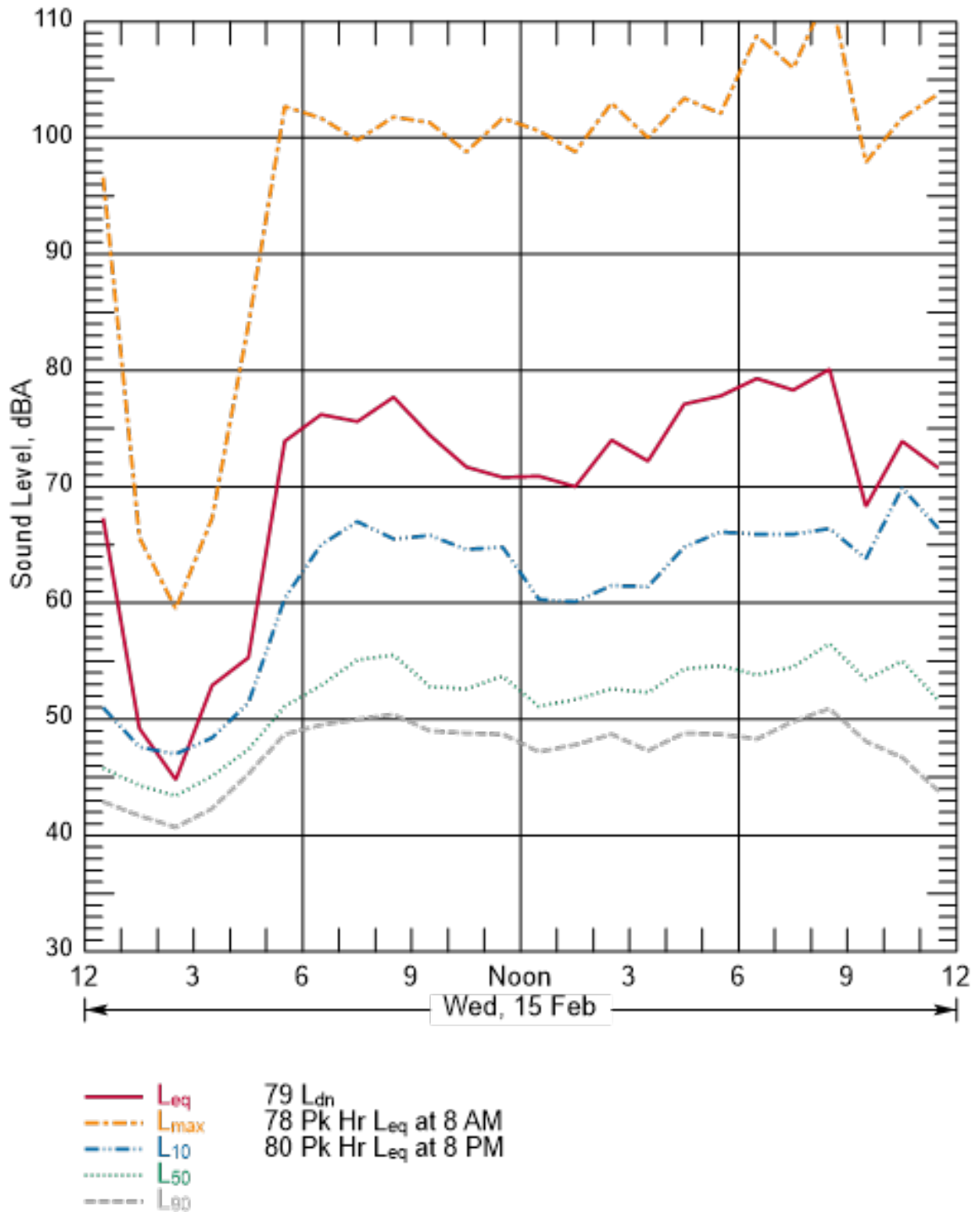
Figure B-95 Hourly Summary of Noise Levels Measured at N33 on February 15, 2017
