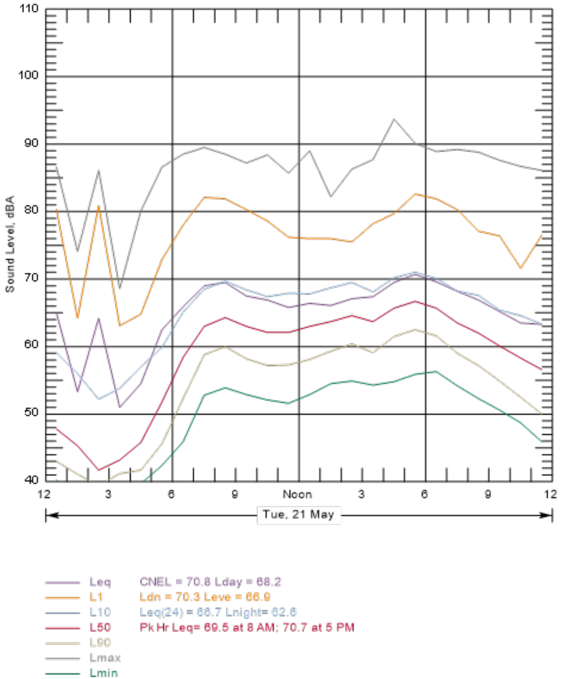
Figure B-119 Hourly Summary of Noise Levels Measured at N41 on May 21, 2013
