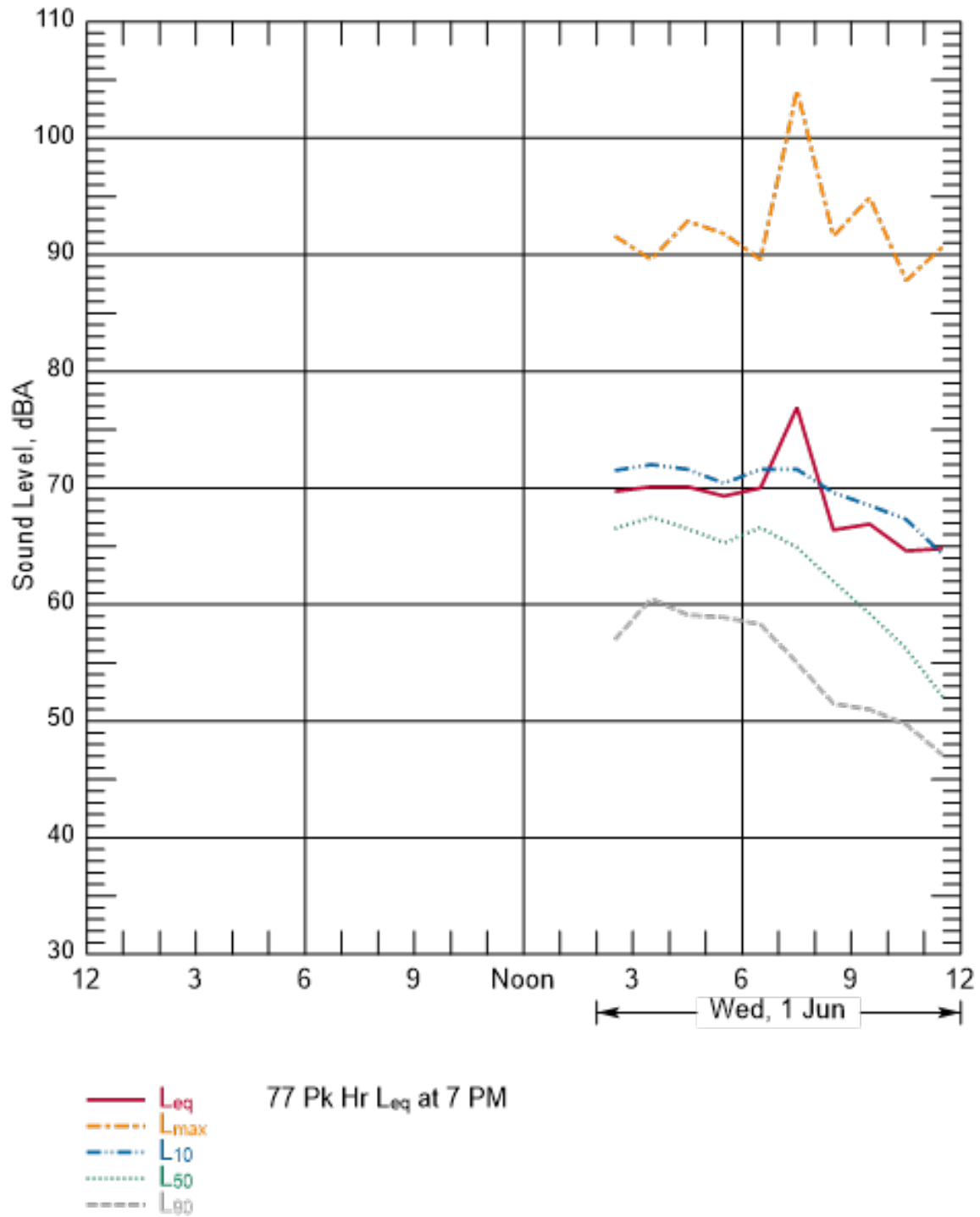
Figure B-86 Hourly Summary of Noise Levels Measured at N30 on June 1, 2016
