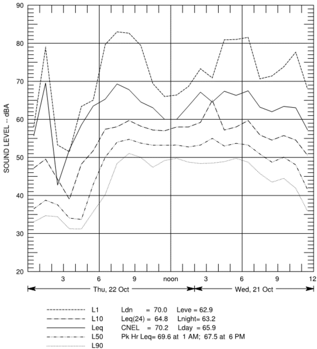
Figure B-194 Hourly Summary of Noise Levels Measured at N67 on October 21 and 22, 2010
