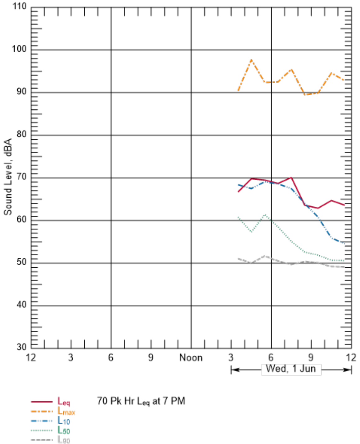
Figure B-113 Hourly Summary of Noise Levels Measured at N39 on June 1, 2016
