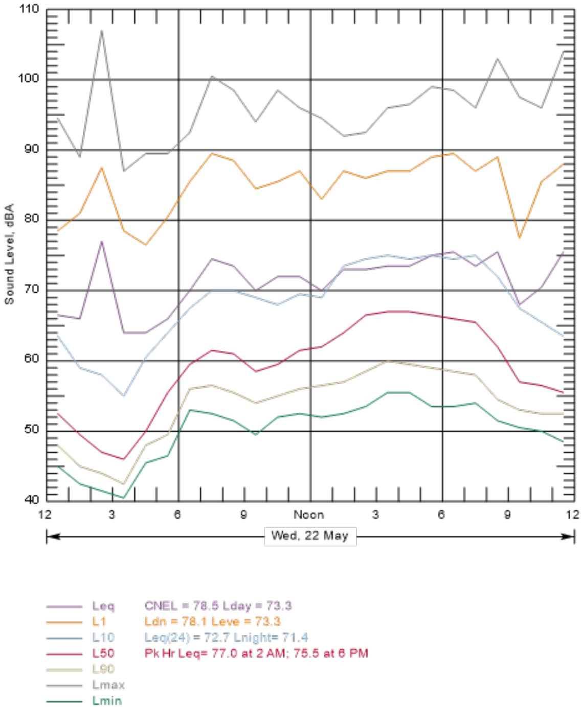
Figure B-52 Hourly Summary of Noise Levels Measured at N18 on May 22, 2013
