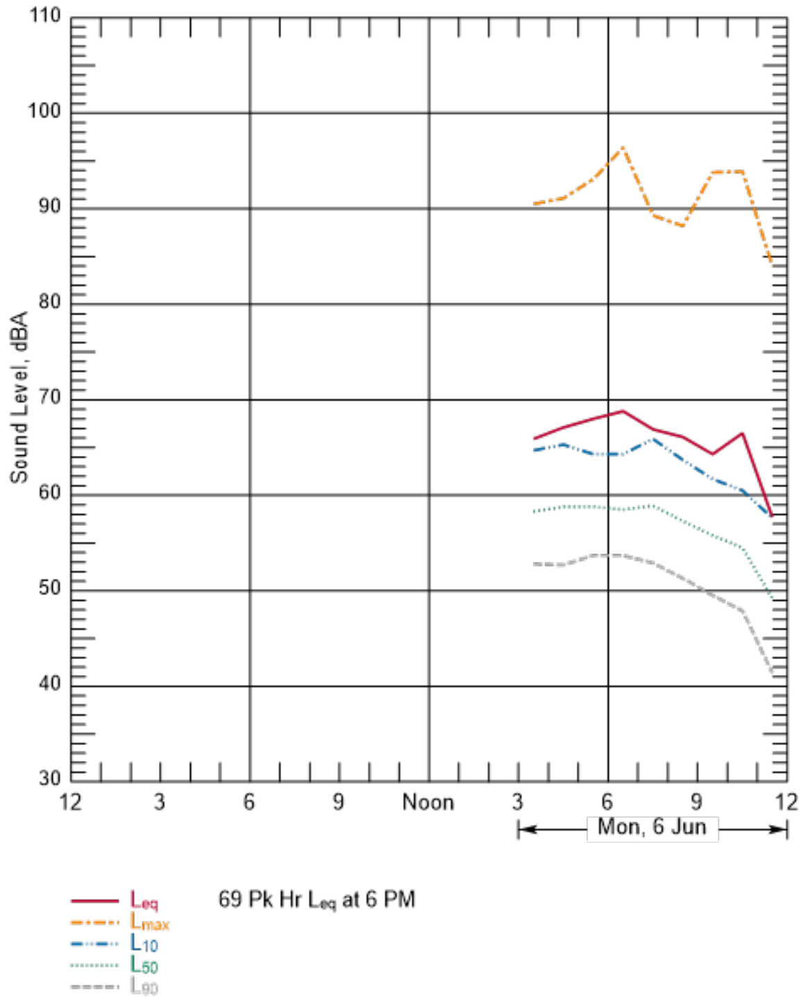
Figure B-190 Hourly Summary of Noise Levels Measured at N66 on June 6, 2016
