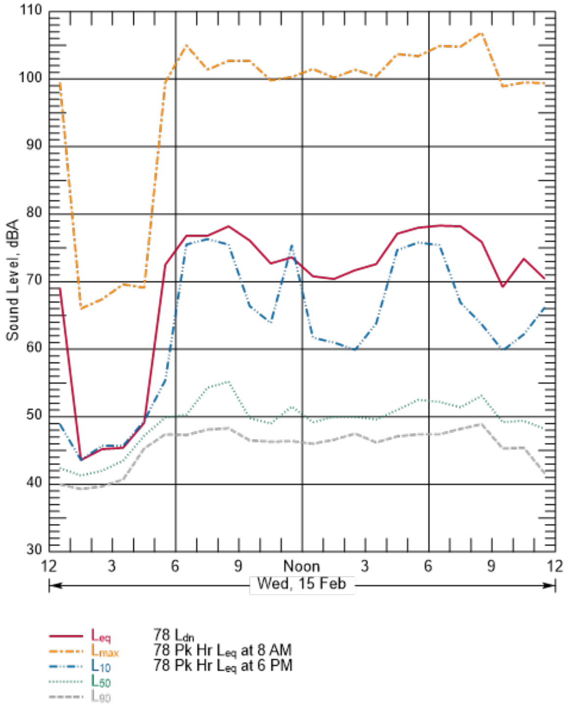
Figure B-99 Hourly Summary of Noise Levels Measured at N34 on February 15, 2017
