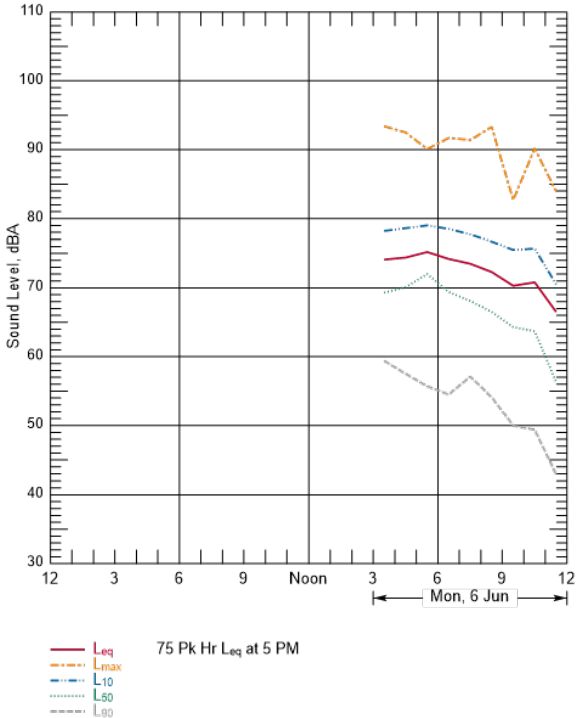
Figure B-187 Hourly Summary of Noise Levels Measured at N65 on June 6, 2016
