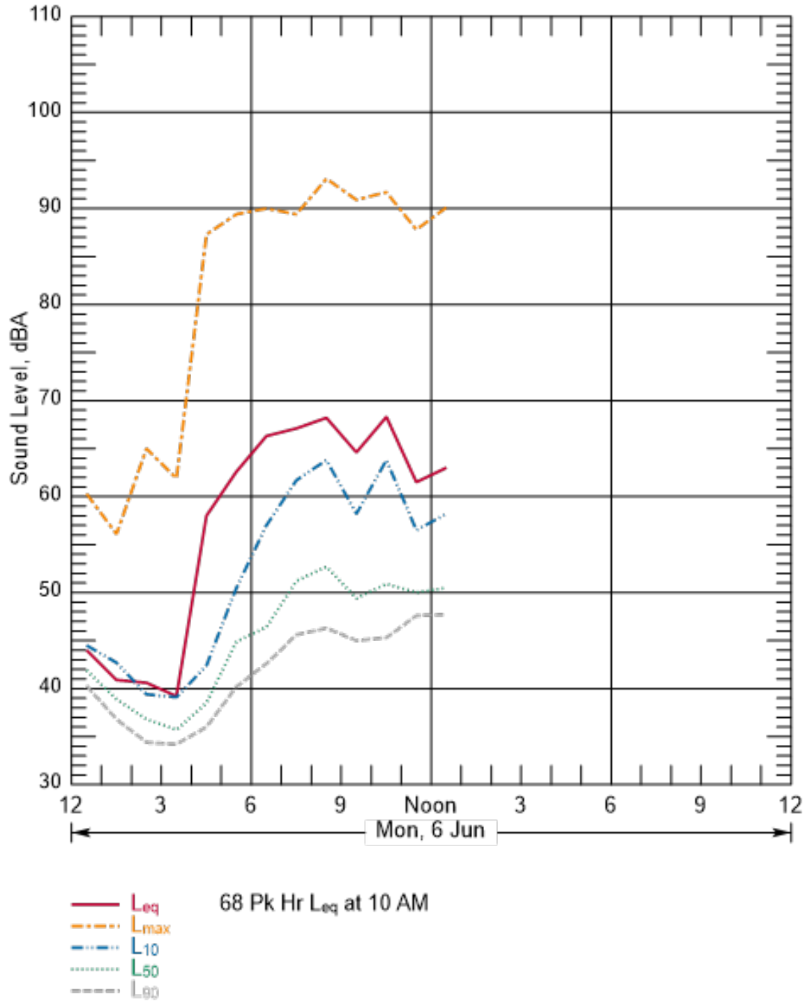
Figure B-146 Hourly Summary of Noise Levels Measured at N49 on June 6, 2016
