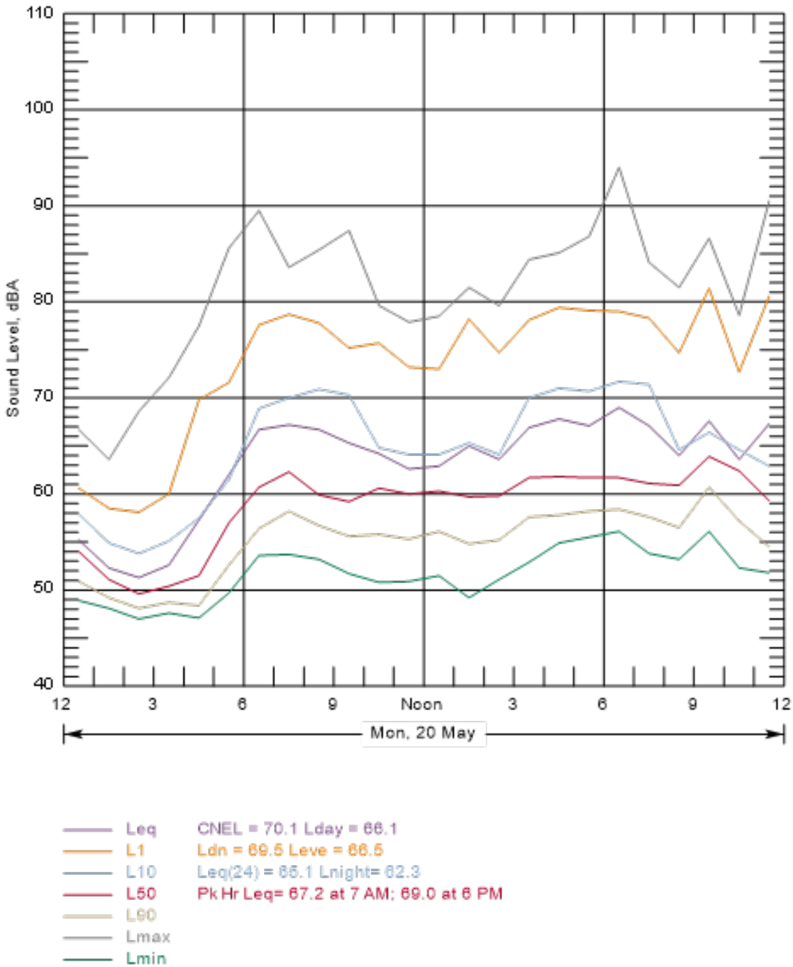
Figure B-206 Hourly Summary of Noise Levels Measured at N73 on May 20, 2013
