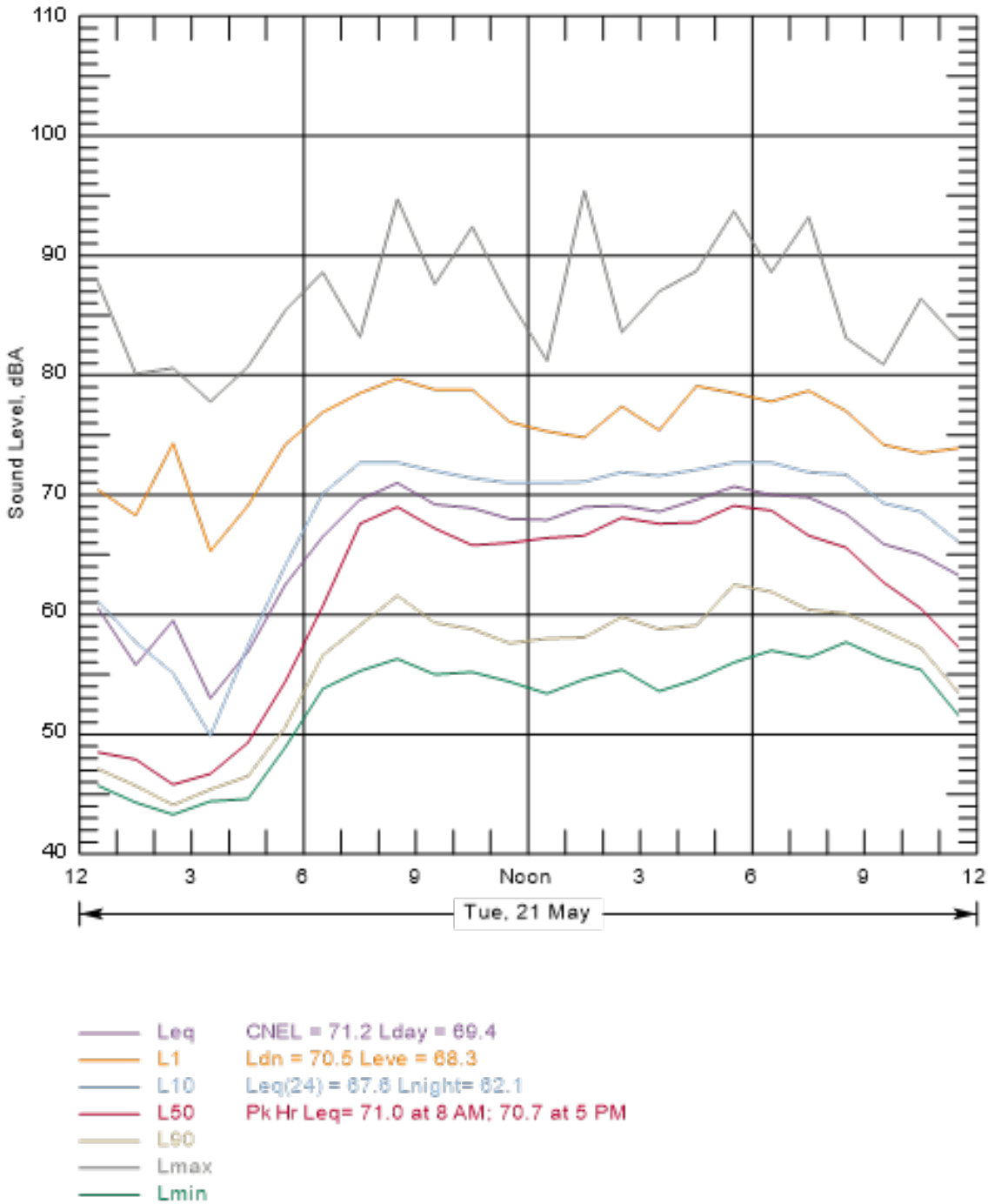
Figure B-82 Hourly Summary of Noise Levels Measured at N29 on May 21, 2013
