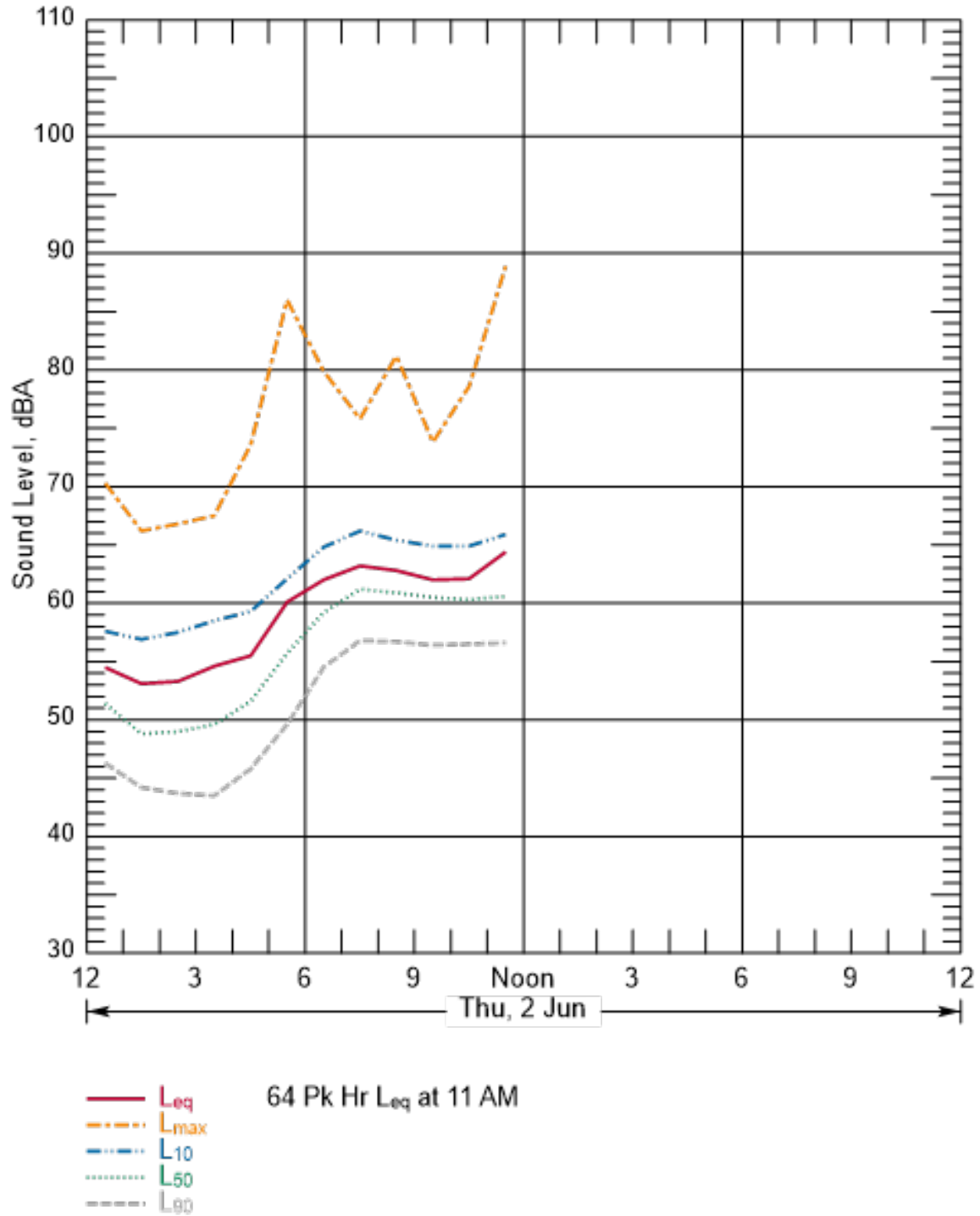
Figure B-40 Hourly Summary of Noise Levels Measured at N13 on June 2, 2016
