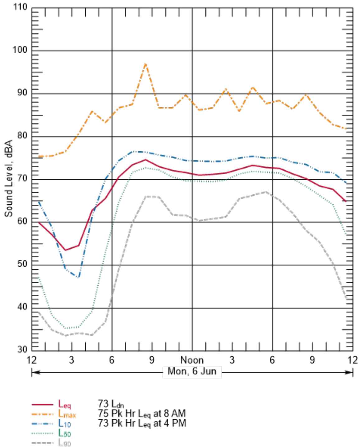
Figure B-176 Hourly Summary of Noise Levels Measured at N61 on June 6, 2016
