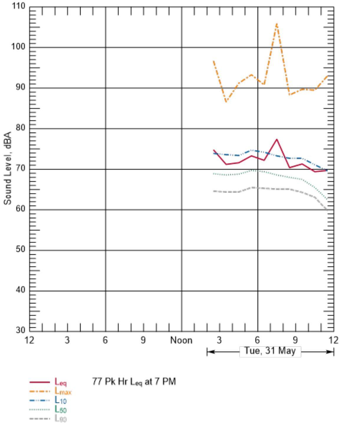
Figure B-57 Hourly Summary of Noise Levels Measured at N20 on May 31, 2016
