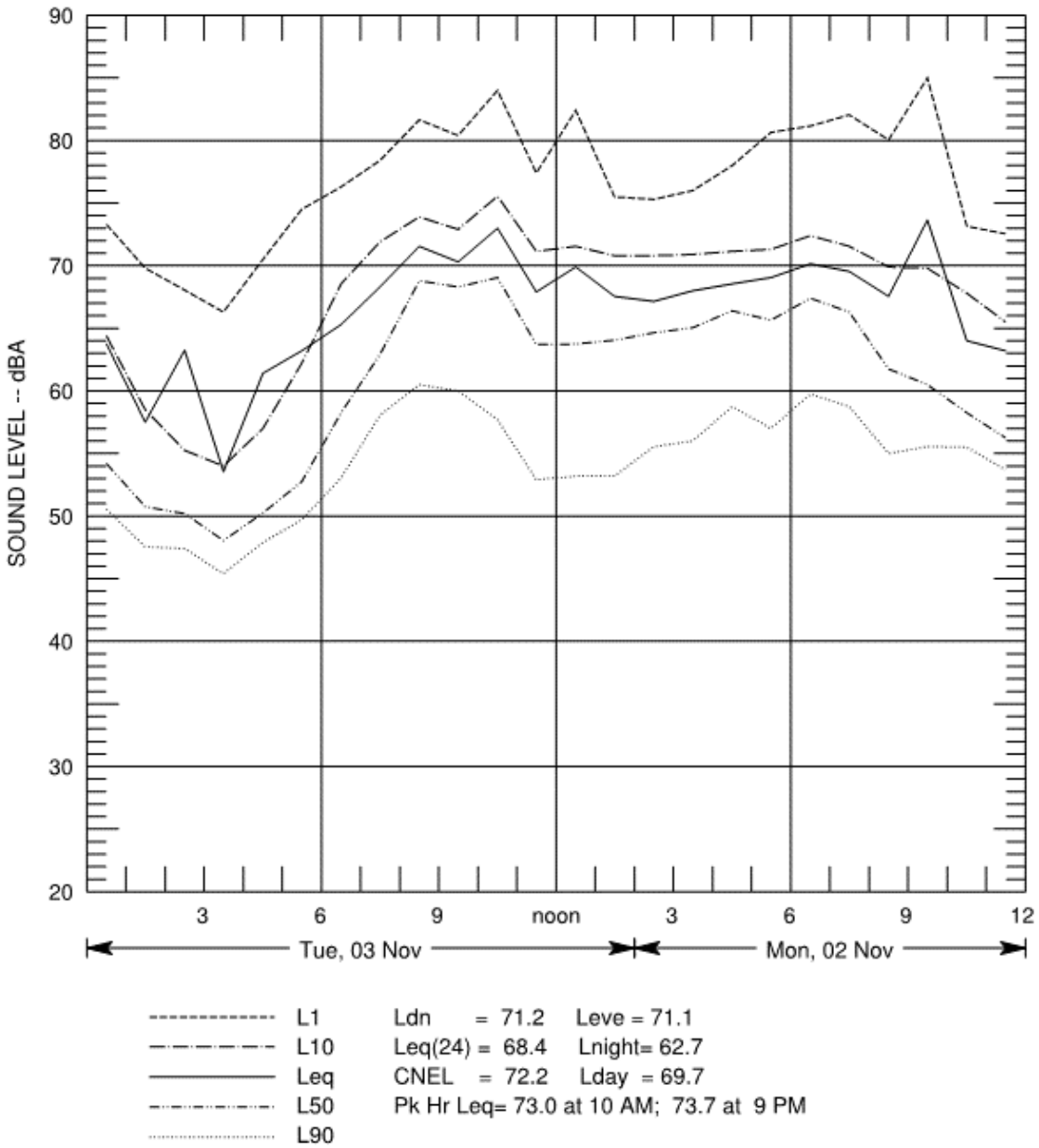
Figure B-92 Hourly Summary of Noise Levels Measured at N32 on November 2 and 3, 2010
