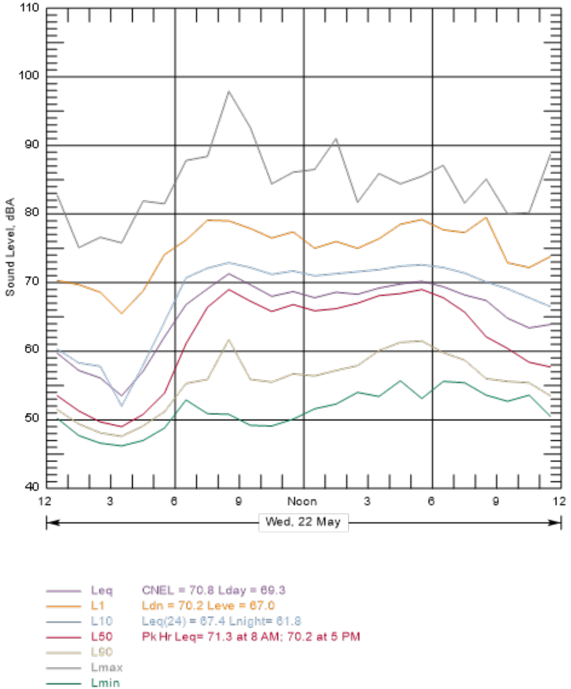
Figure B-83 Hourly Summary of Noise Levels Measured at N29 on May 22, 2013
