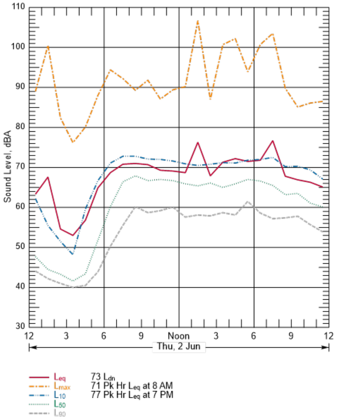
Figure B-87 Hourly Summary of Noise Levels Measured at N30 on June 2, 2016
