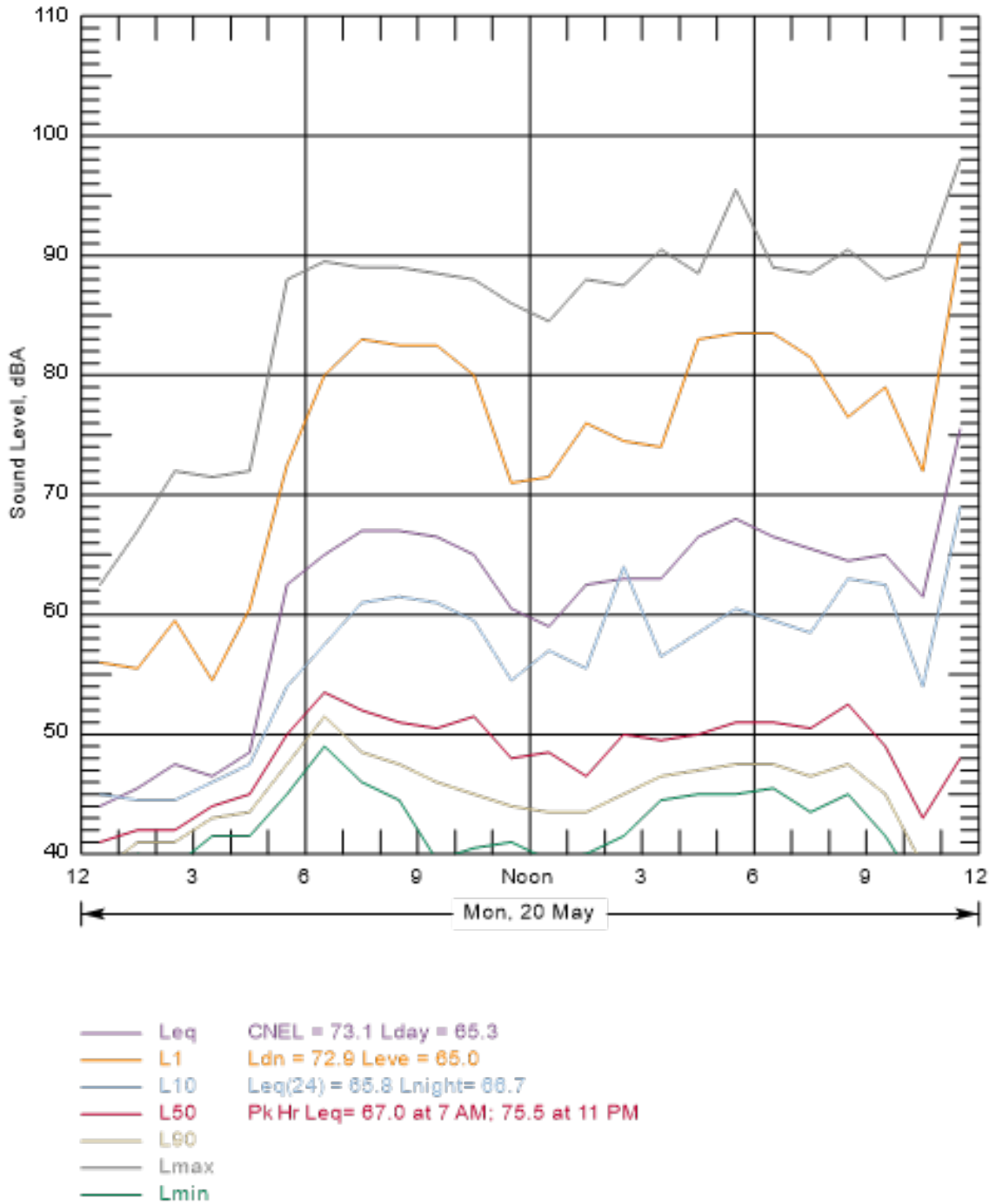
Figure B-139 Hourly Summary of Noise Levels Measured at N48 on May 20, 2013
