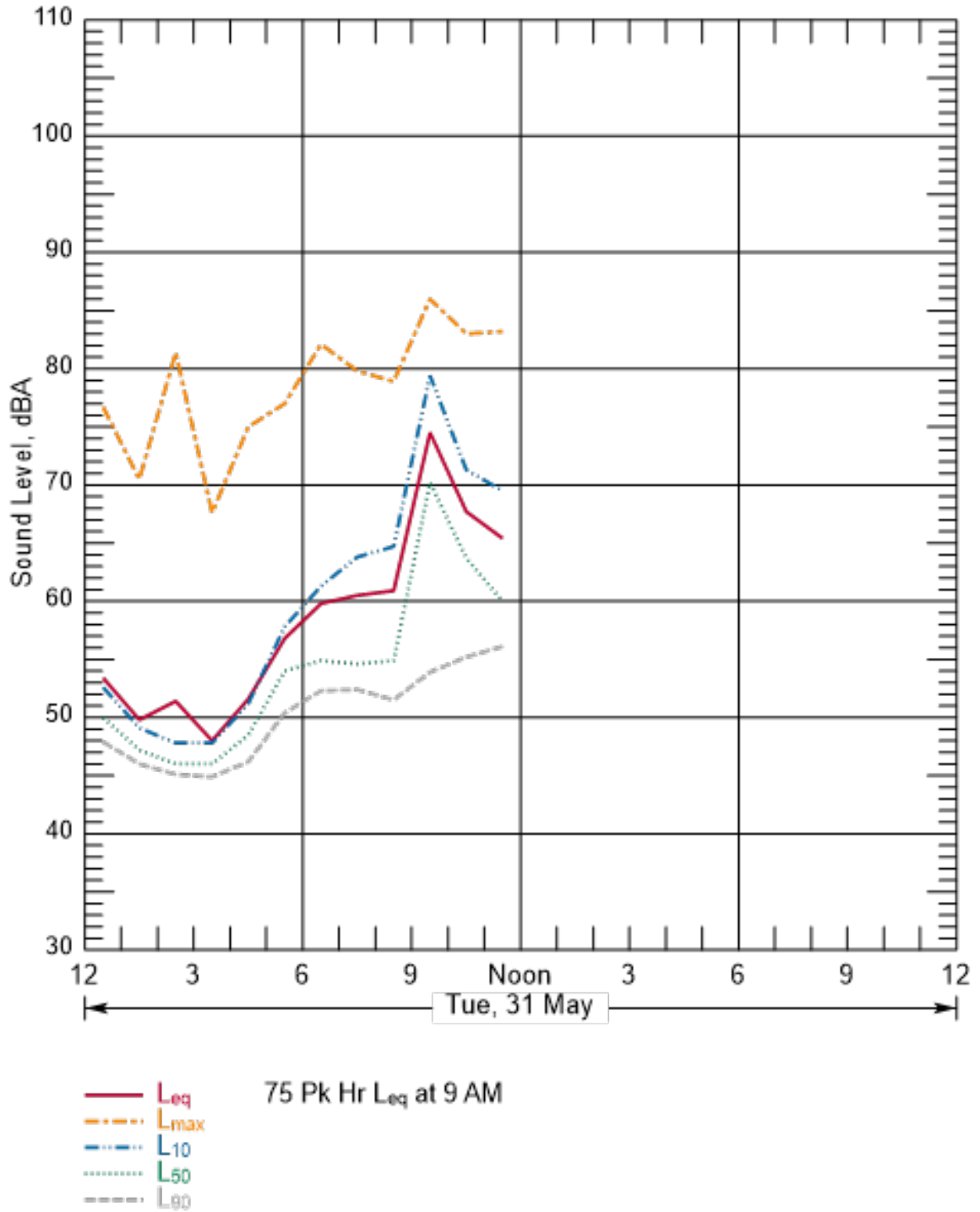
Figure B-33 Hourly Summary of Noise Levels Measured at N11 on May 31, 2016
