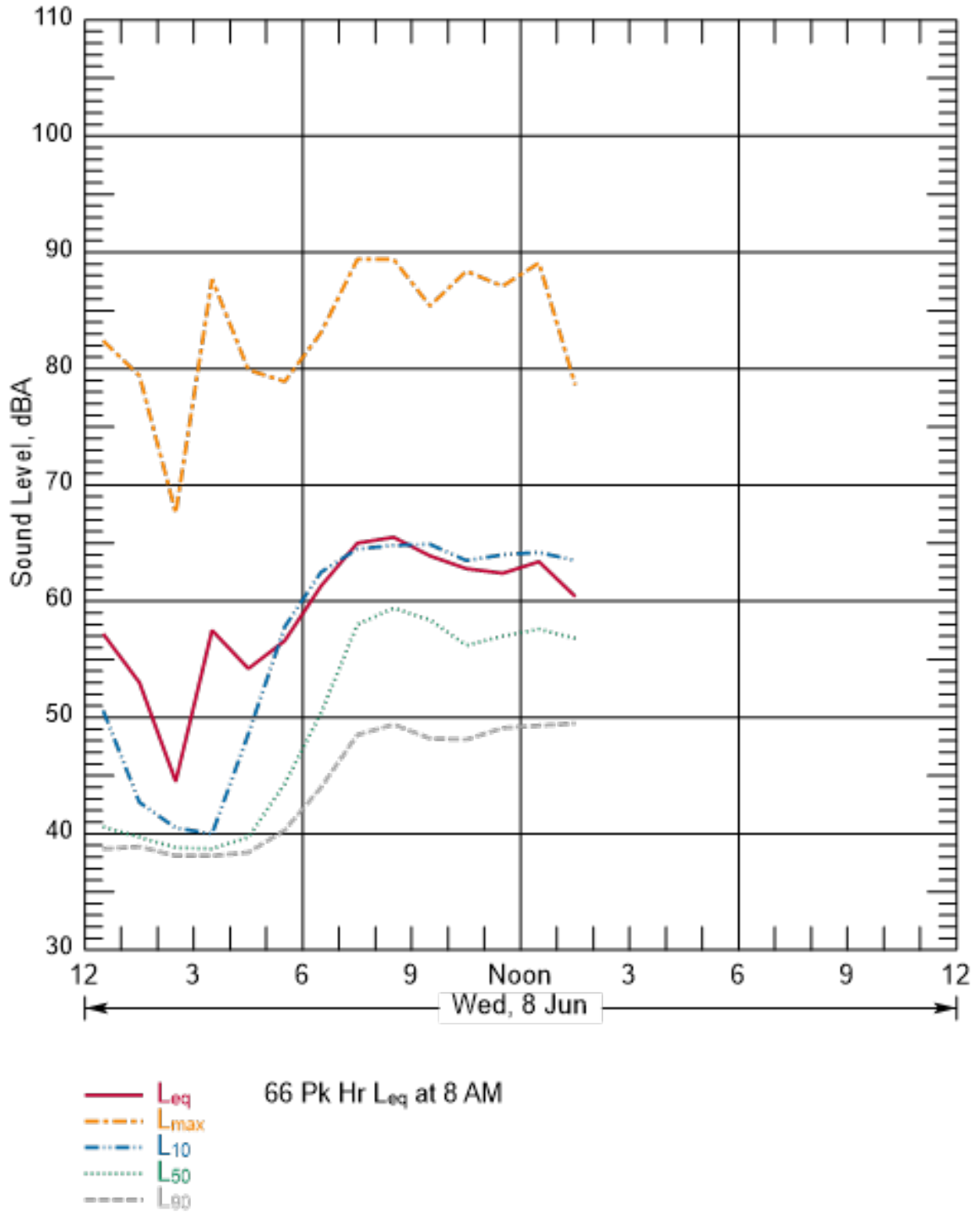
Figure B-201 Hourly Summary of Noise Levels Measured at N70 on June 8, 2016
