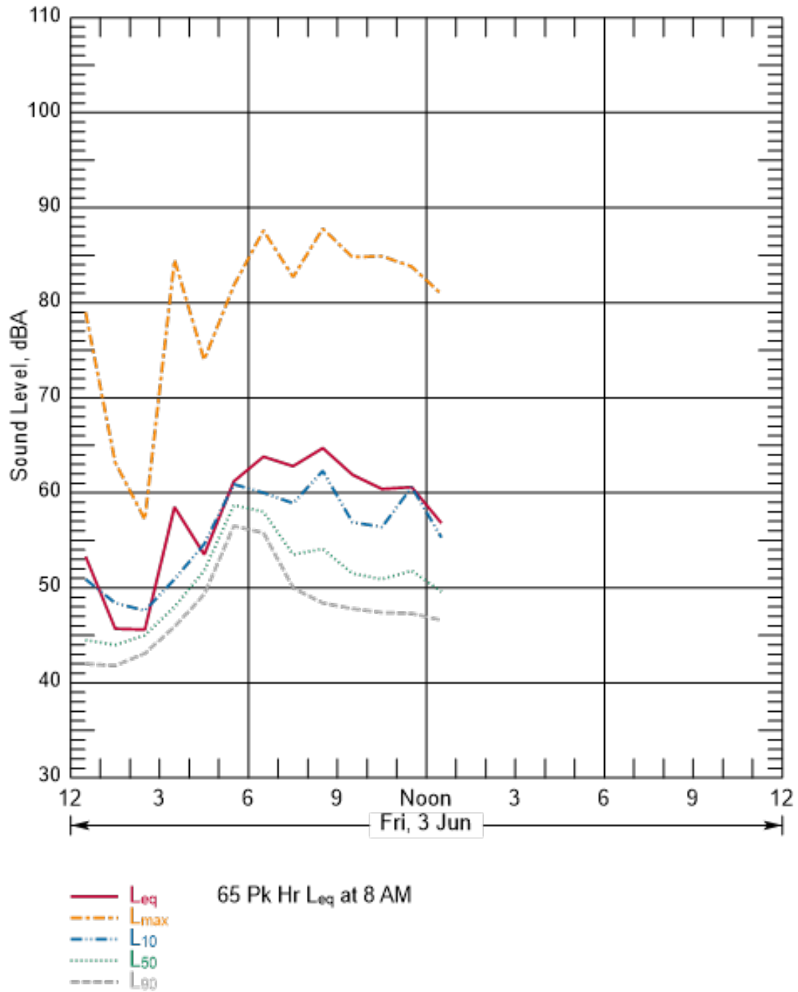
Figure B-110 Hourly Summary of Noise Levels Measured at N37 on June 3, 2016
