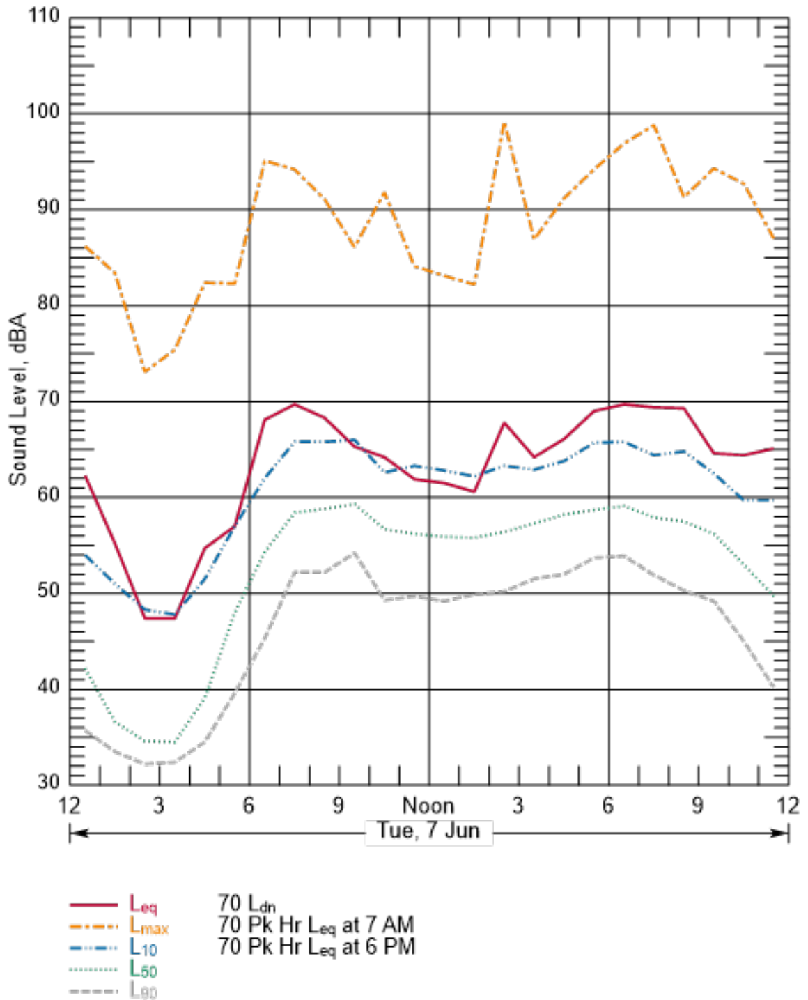
Figure B-191 Hourly Summary of Noise Levels Measured at N66 on June 7, 2016
