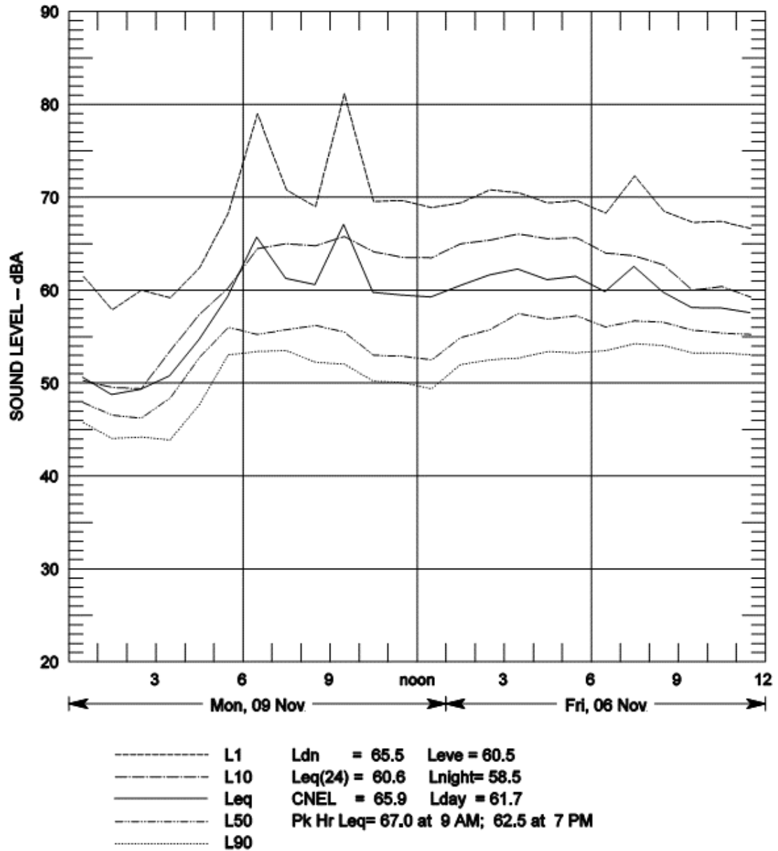
Figure B-9 Hourly Summary of Noise Levels Measured at N03 on November 6 and 9, 2009
