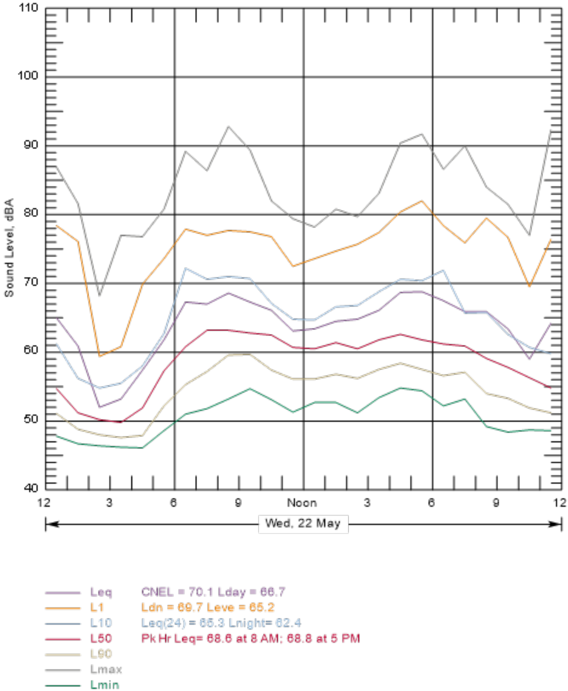
Figure B-208 Hourly Summary of Noise Levels Measured at N73 on May 22, 2013
