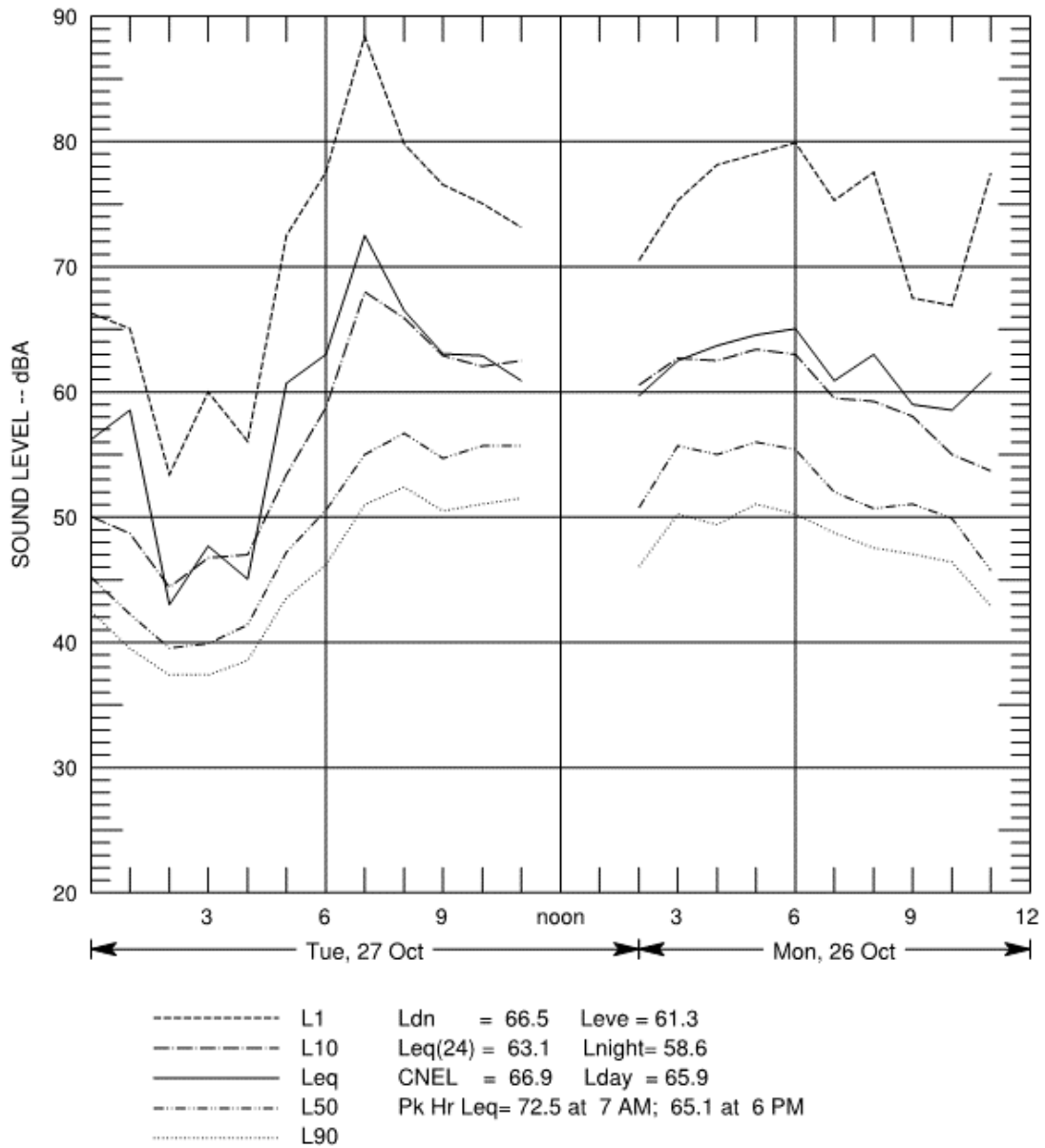
Figure B-157 Hourly Summary of Noise Levels Measured at N54 on October 26 and 27, 2010
