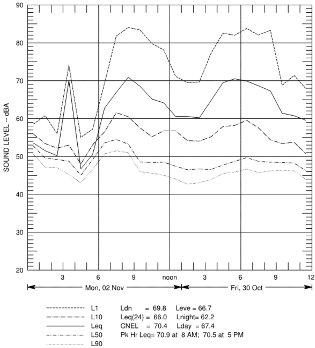
Figure B-106 Hourly Summary of Noise Levels Measured at N36 on October 30 and November 2, 2010
