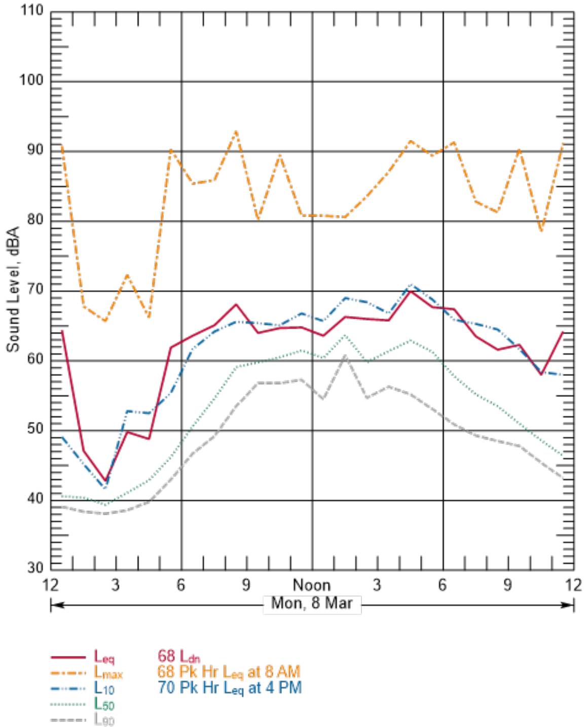
Figure B-155 Hourly Summary of Noise Levels Measured at N53 on March 8, 2010
