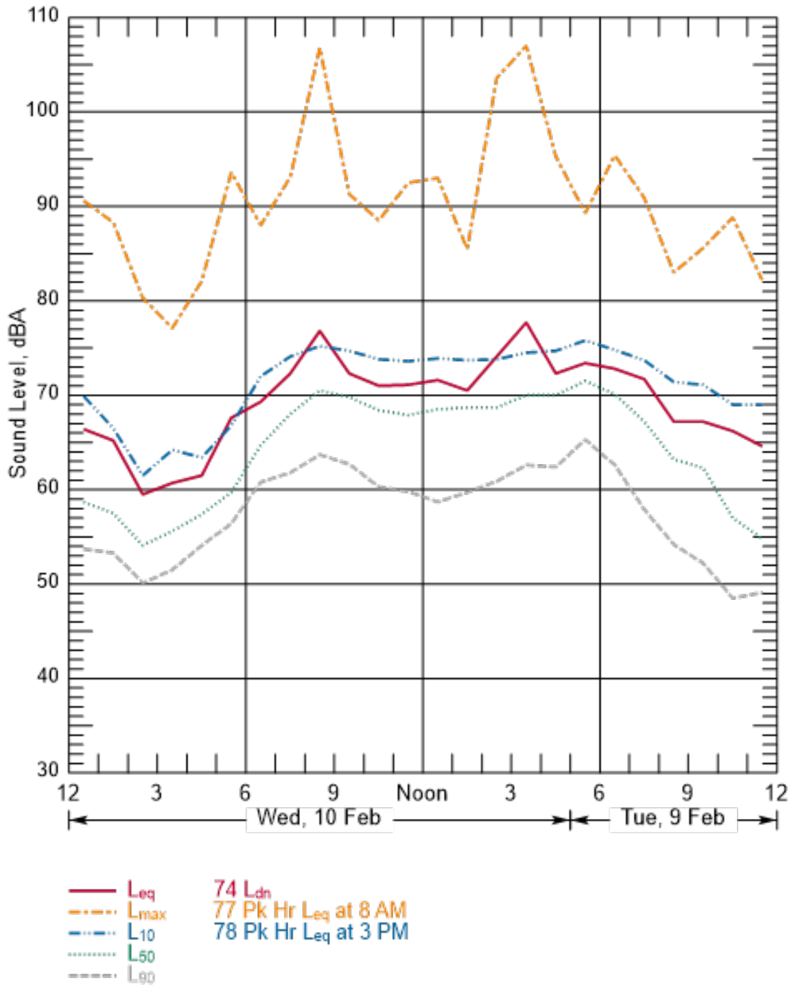
Figure B-89 Hourly Summary of Noise Levels Measured at N31 on February 9 and 10, 2010
