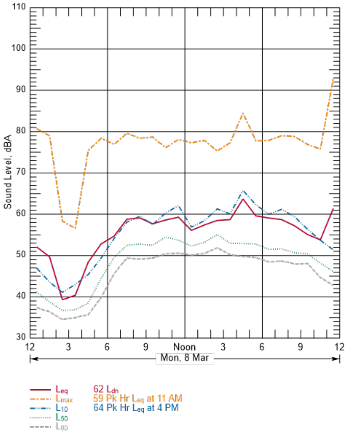
Figure B-179 Hourly Summary of Noise Levels Measured at N62 on March 8, 2010
