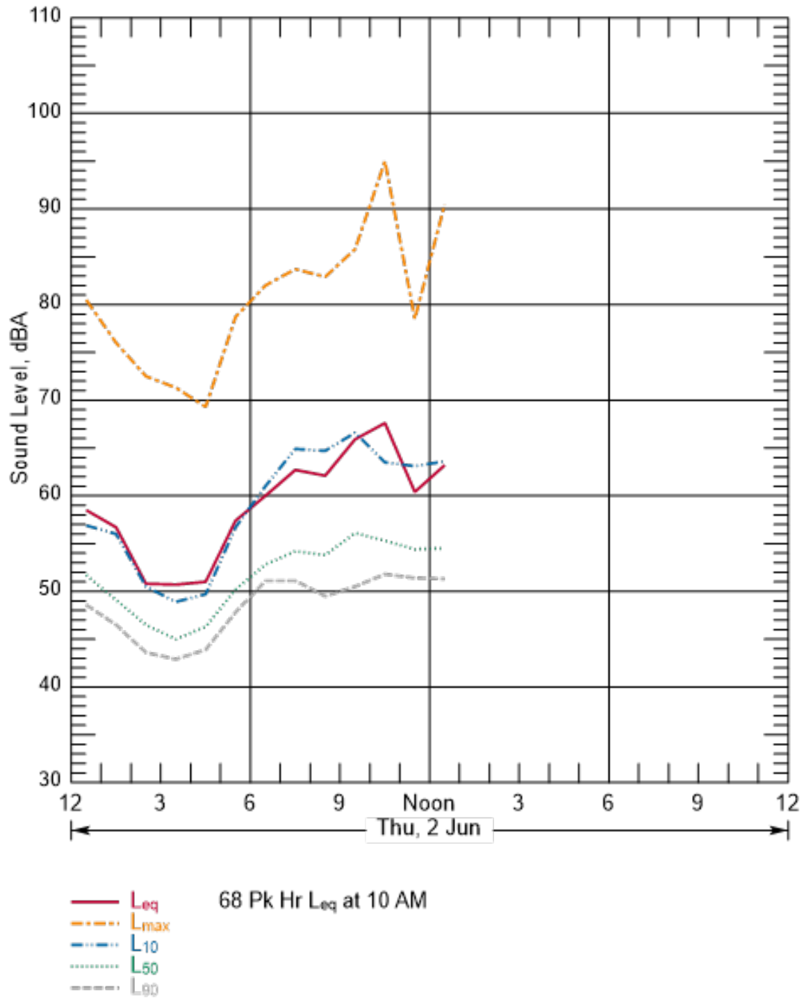
Figure B-64 Hourly Summary of Noise Levels Measured at N22 on June 2, 2016
