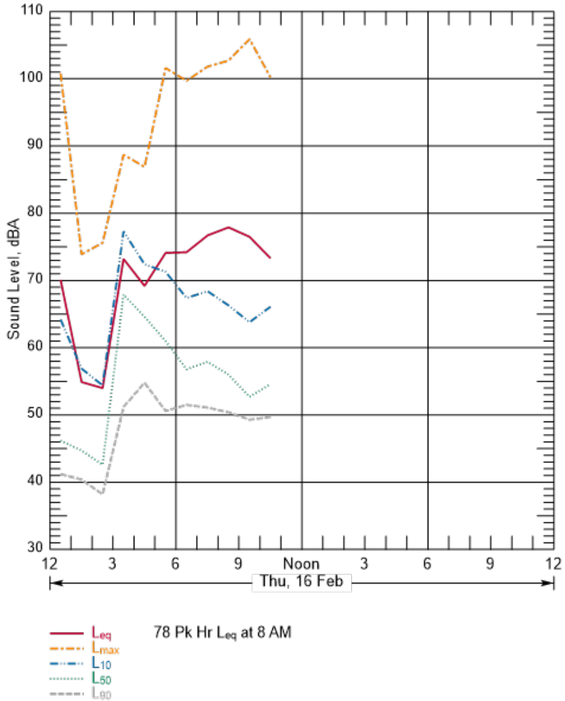
Figure B-96 Hourly Summary of Noise Levels Measured at N33 on February 16, 2017
