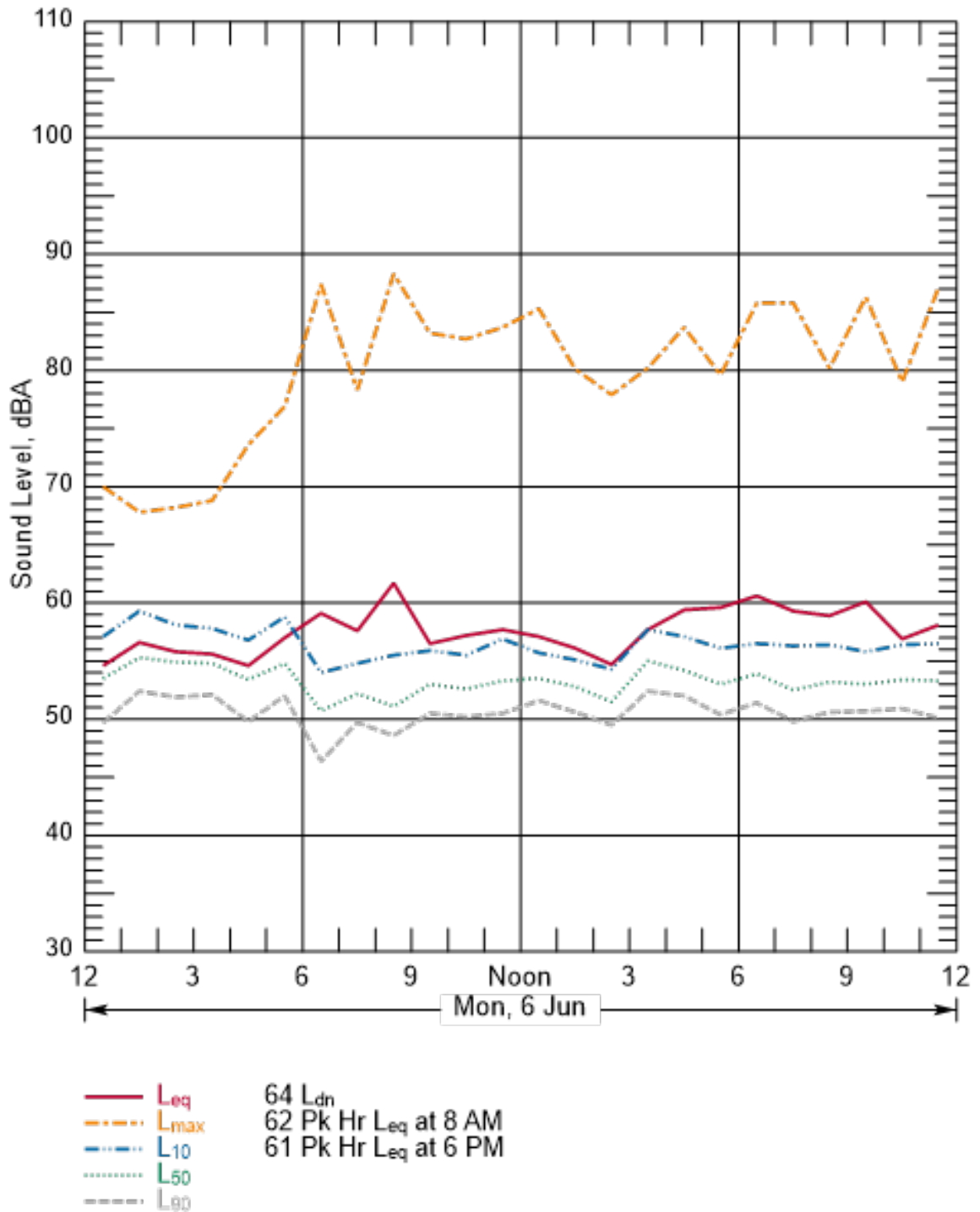
Figure B-159 Hourly Summary of Noise Levels Measured at N55 on June 6, 2016
