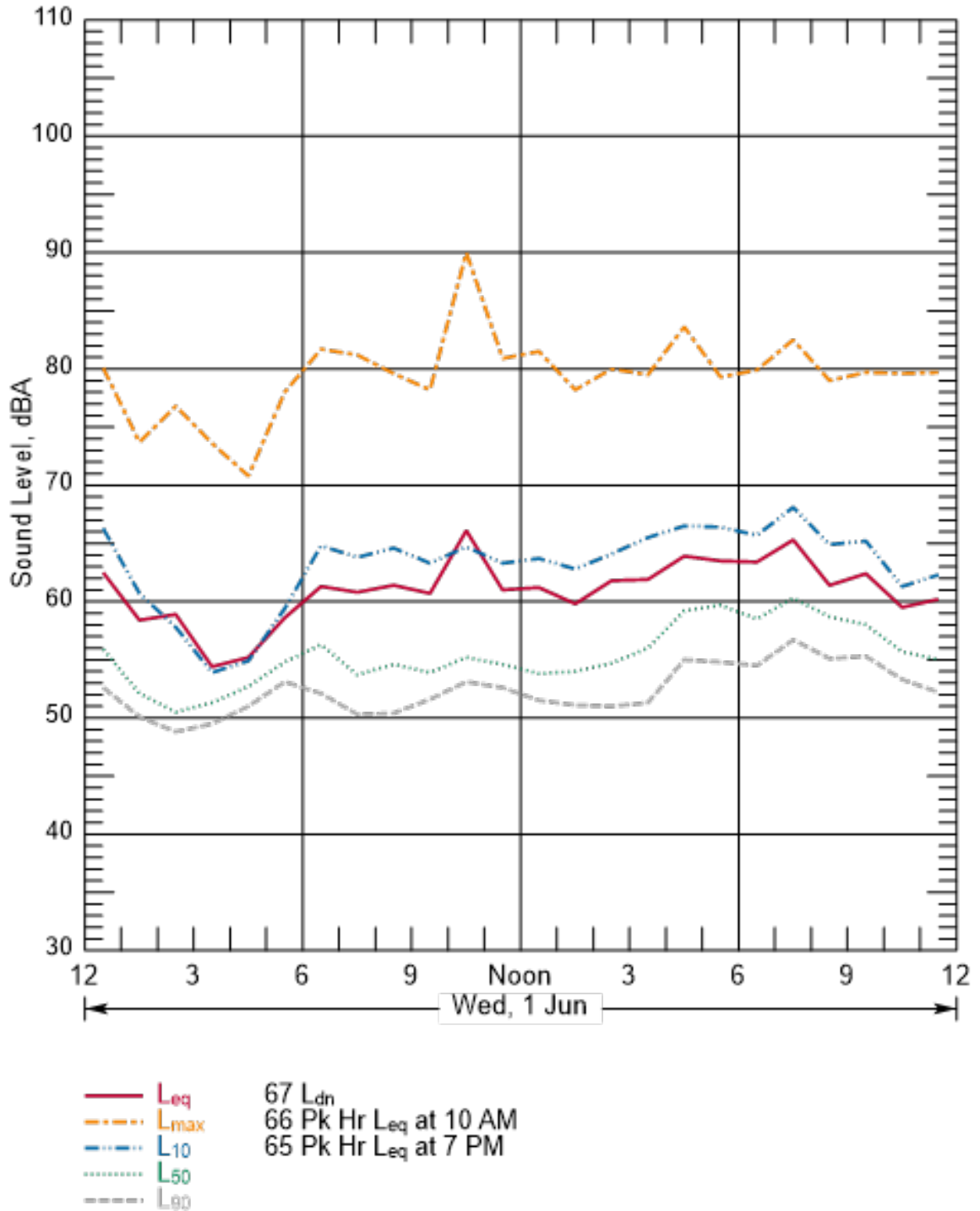
Figure B-63 Hourly Summary of Noise Levels Measured at N22 on June 1, 2016
