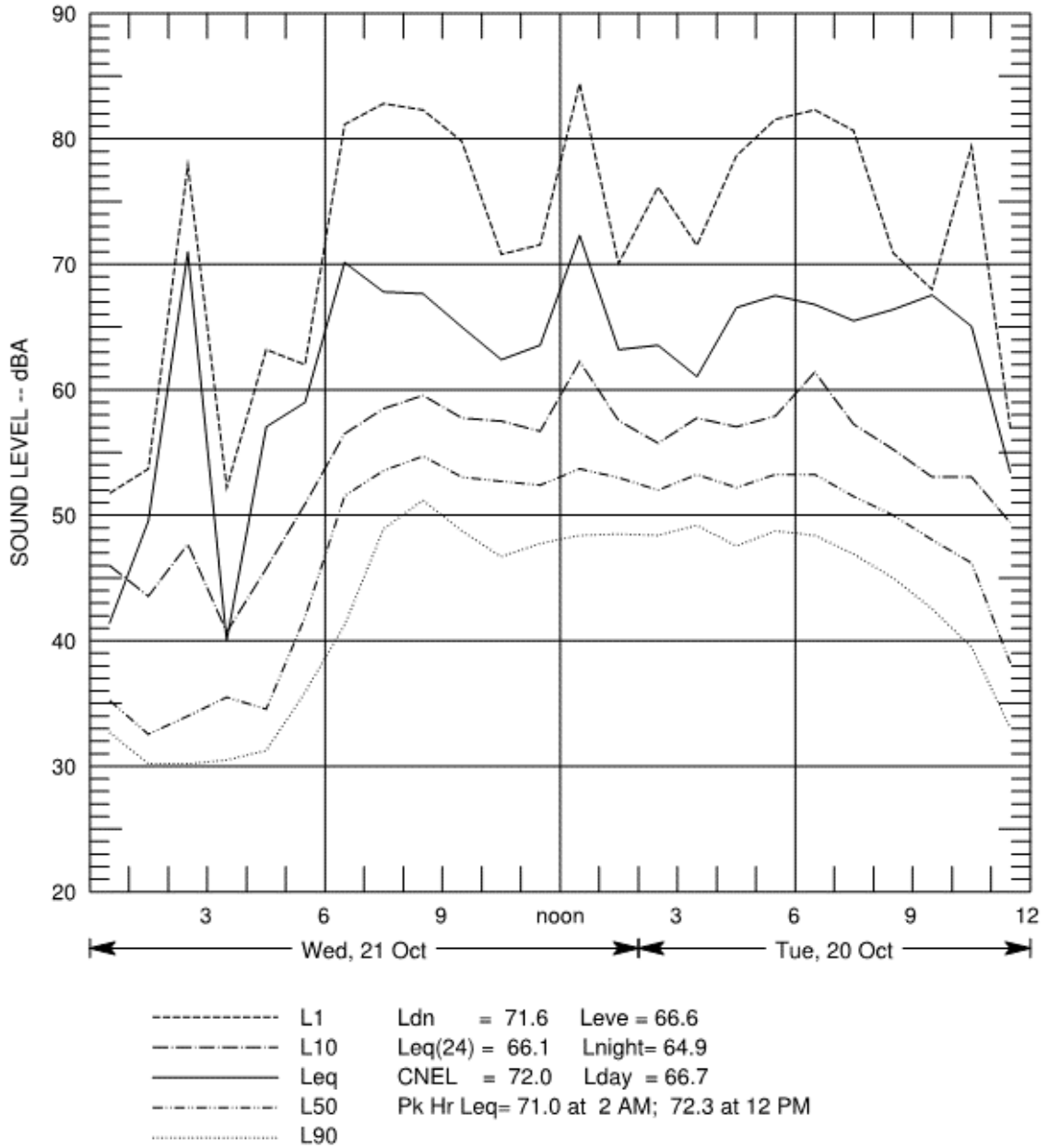
Figure B-193 Hourly Summary of Noise Levels Measured at N67 on October 20 and 21, 2010
