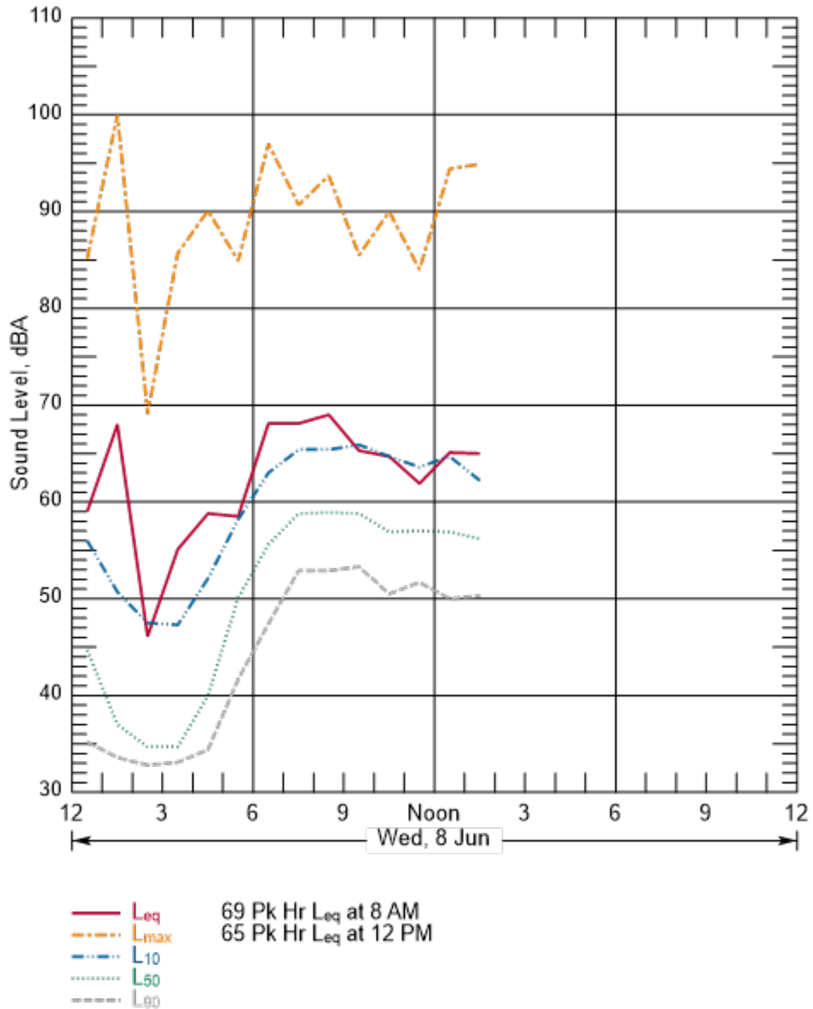
Figure B-192 Hourly Summary of Noise Levels Measured at N66 on June 8, 2016
