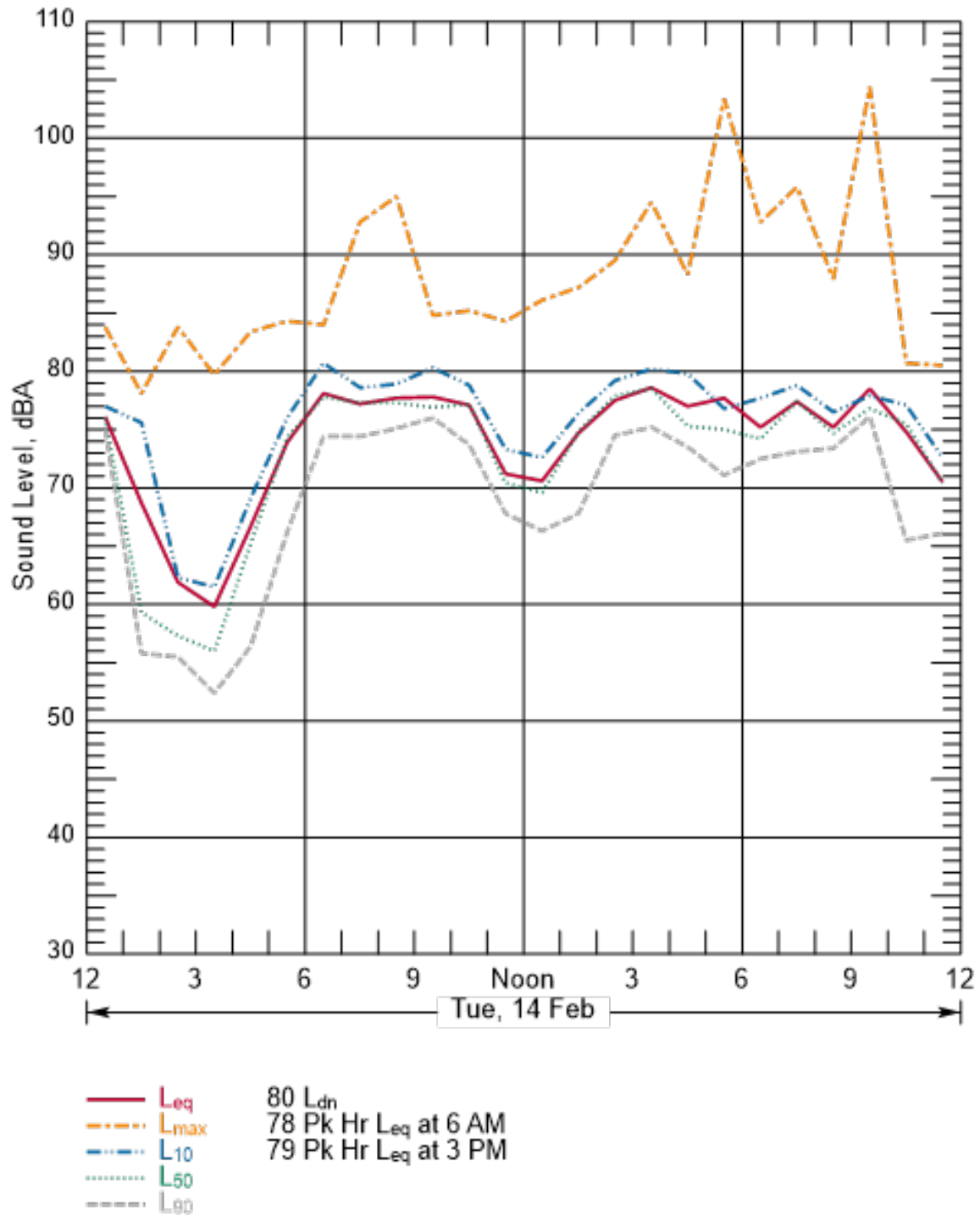
Figure B-2 Hourly Summary of Noise Levels Measured at N01 on February 14, 2017
