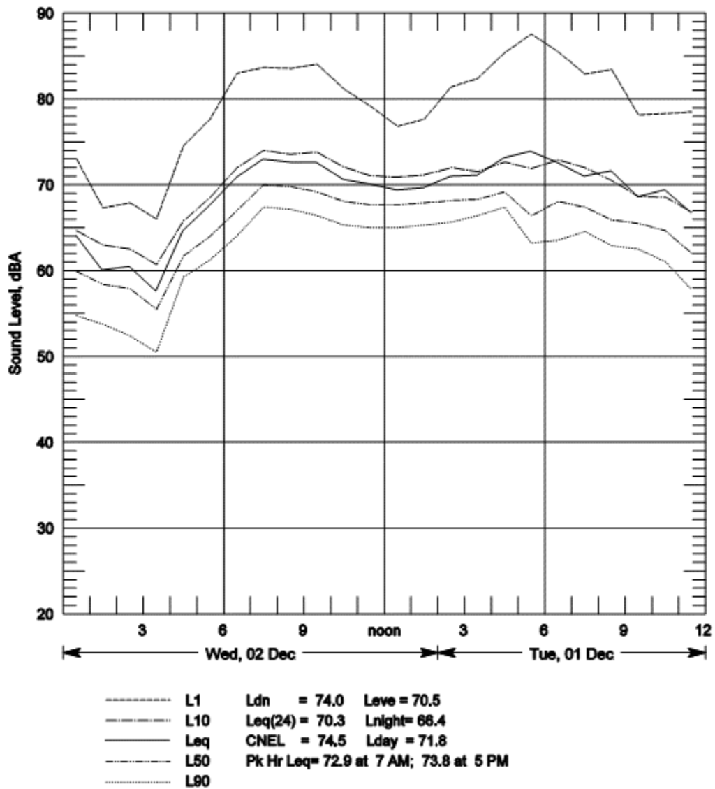
Figure B-12 Hourly Summary of Noise Levels Measured at N04 on December 1 and 2, 2009
