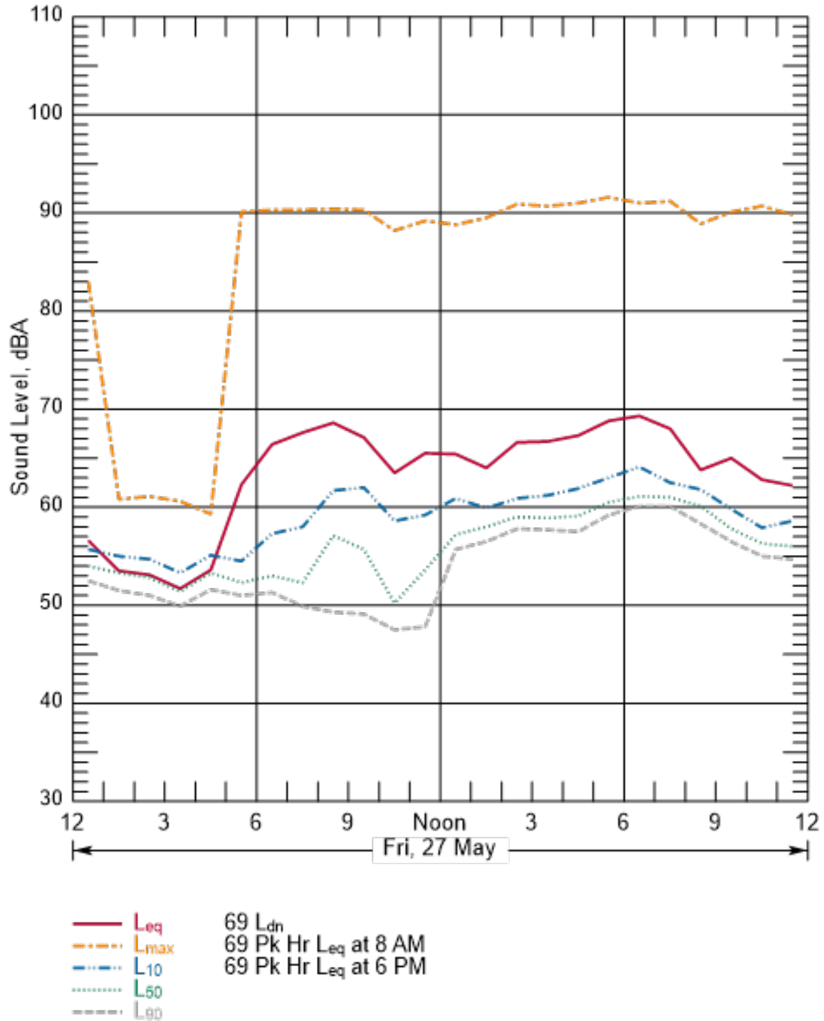
Figure B-16 Hourly Summary of Noise Levels Measured at N06 on May 27, 2016
