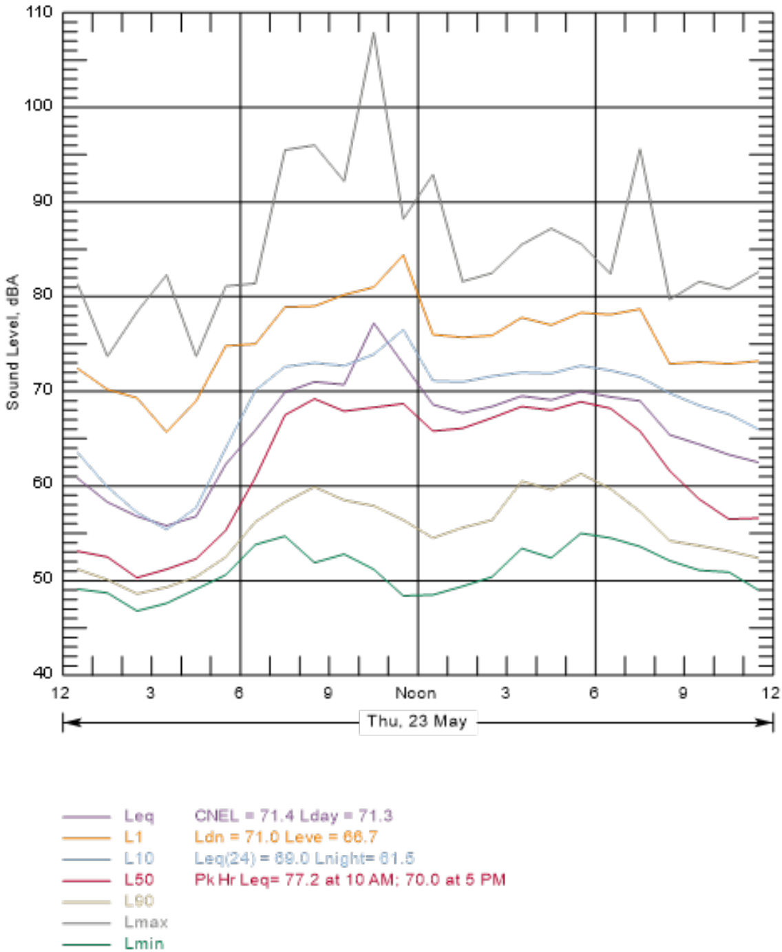
Figure B-84 Hourly Summary of Noise Levels Measured at N29 on May 23, 2013
