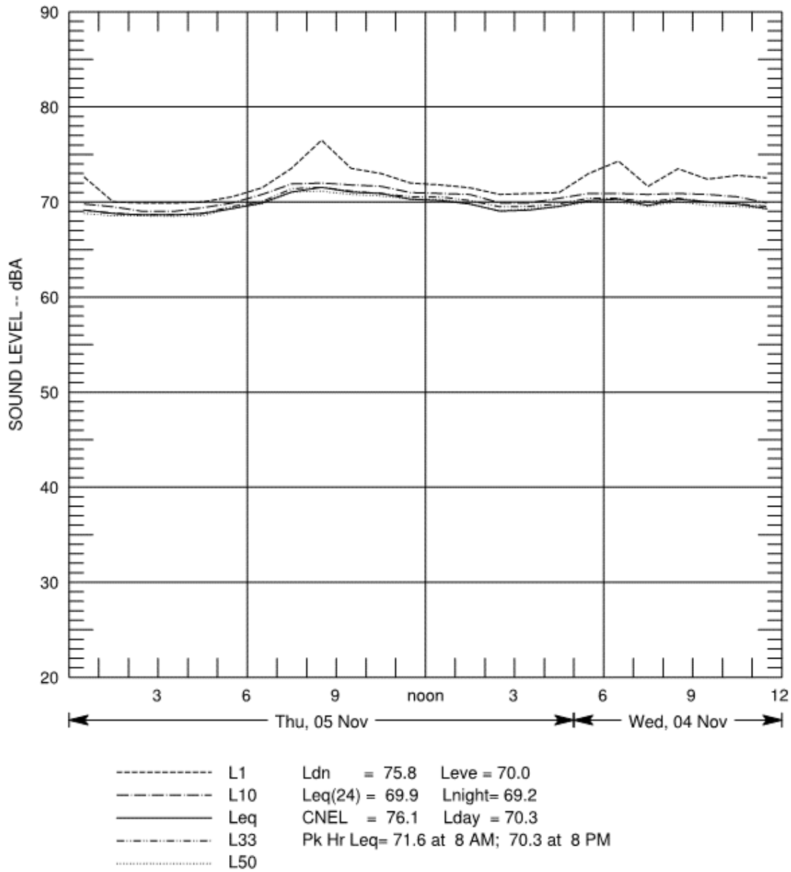
Figure B-42 Hourly Summary of Noise Levels Measured at N14 on November 4 and 5, 2010
