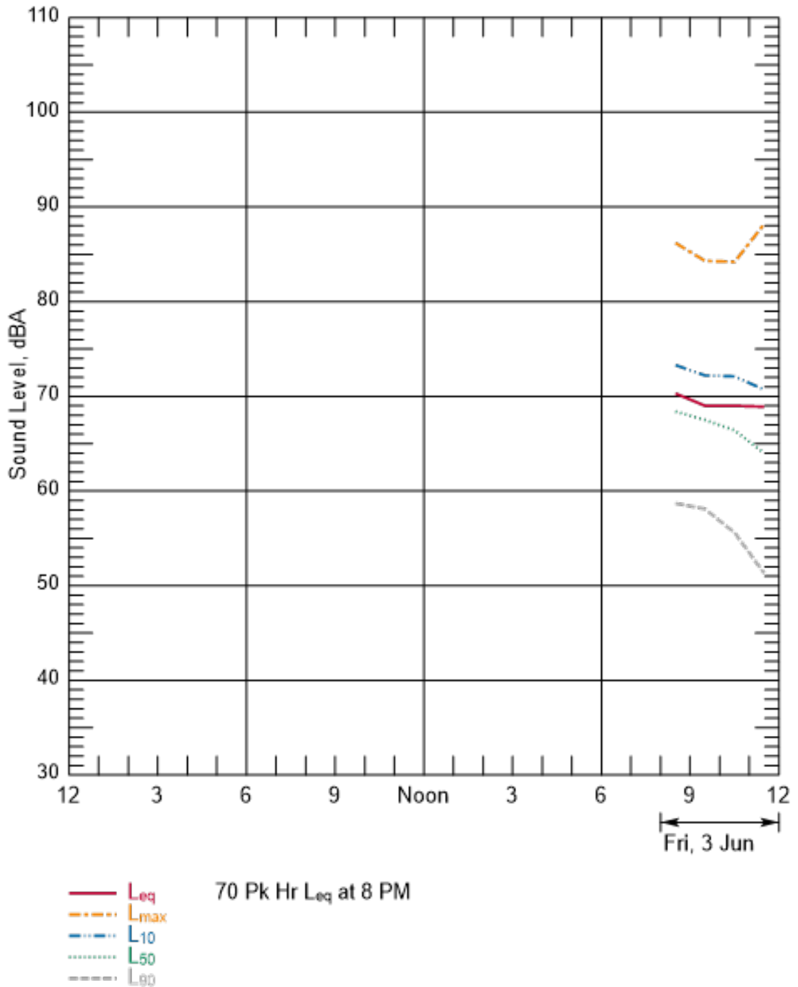
Figure B-175 Hourly Summary of Noise Levels Measured at N61 on June 3, 2016
