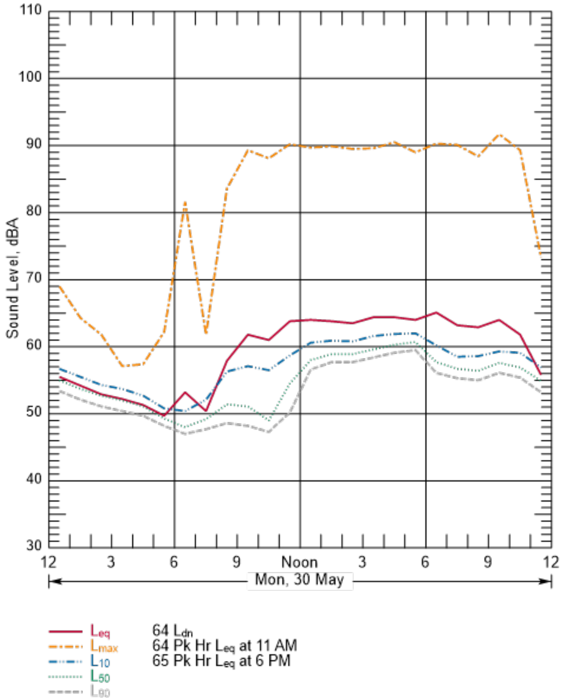
Figure B-17 Hourly Summary of Noise Levels Measured at N06 on May 30, 2016
