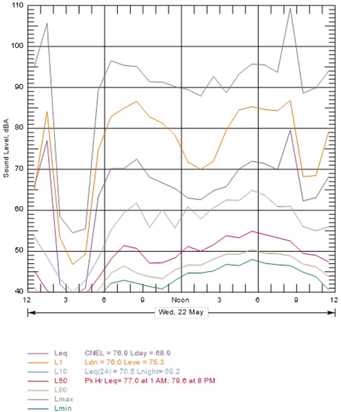
Figure B-103 Hourly Summary of Noise Levels Measured at N35 on May 22, 2013
