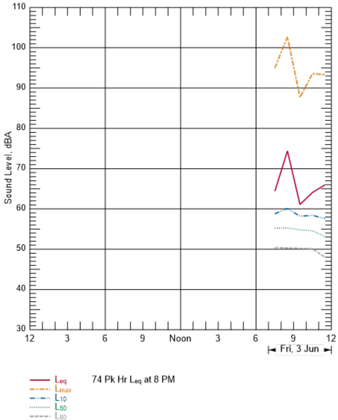
Figure B-158 Hourly Summary of Noise Levels Measured at N55 on June 3, 2016
