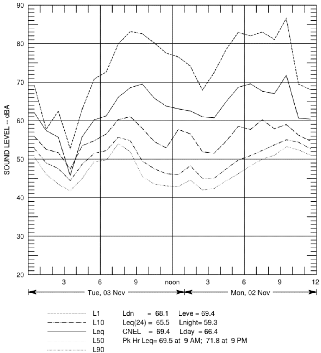
Figure B-107 Hourly Summary of Noise Levels Measured at N36 on November 2 and 3, 2010
