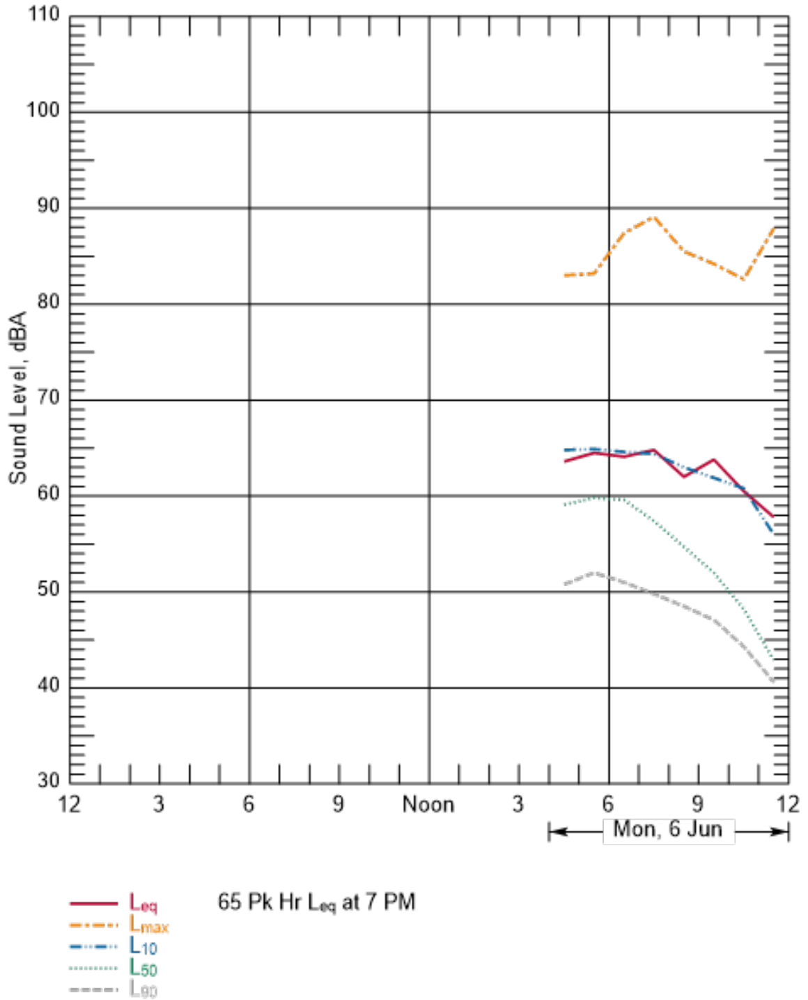
Figure B-199 Hourly Summary of Noise Levels Measured at N70 on June 6, 2016
