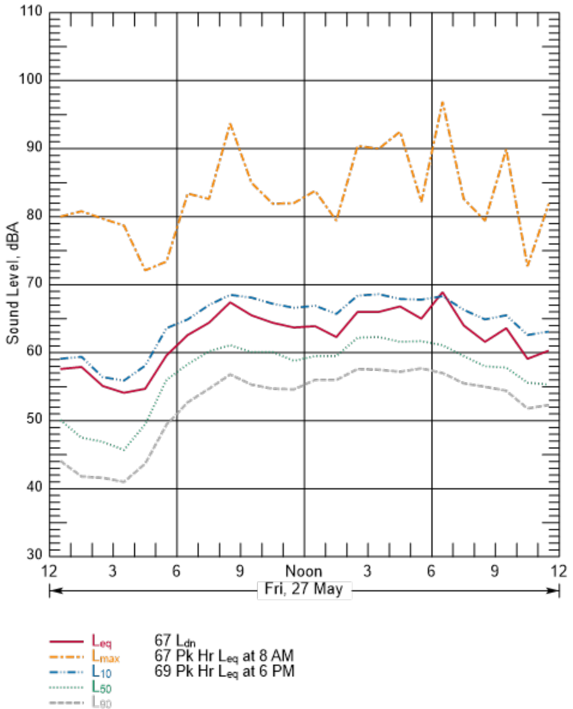
Figure B-27 Hourly Summary of Noise Levels Measured at N10 on May 27, 2016
