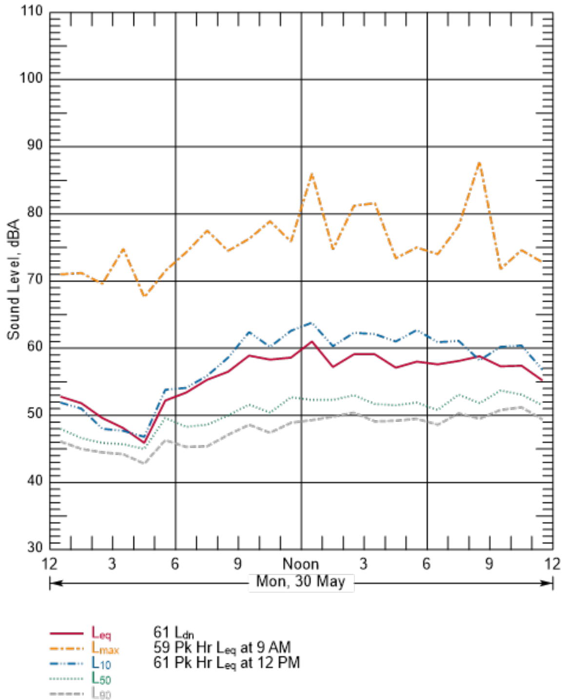
Figure B-32 Hourly Summary of Noise Levels Measured at N11 on May 30, 2016
