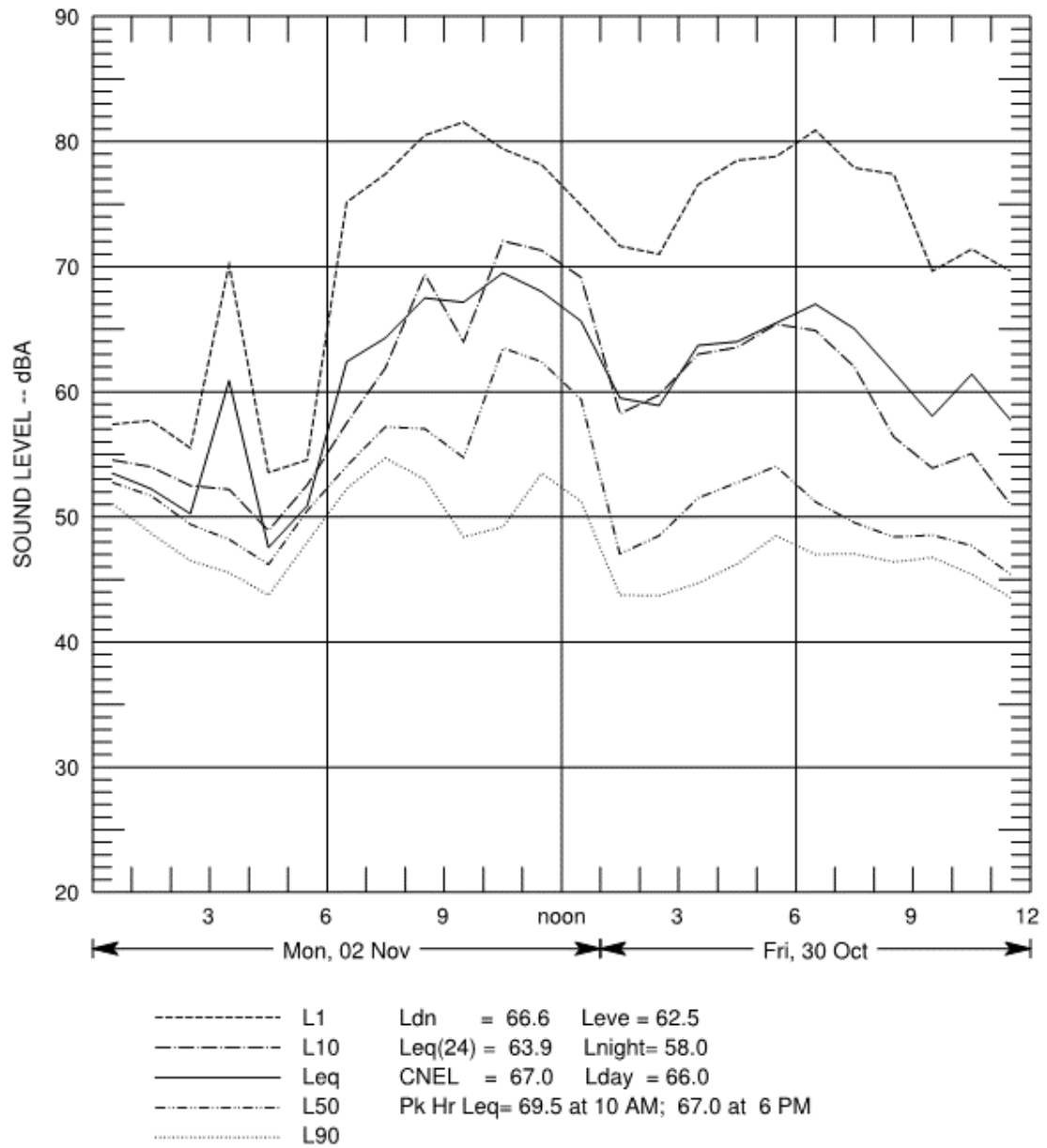
Figure B-133 Hourly Summary of Noise Levels Measured at N45 on October 29 and 30, 2010
