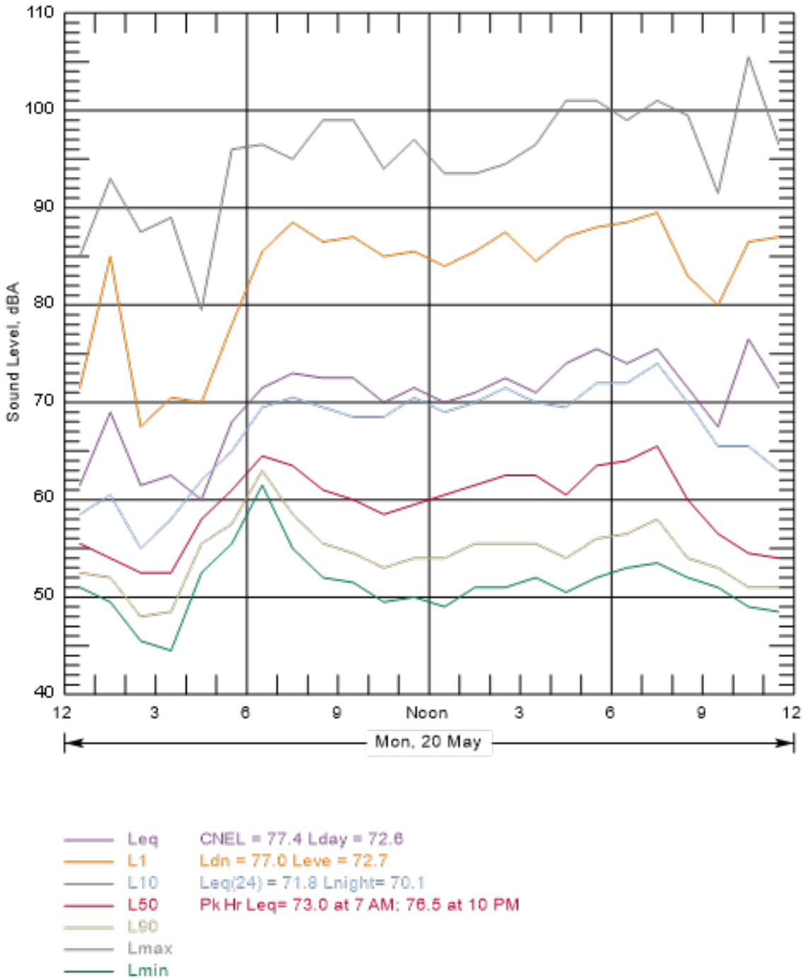
Figure B-50 Hourly Summary of Noise Levels Measured at N18 on May 20, 2013
