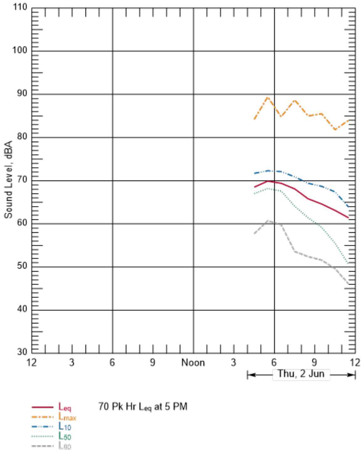
Figure B-123 Hourly Summary of Noise Levels Measured at N42 on June 2, 2016
