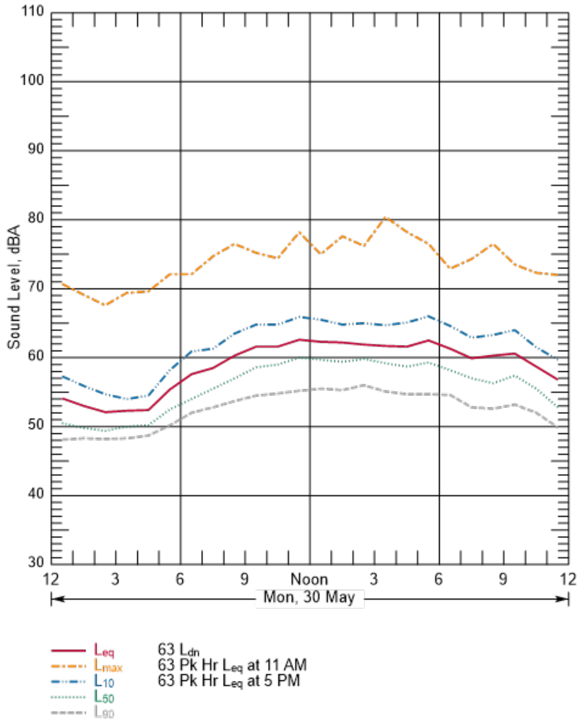
Figure B-36 Hourly Summary of Noise Levels Measured at N12 on May 30, 2016
