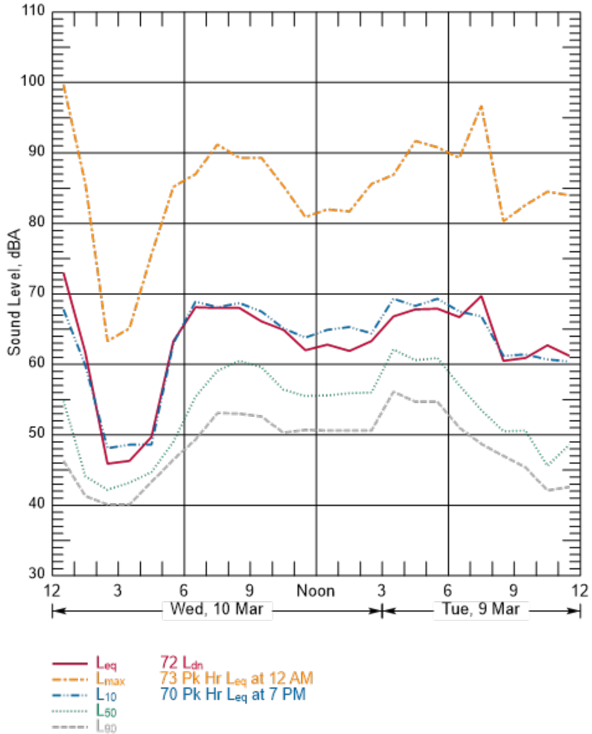
Figure B-152 Hourly Summary of Noise Levels Measured at N52 on March 9 and 10, 2010
