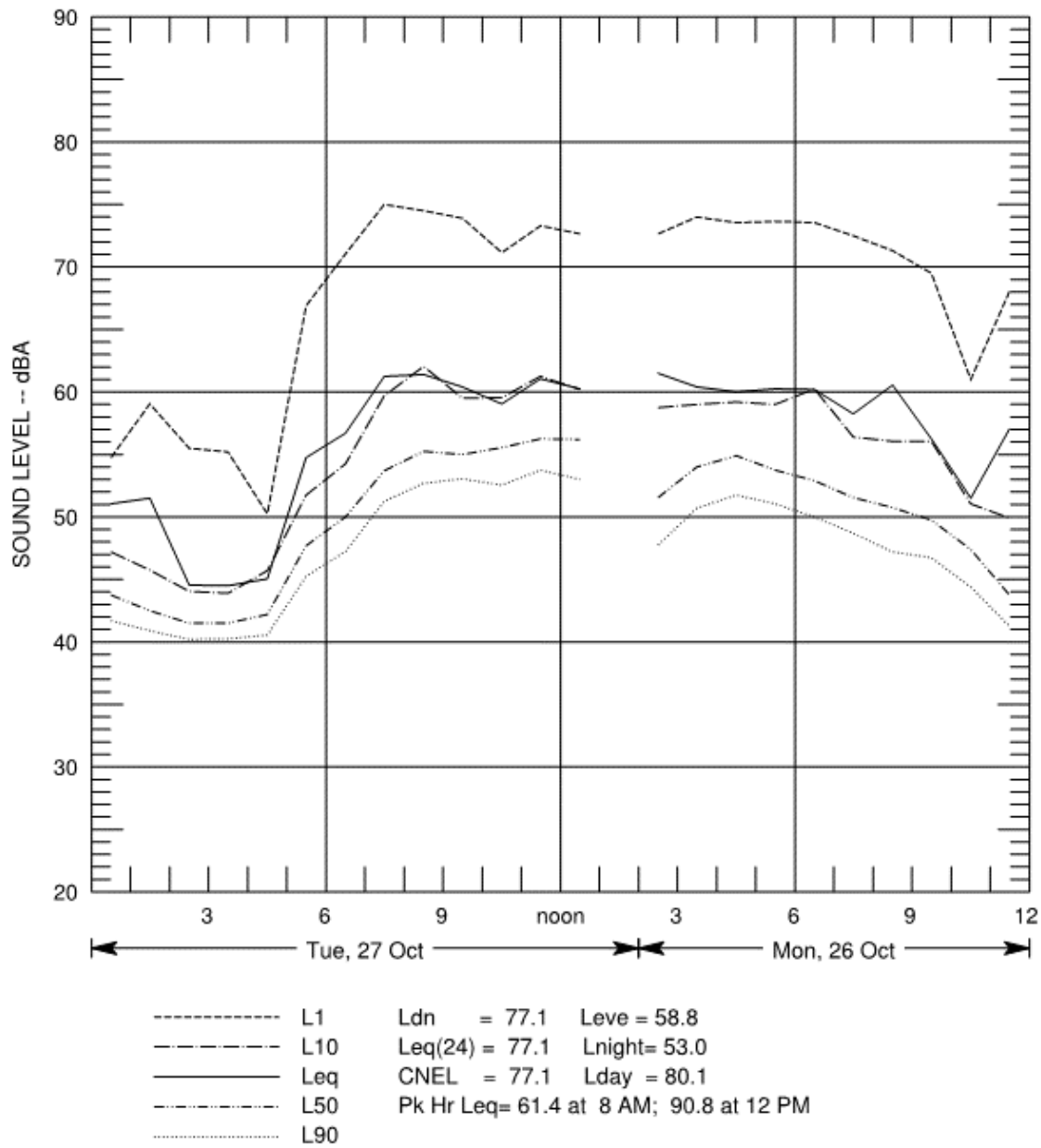
Figure B-166 Hourly Summary of Noise Levels Measured at N58 on October 26 and 27, 2010
