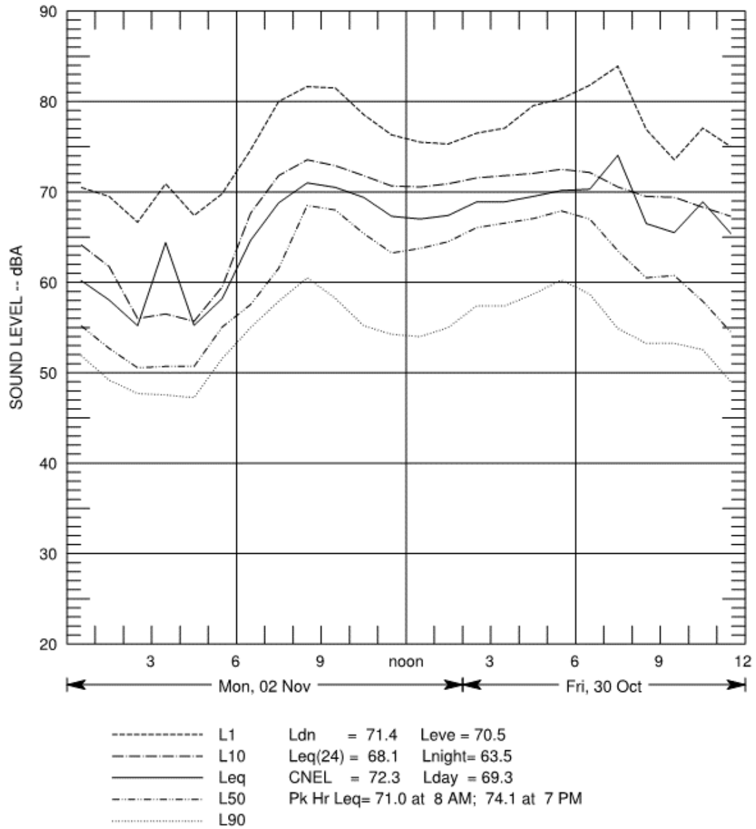
Figure B-91 Hourly Summary of Noise Levels Measured at N32 on October 30 and November 2, 2010
