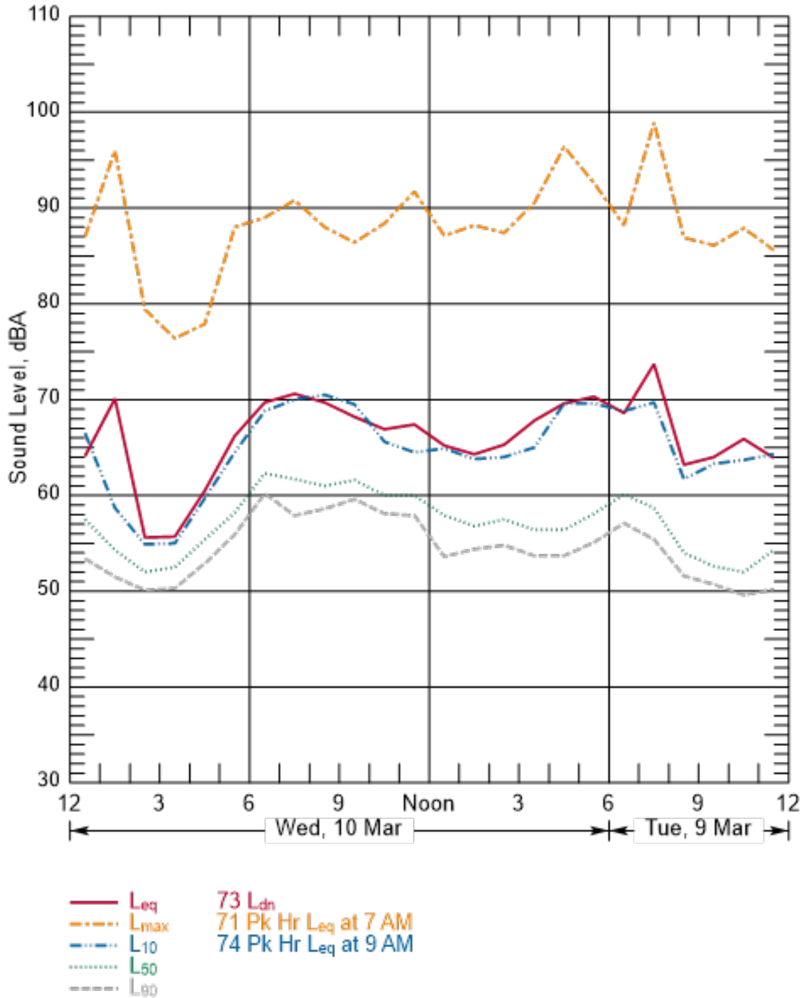
Figure B-77 Hourly Summary of Noise Levels Measured at N27 on March 9 and 10, 2010
