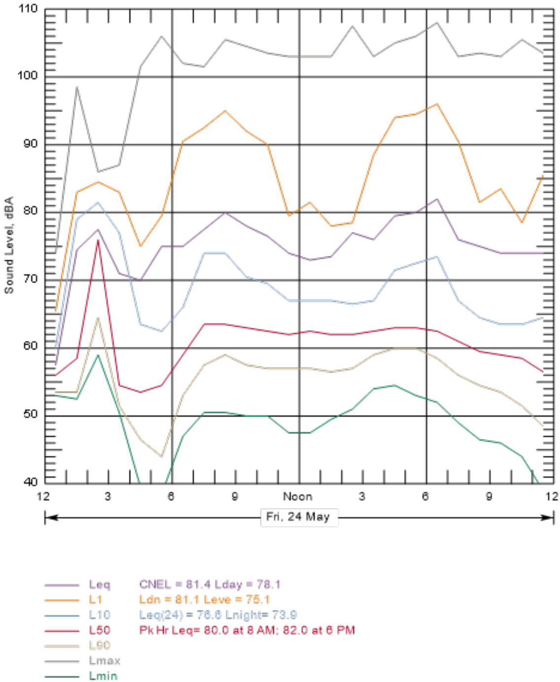
Figure B-184 Hourly Summary of Noise Levels Measured at N63 on May 24, 2013
