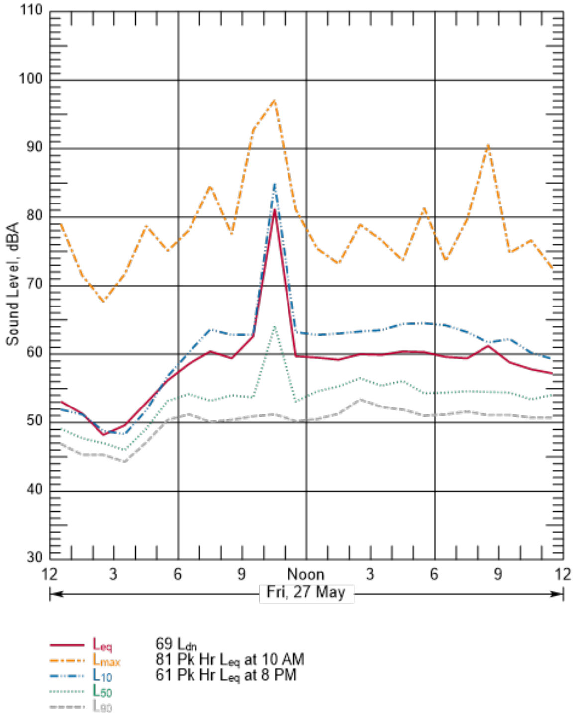
Figure B-31 Hourly Summary of Noise Levels Measured at N11 on May 27, 2016
