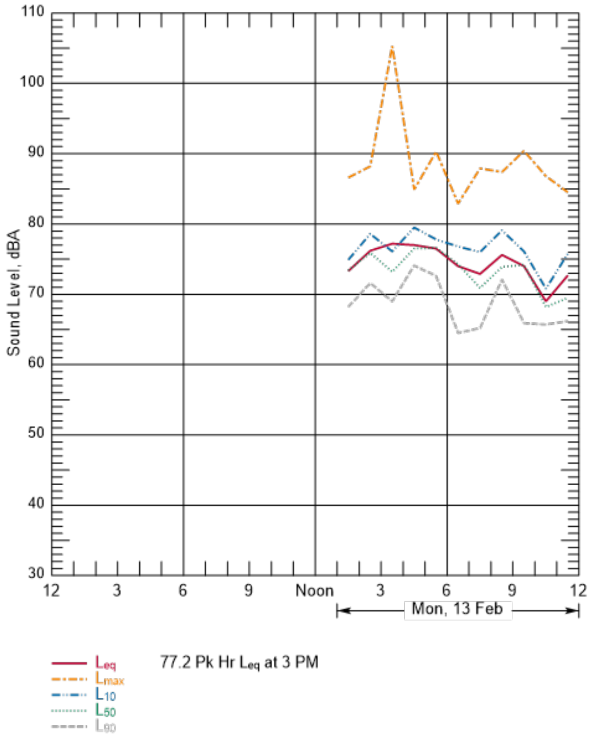
Figure B-1 Hourly Summary of Noise Levels Measured at N01 on February 13, 2017
