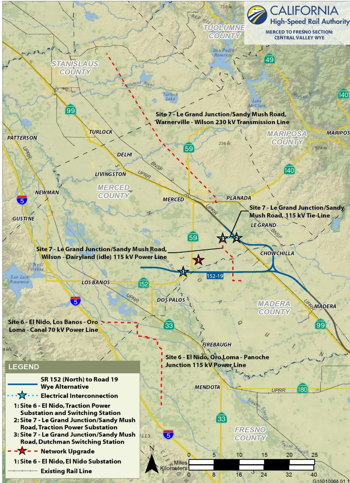
Figure 2-11 SR 152 (North) to Road 19 Wye Alternative Electrical Interconnections and Network Upgrades
