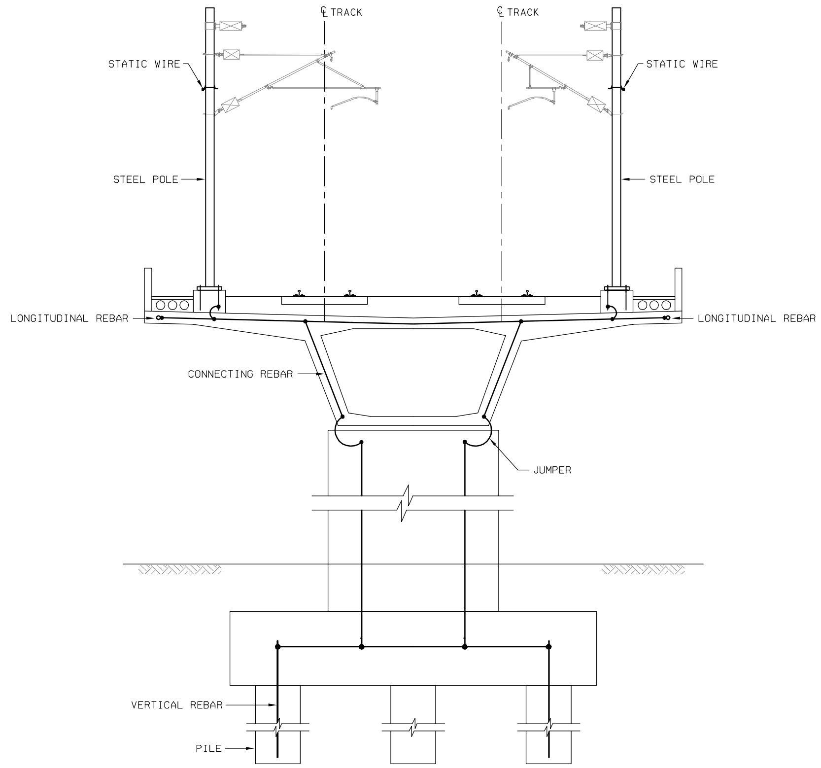
TYPICAL OCS GROUNDING AND BONDING AT VIADUCT STRUCTURE
