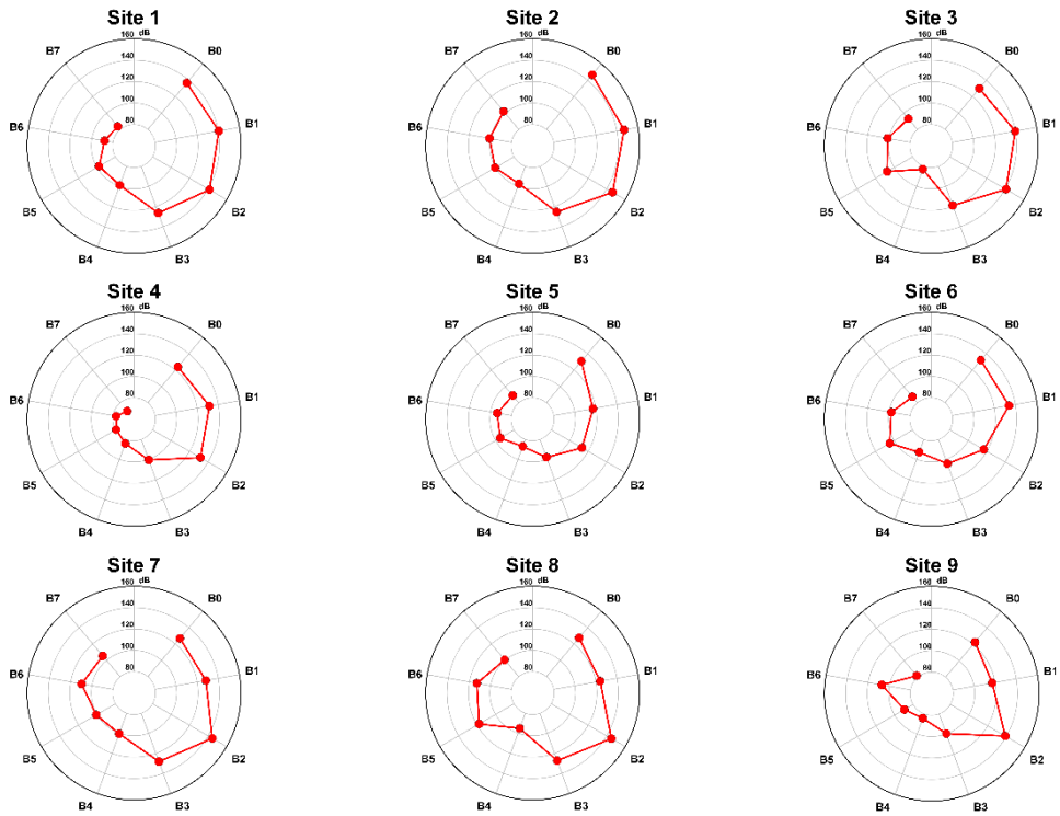
Figure 3.5A-3 Maximum Electric Field Strengths by Site
