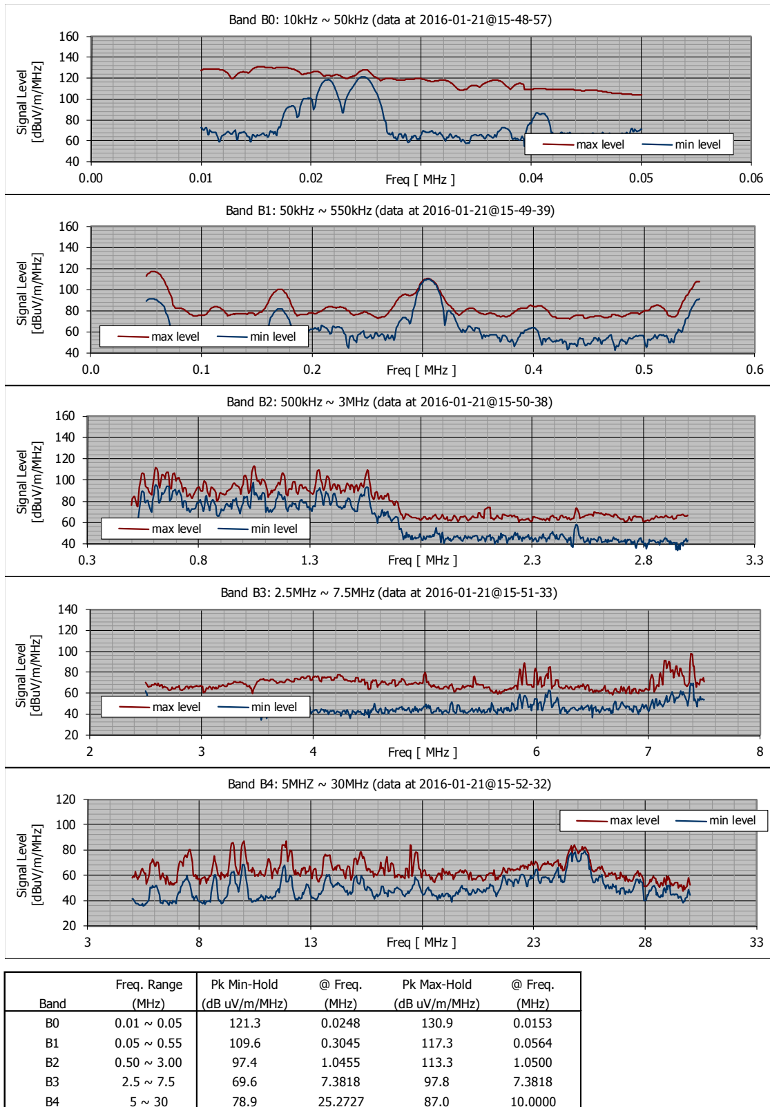
Figure A3.5-5(e) Location 05: RF Data from Non-Directional Vertically-Oriented Monopole Antenna
