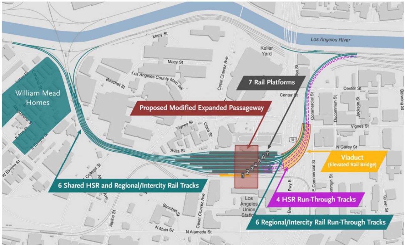
Figure 2: Link US Project Components
