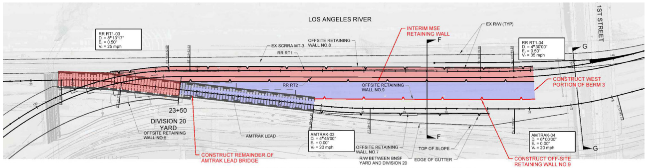
Figure 4: Link US Phase A Project Base Scope with Optional Scope (in Blue) in the Vicinity of the BNSF Yard (Source: Metro Response to PFAL Issues 11/22/2019)
