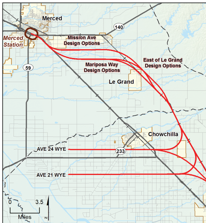
Figure 2-48 Mission Ave and Mariposa Way Design Options in the Merced Project Vicinity
