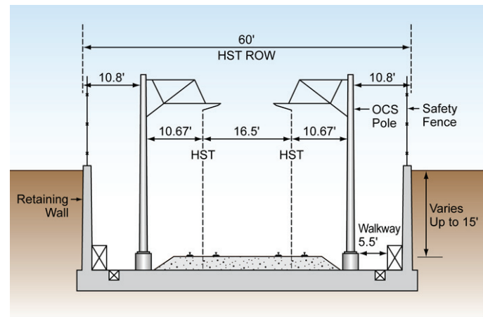
Figure 2-7b Retained Cut Typical Cross Section
