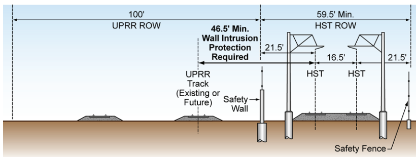
(c) UPRR/SR 99 Centerline-UPRR Right-of-Way Separation 21.5 Feet (Min.) to 48 Feet (Wall Intrusion Protection Required)
