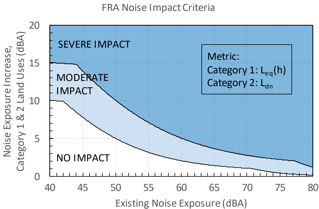
Figure 3.4-5 Allowable Increase in Combined/Cumulative Noise Levels (Land Use Categories 1 & 2)
