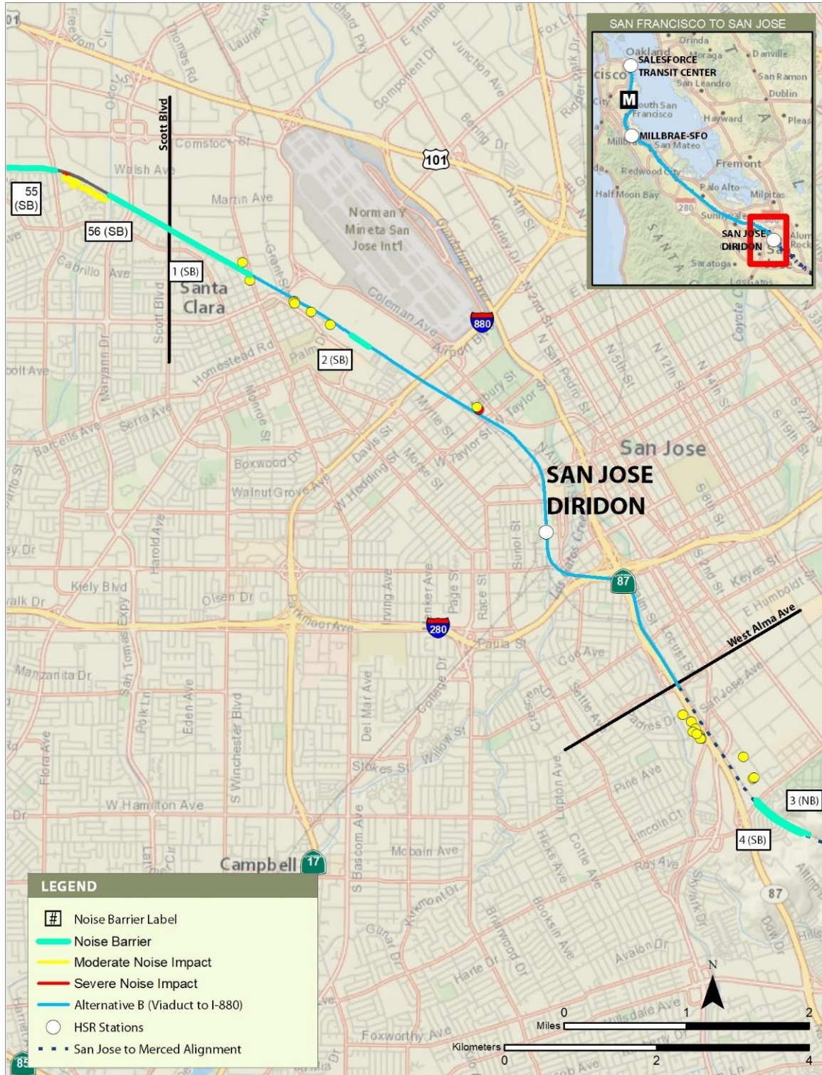
Figure 3.4-41 Noise Barriers and Residual Noise Impacts without Quiet Zones—Alternative B (Viaduct to I-880) (San Jose Diridon Station Approach Subsection)
