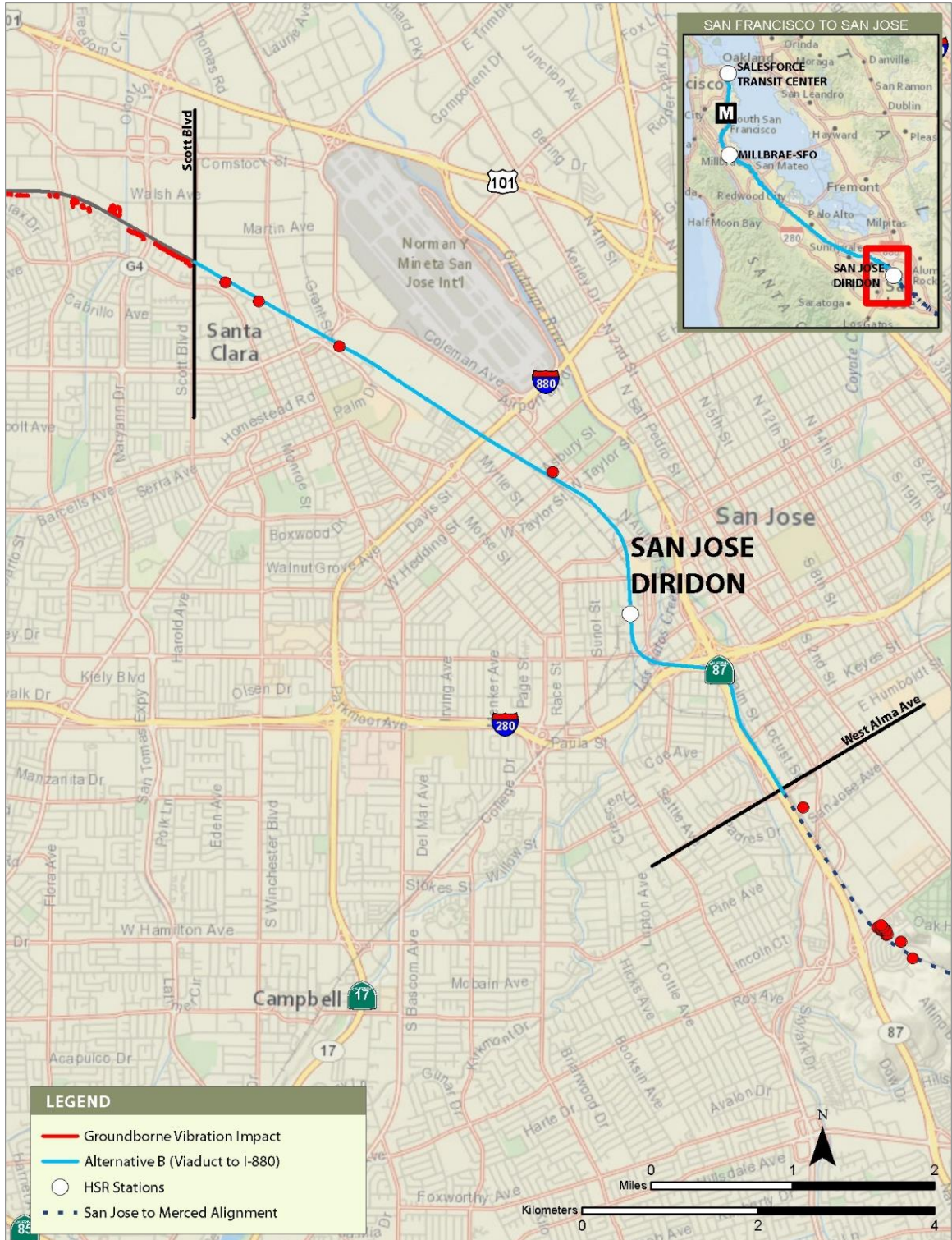
Figure 3.4-29 2040 Plus Project Vibration Impacts—Alternative B (Viaduct to I-880) (San Jose Diridon Station Approach Subsection)
