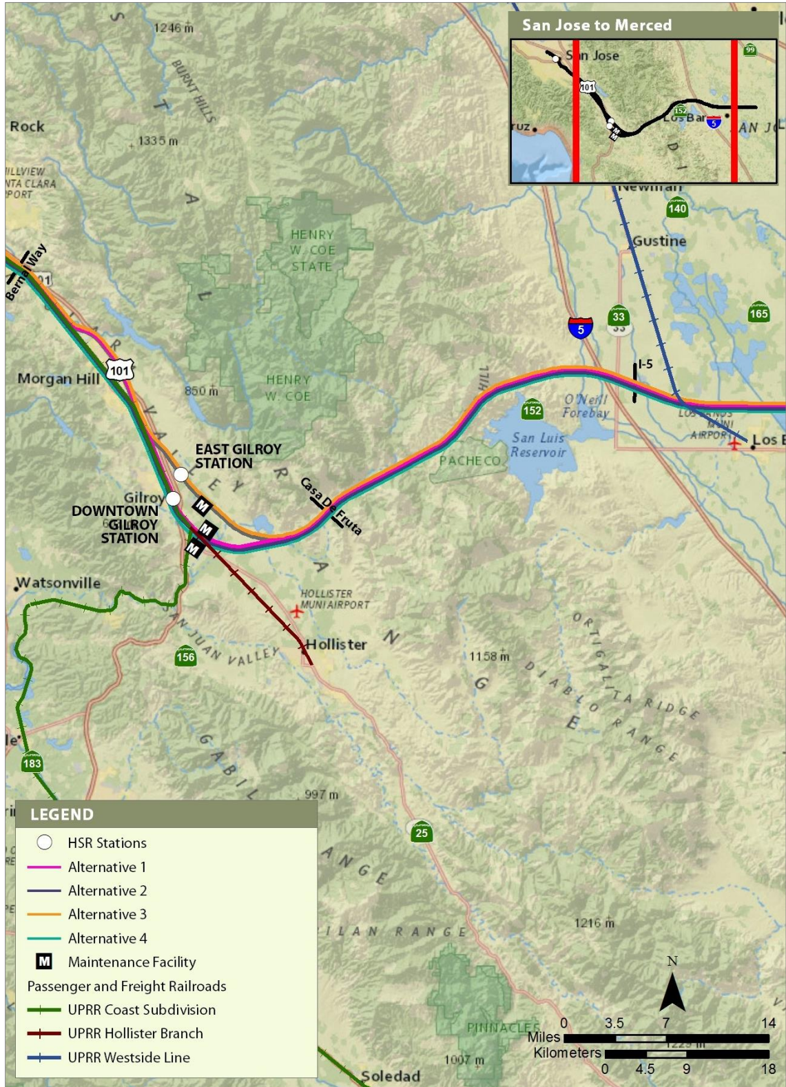
Figure 3.2-10 Railroad Control Points and Subdivisions in the RSA (Morgan Hill and Gilroy and Pacheco Pass Subsections)
