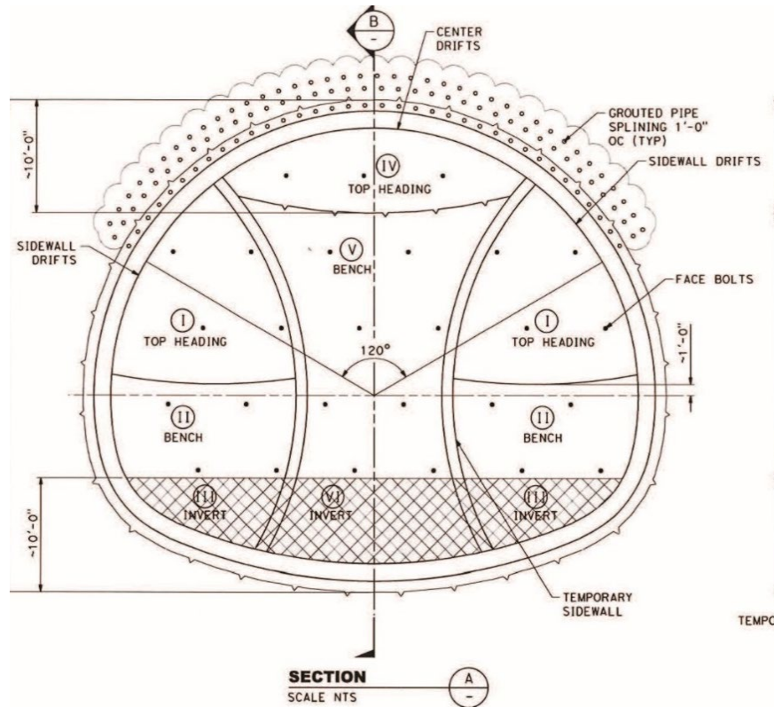
Figure 2-45 Sequential Excavation Method Construction Sequencing
