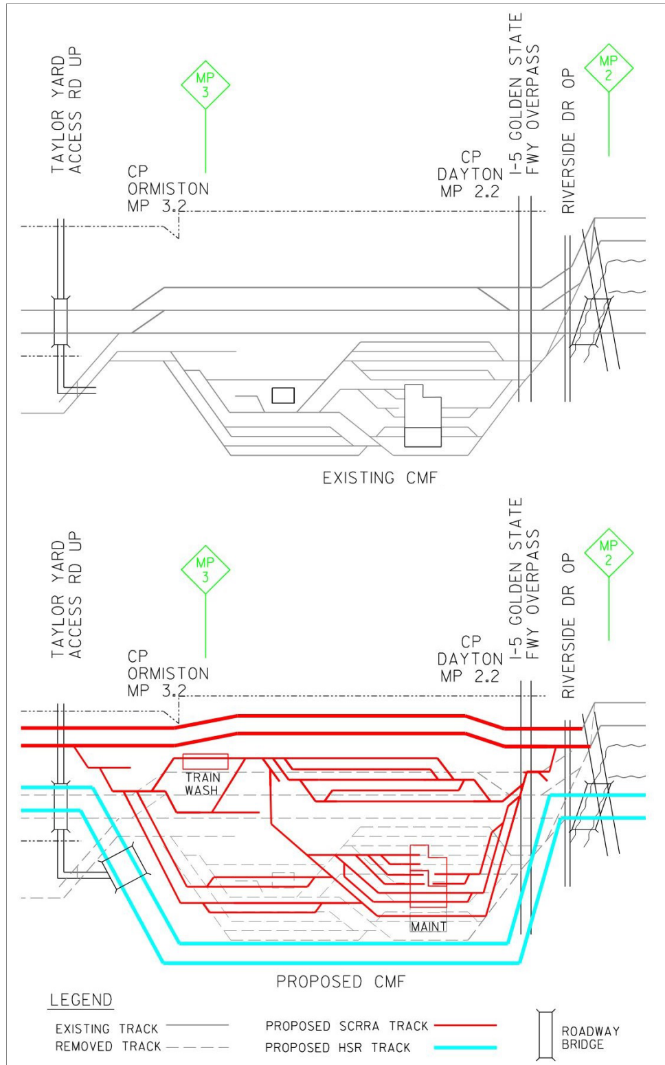
Figure 2-27 Diagram of Existing and Proposed Metrolink Central Maintenance Facility
