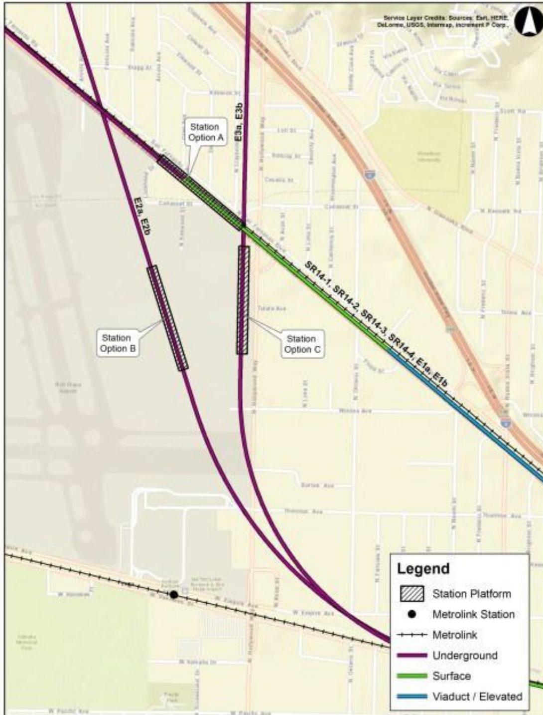
Figure 2-19 Burbank Airport Station Options Evaluated in Palmdale to Burbank 2015 Supplemental Alternatives Analysis
