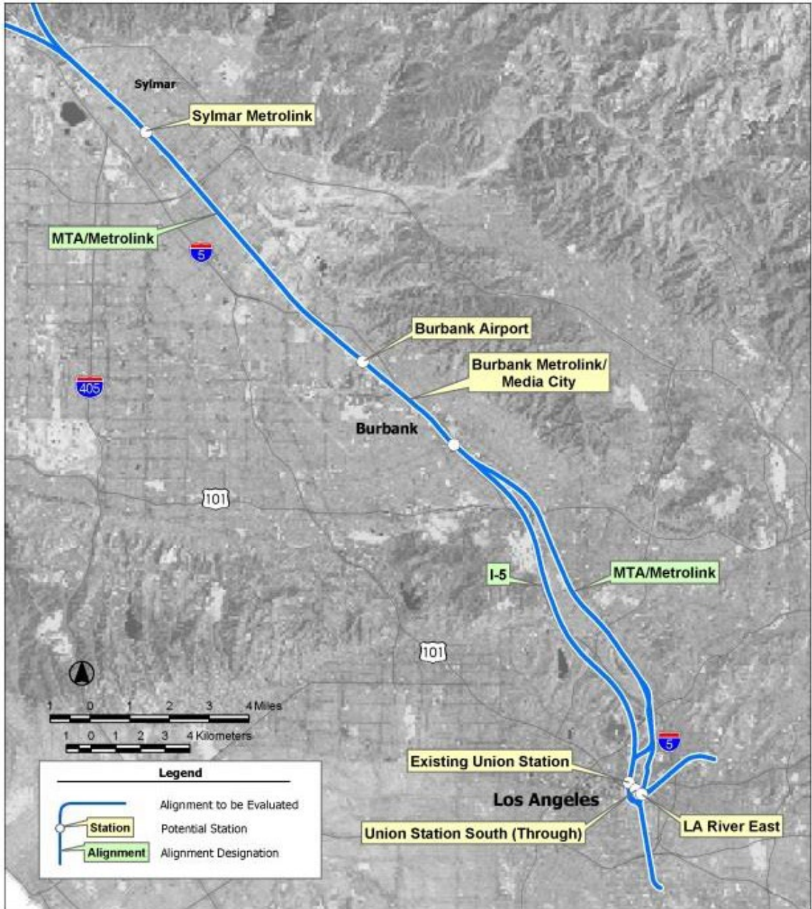
Figure 2-17 Los Angeles Basin Alignment and Station Options Carried forward from 2005 Program EIR/EIS
