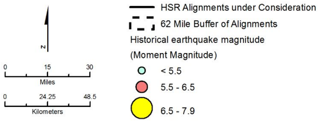
Figure 3.9-13 Historic Earthquakes and Magnitudes within 62 Miles of the Project Vicinity
