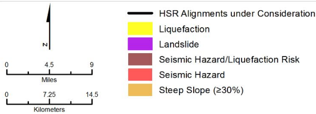
Figure 3.9-9 Landslides, Liquefaction, Seismic Hazards, and Steep Slopes
